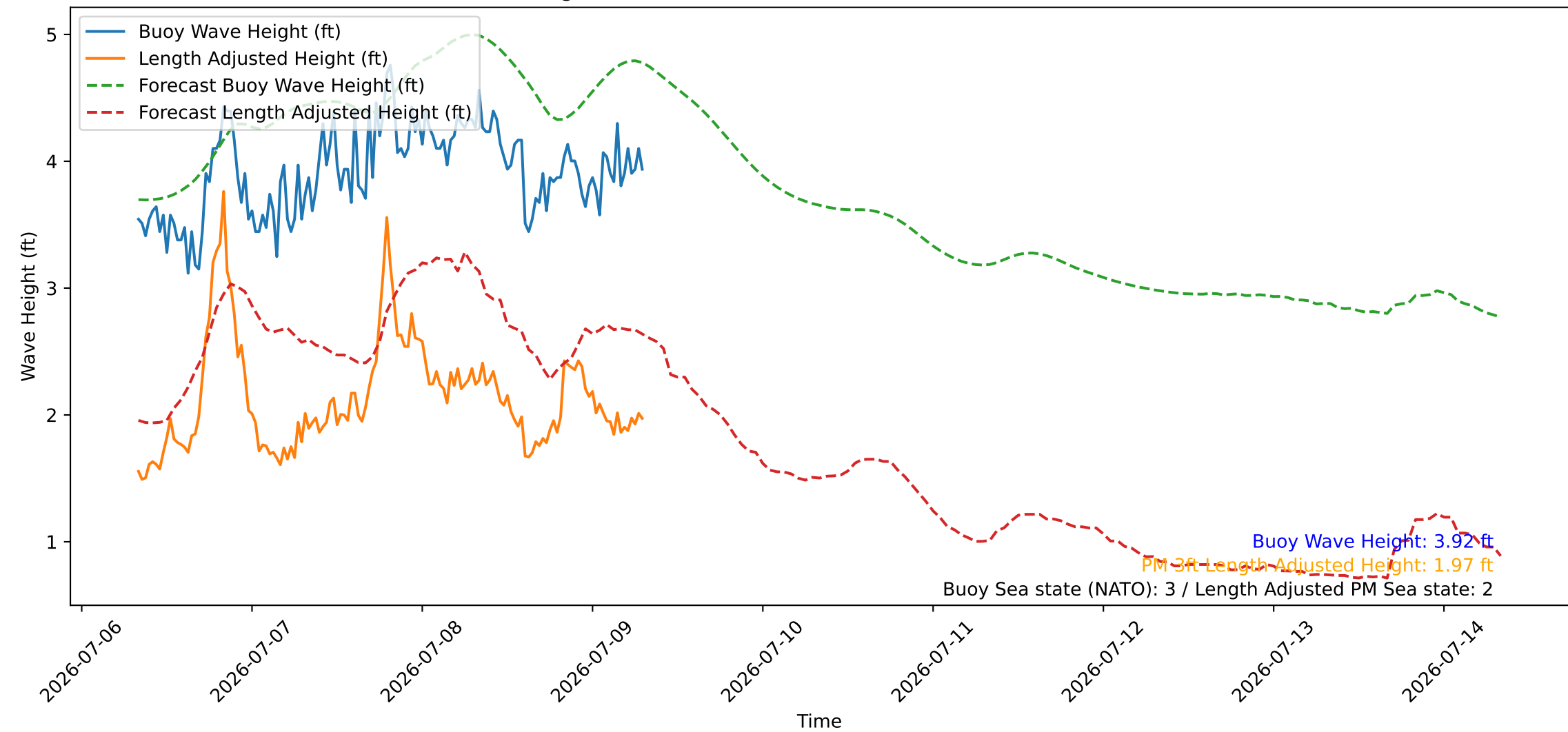
Wave Heights over Time for Green Beach at 2026-07-09 08:01:09
