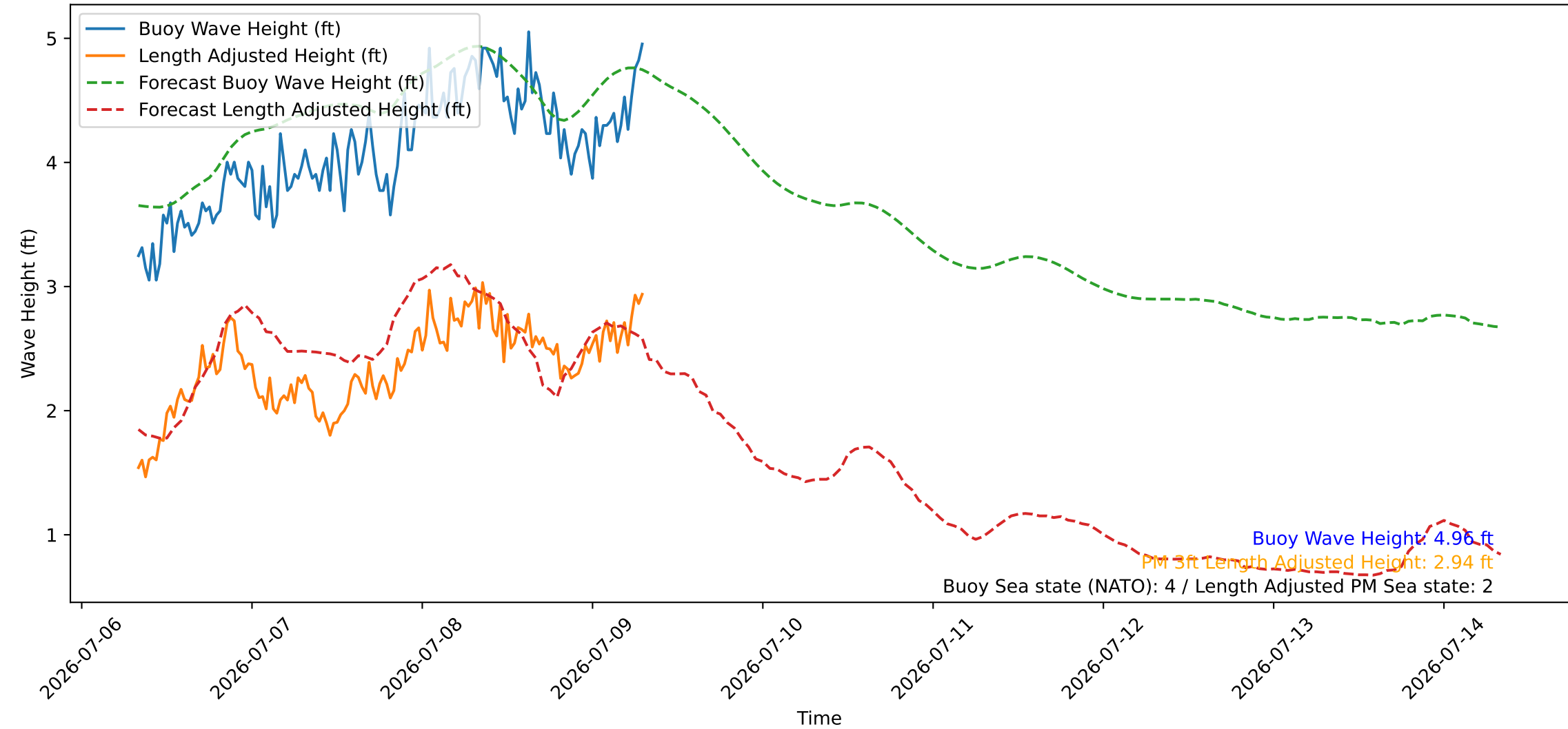
Wave Heights over Time for Oceanside Harbor at 2026-07-09 08:00:27
