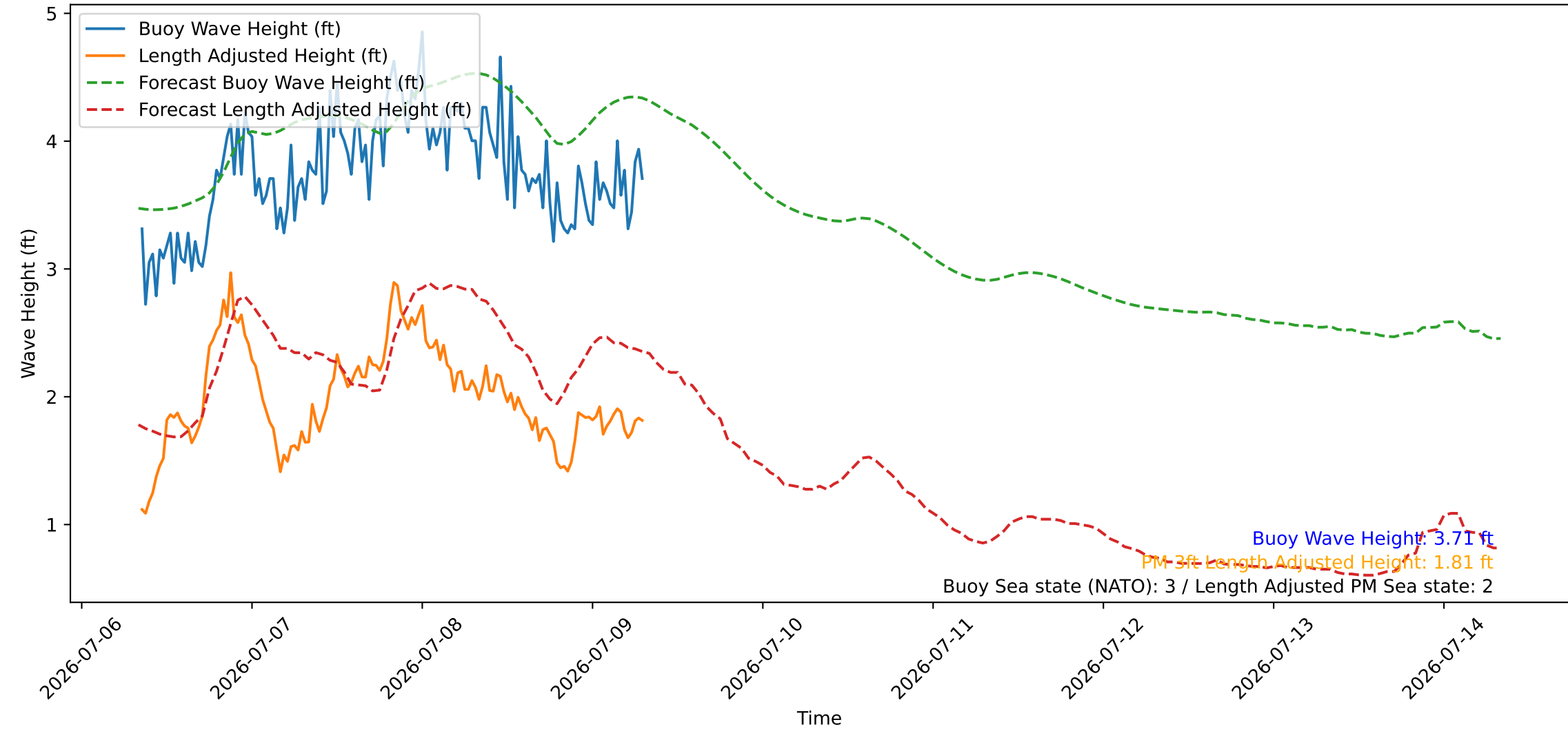
Wave Heights over Time for Red Beach at 2026-07-09 08:00:46
