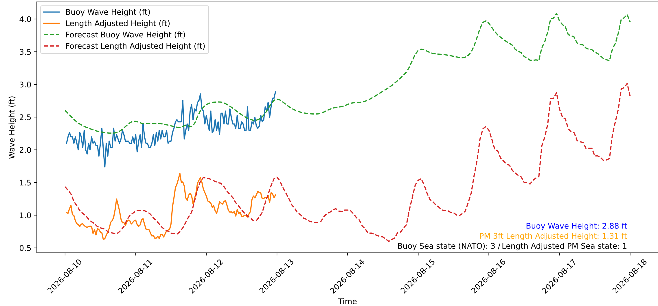
Wave Heights over Time for Red Beach at 2026-08-13 00:20:47
