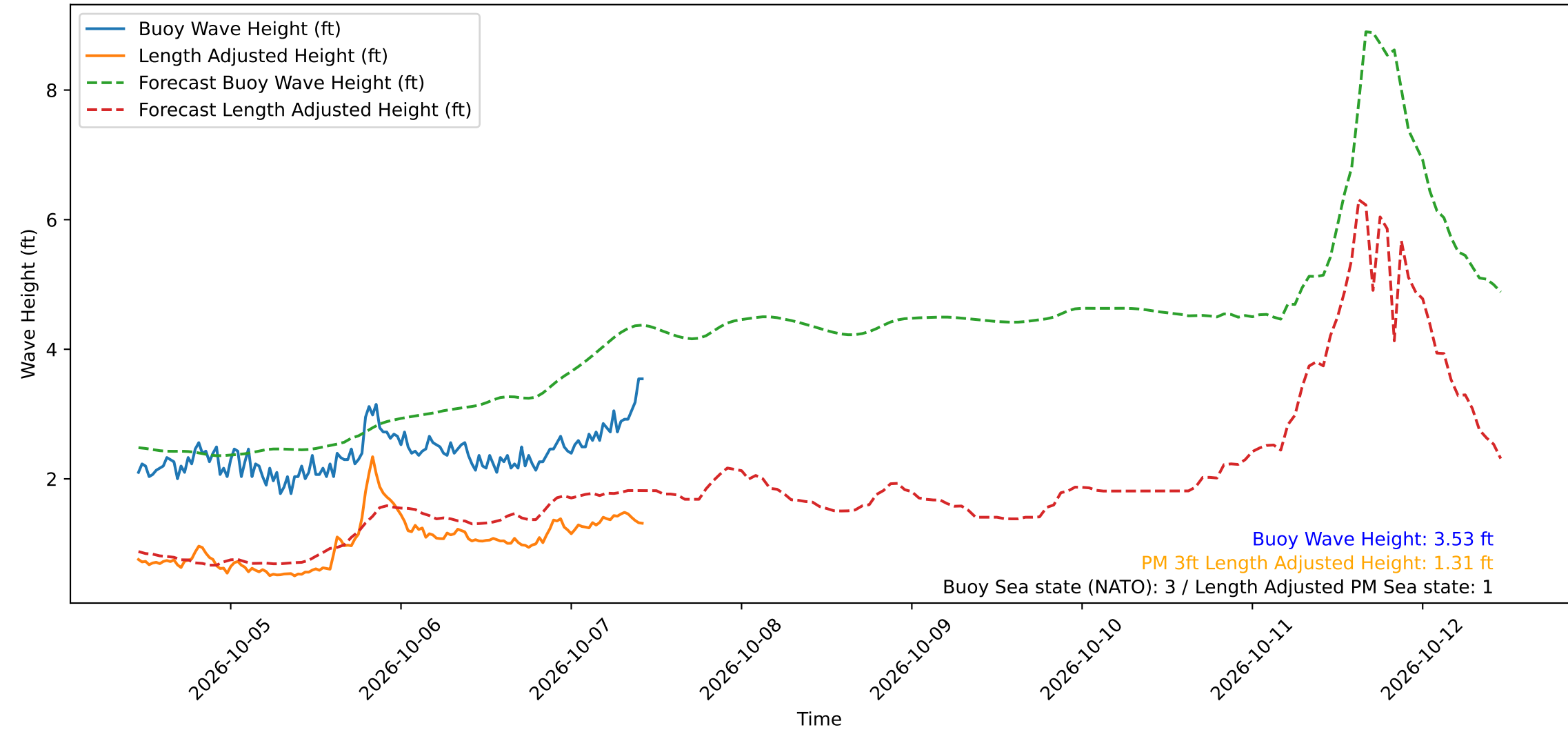
Wave Heights over Time for Green Beach at 2026-10-07 10:41:13
