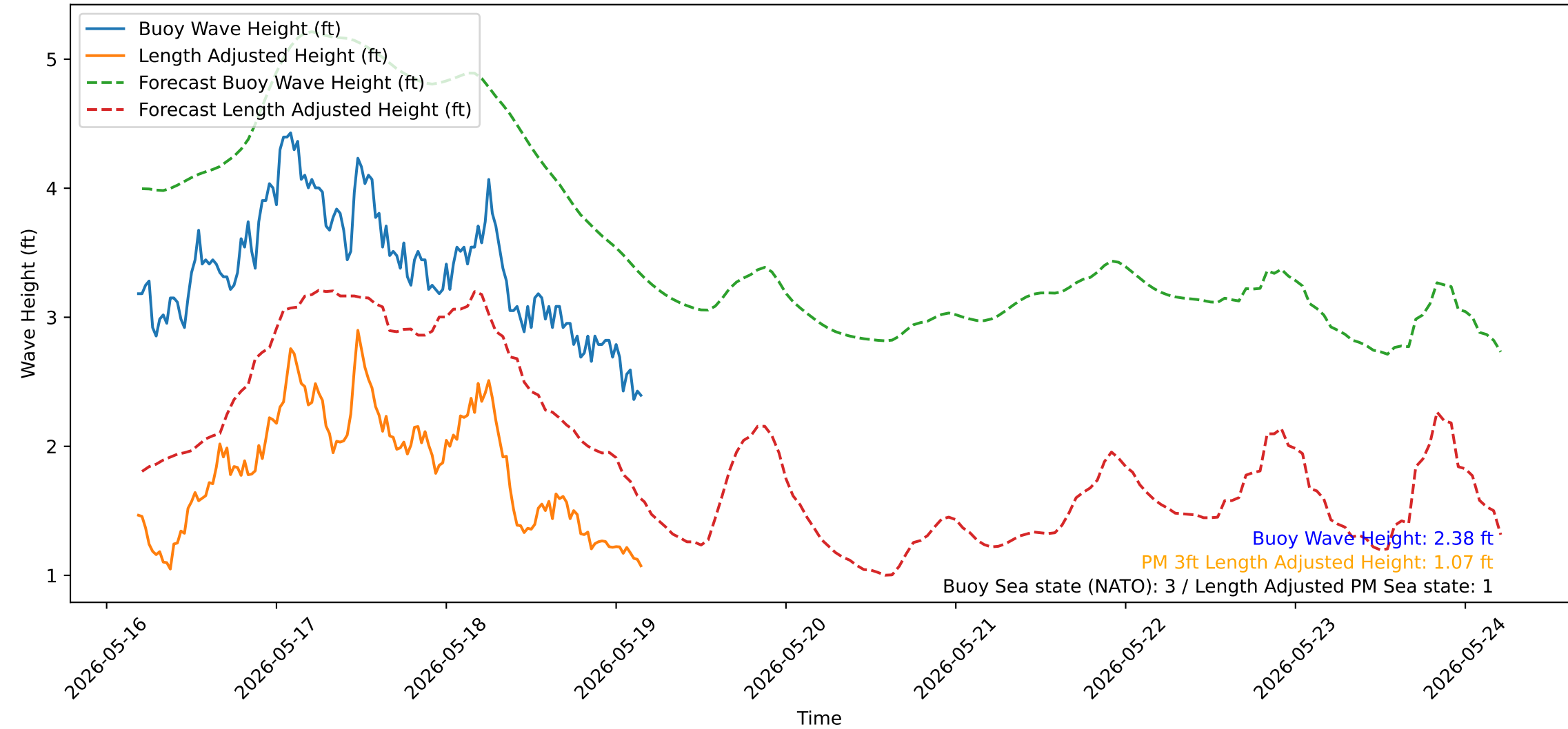
Wave Heights over Time for Green Beach at 2026-05-19 04:31:13
