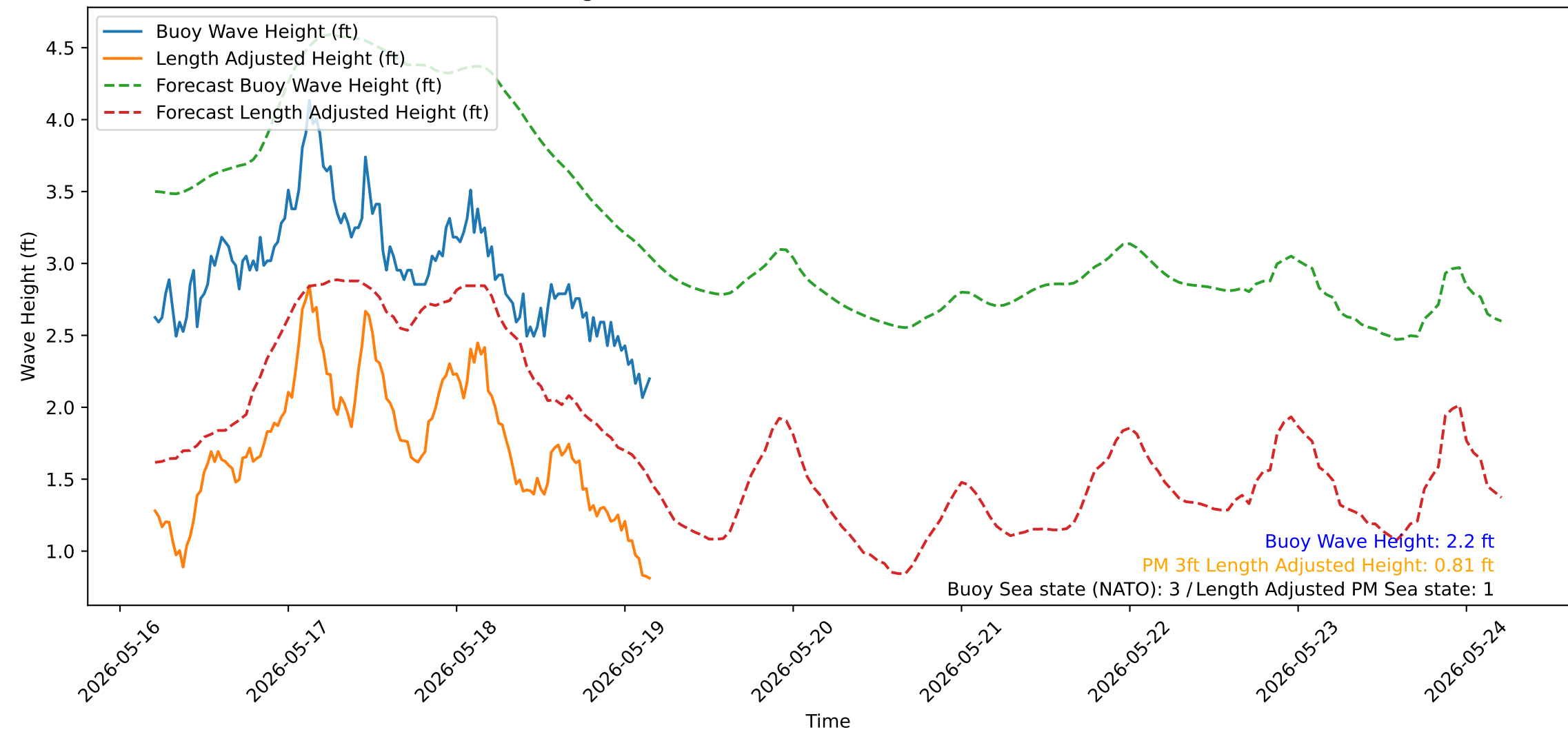
Wave Heights over Time for Red Beach at 2026-05-19 04:30:51
