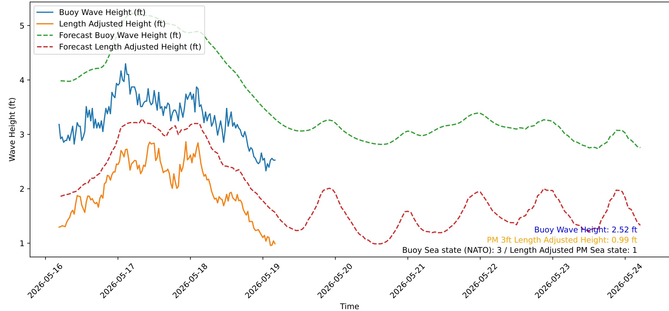
Wave Heights over Time for Oceanside Harbor at 2026-05-19 04:30:31
