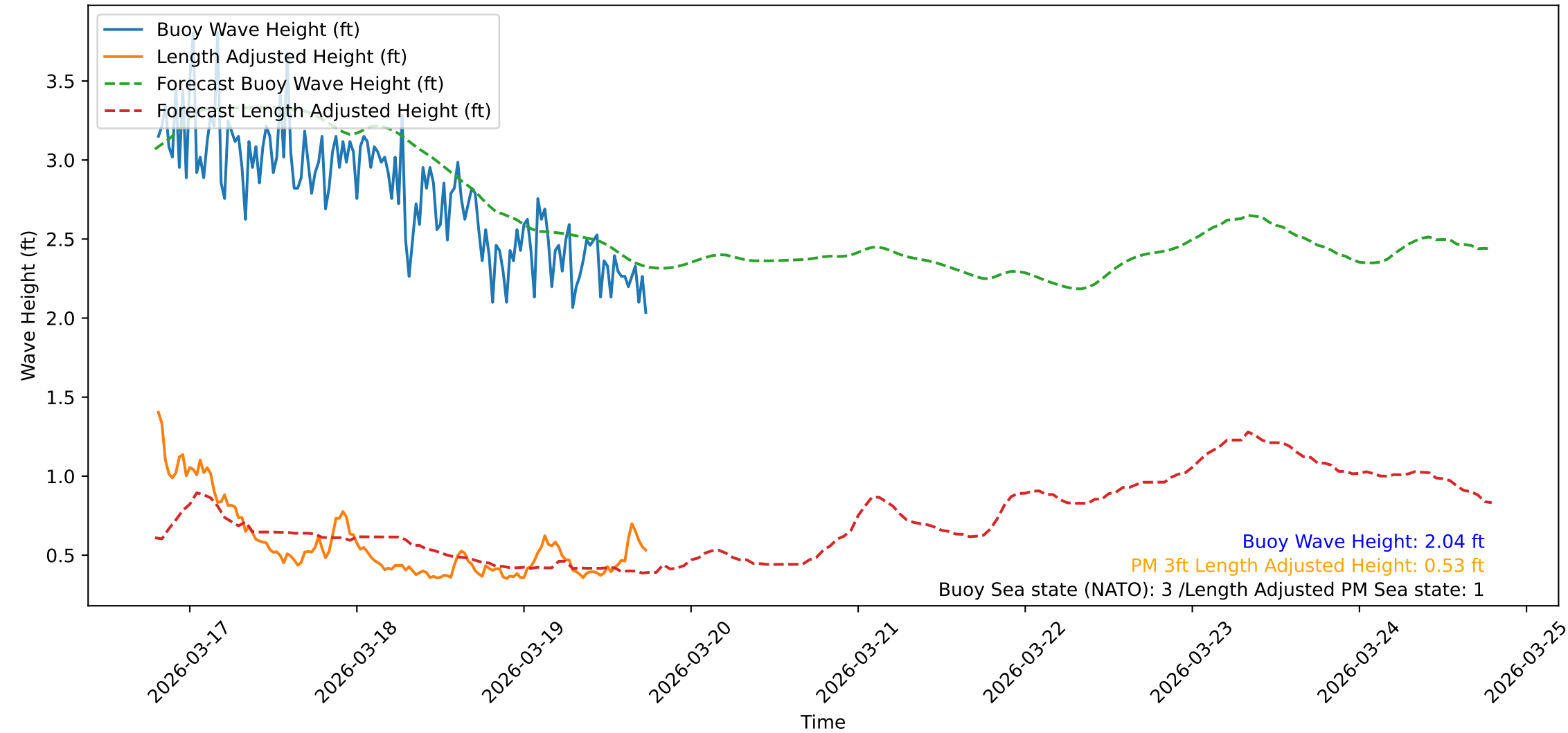
Wave Heights over Time for Red Beach at 2026-03-19 19:00:50
