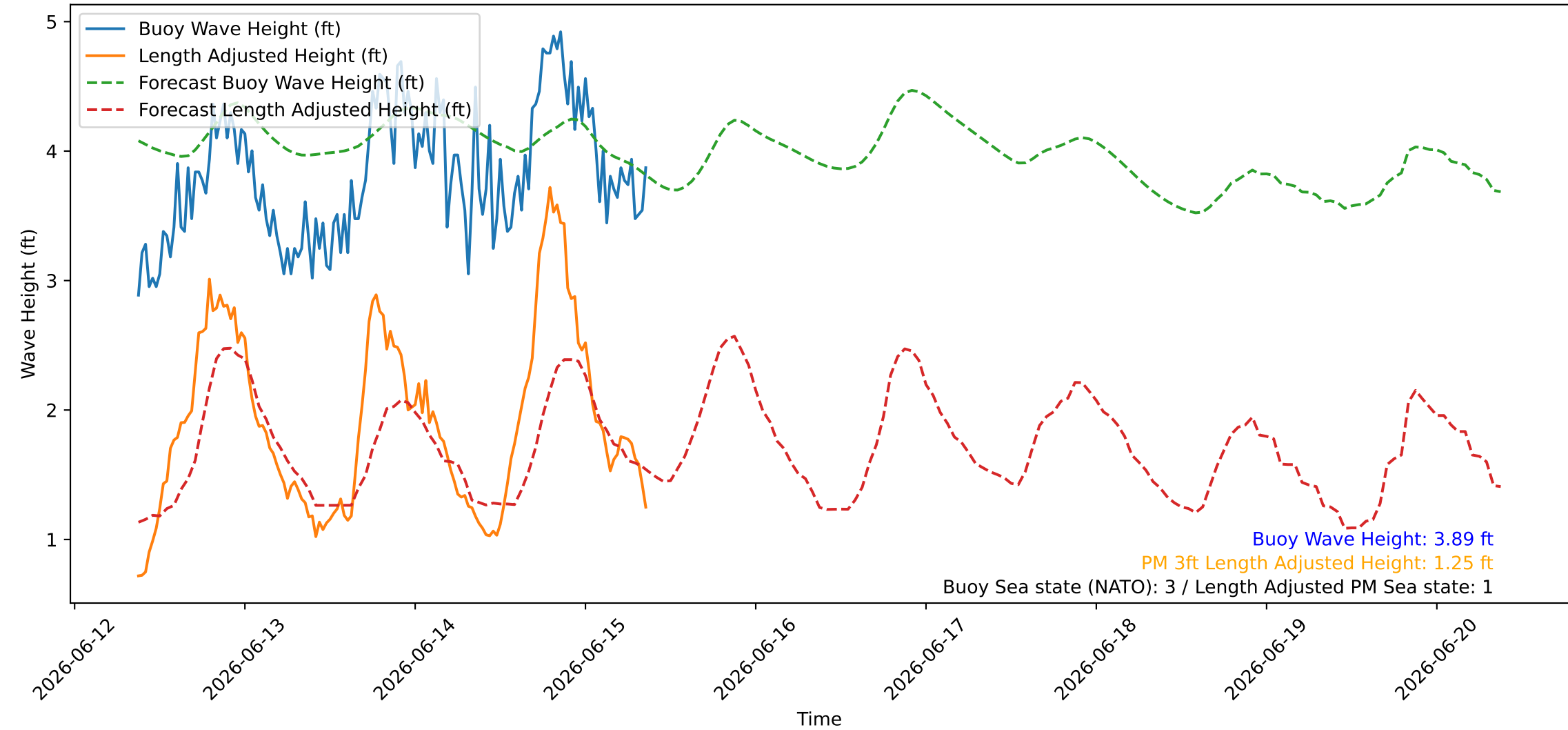
Wave Heights over Time for Green Beach at 2026-06-15 09:11:09
