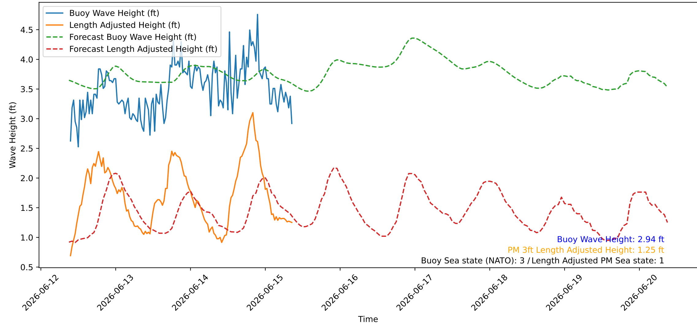
Wave Heights over Time for Red Beach at 2026-06-15 09:10:46
