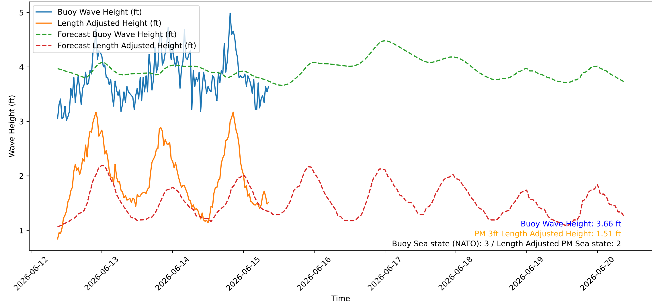
Wave Heights over Time for Oceanside Harbor at 2026-06-15 09:10:26
