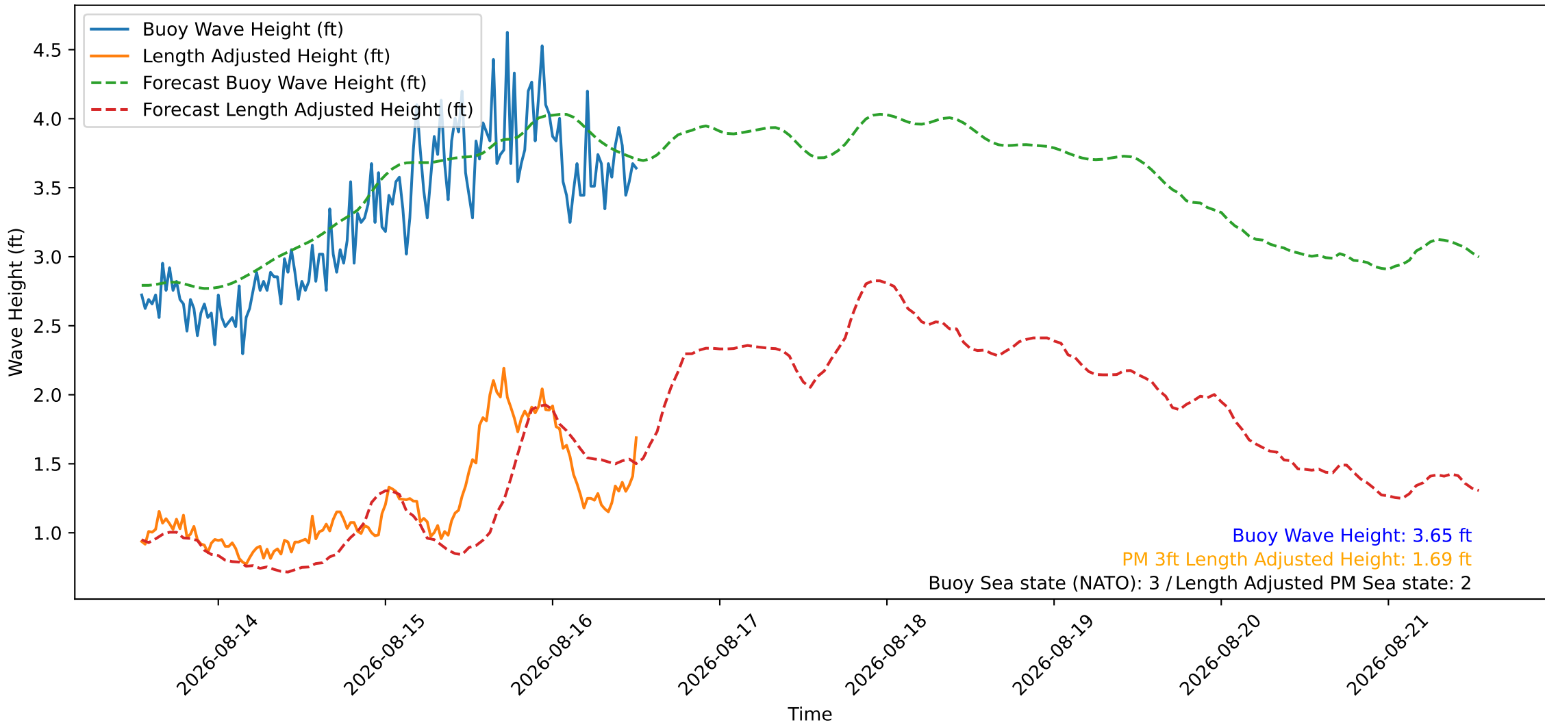
Wave Heights over Time for Oceanside Harbor at 2026-08-16 13:00:26
