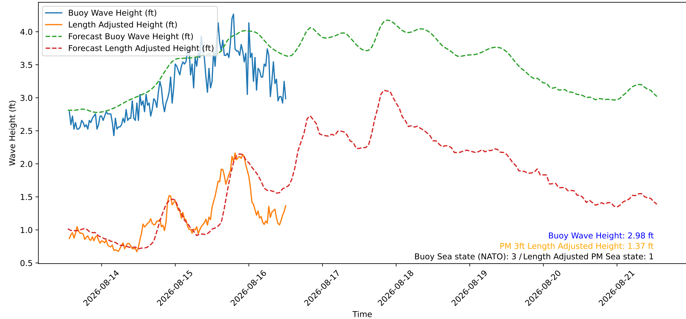
Wave Heights over Time for Green Beach at 2026-08-16 13:01:07
