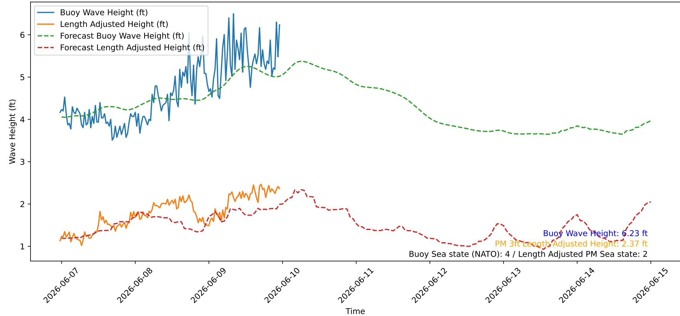
Wave Heights over Time for Oceanside Harbor at 2026-06-09 23:40:27
