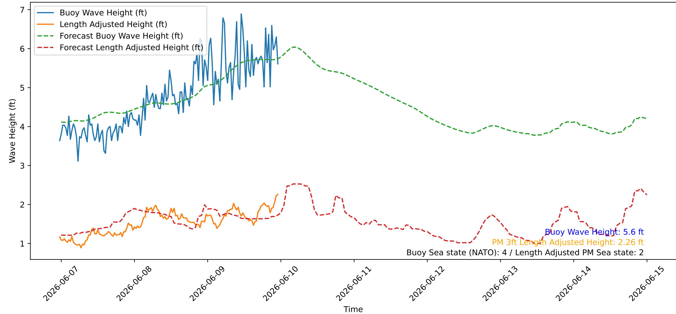
Wave Heights over Time for Green Beach at 2026-06-09 23:41:10
