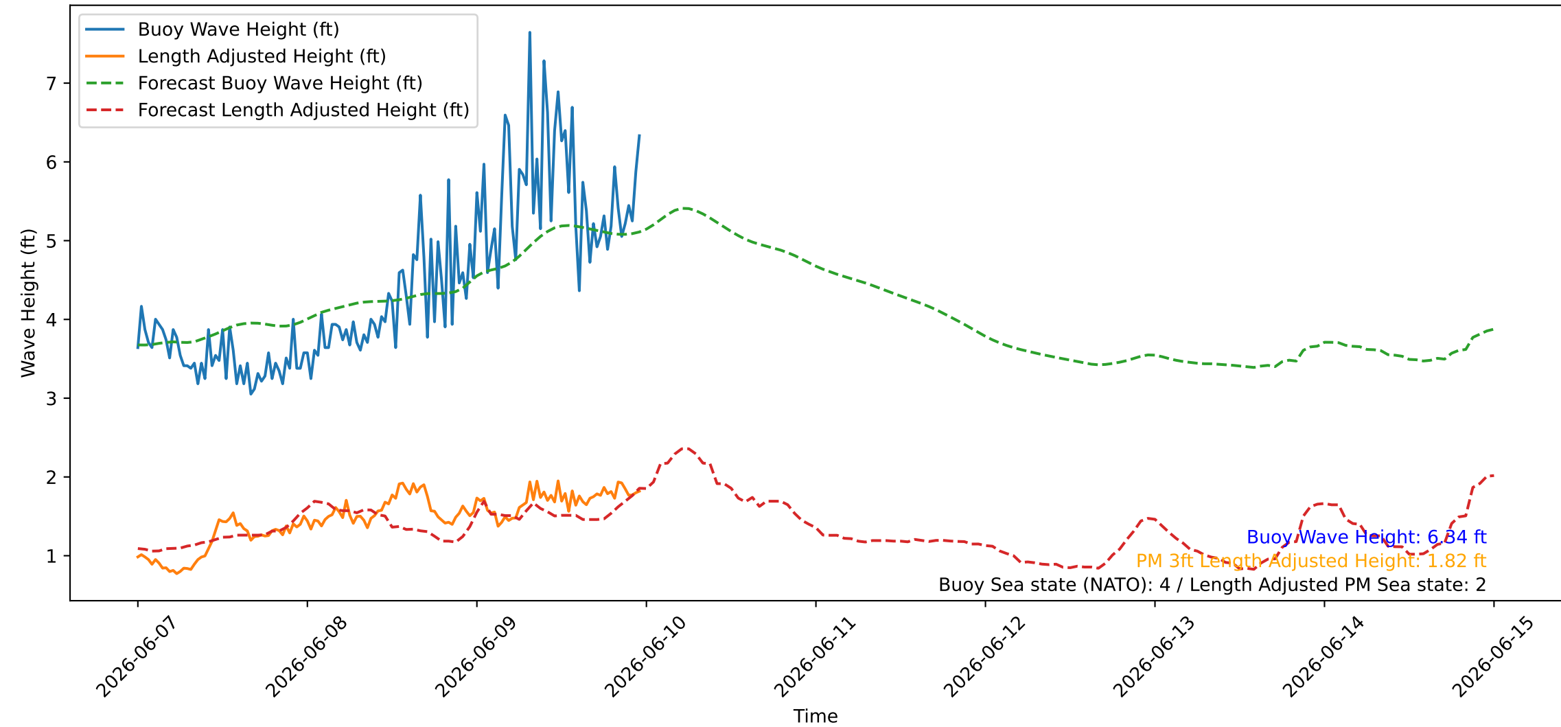
Wave Heights over Time for Red Beach at 2026-06-09 23:40:47
