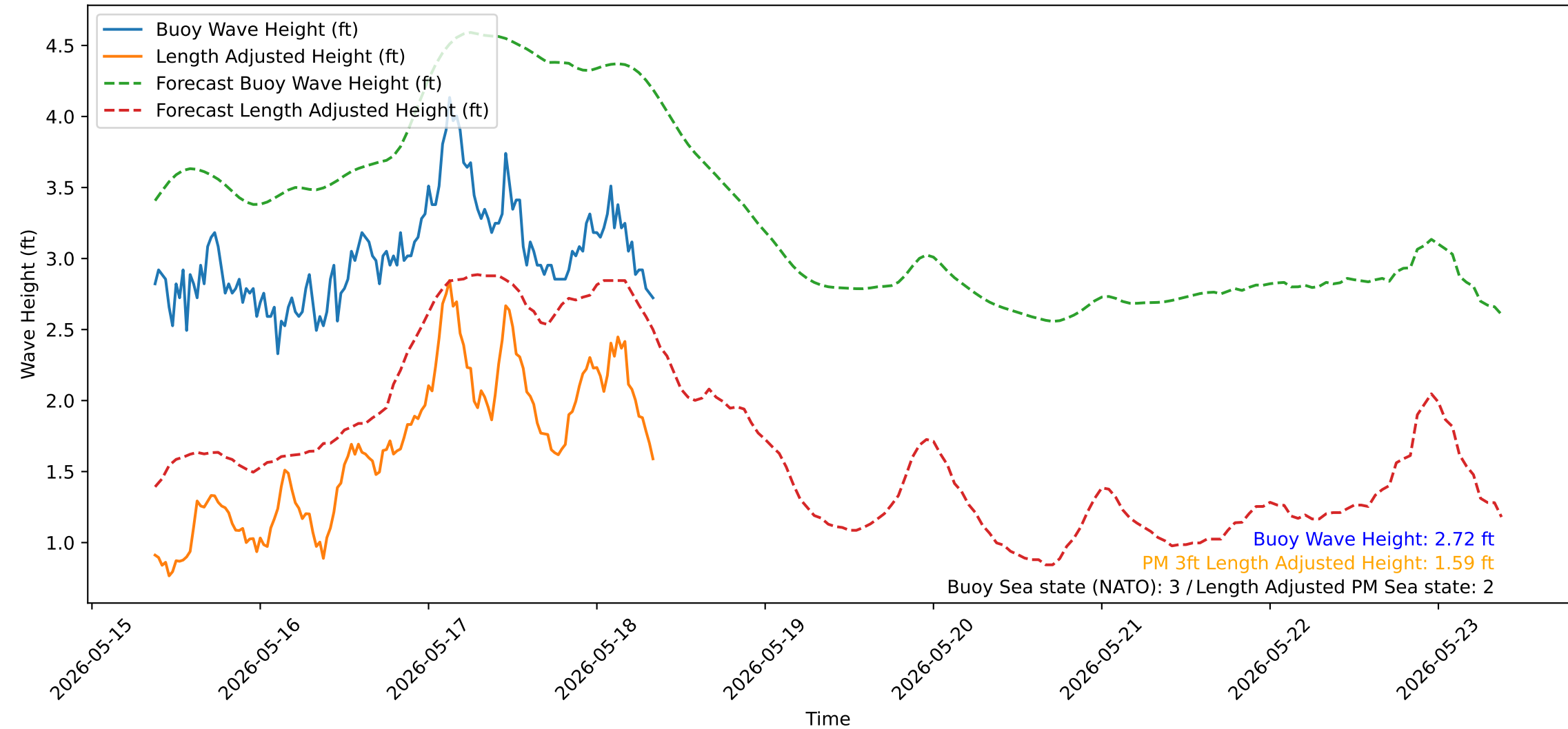
Wave Heights over Time for Red Beach at 2026-05-18 08:40:50
