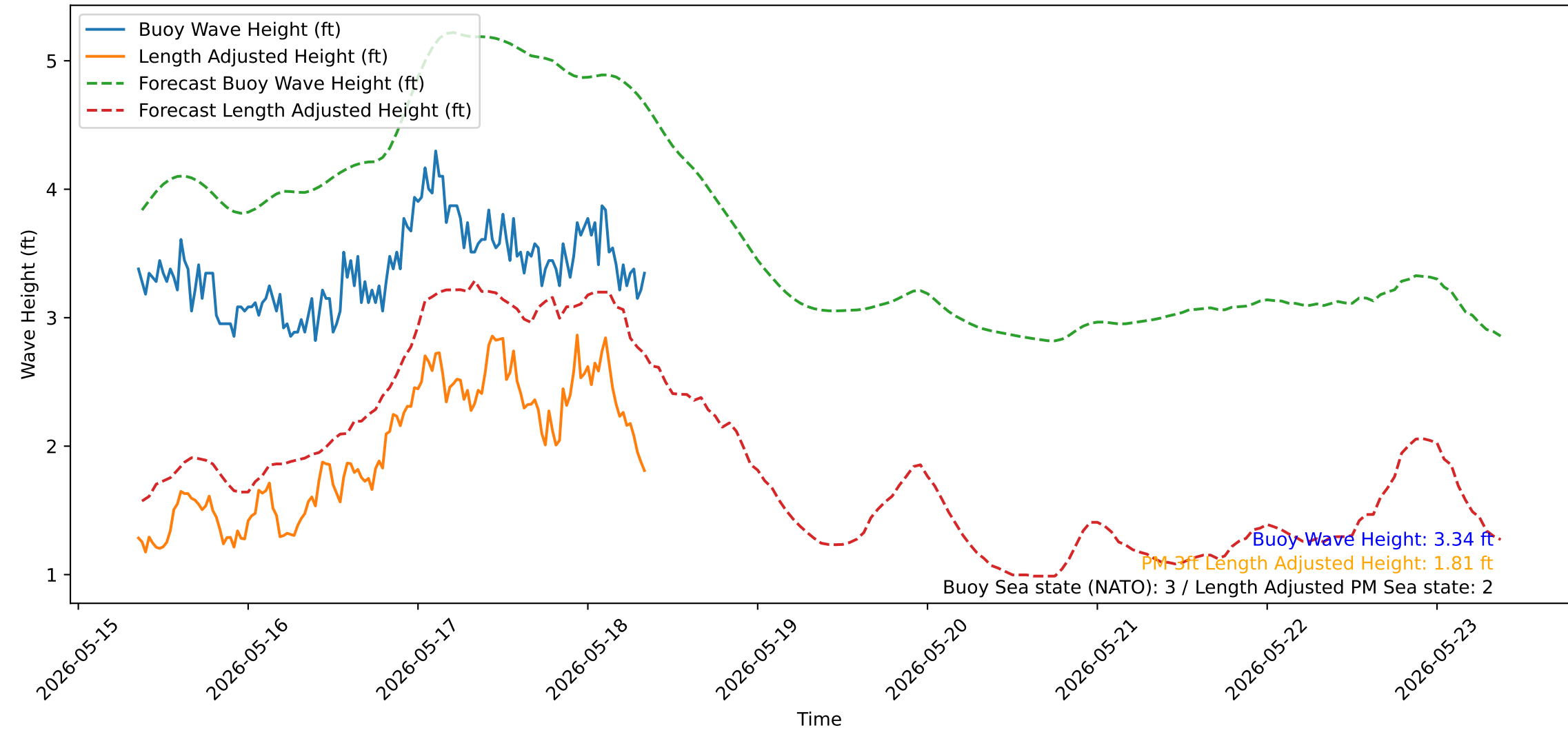
Wave Heights over Time for Oceanside Harbor at 2026-05-18 08:40:31
