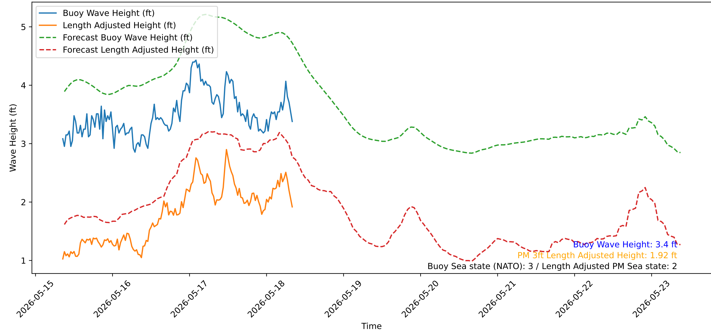
Wave Heights over Time for Green Beach at 2026-05-18 08:41:13
