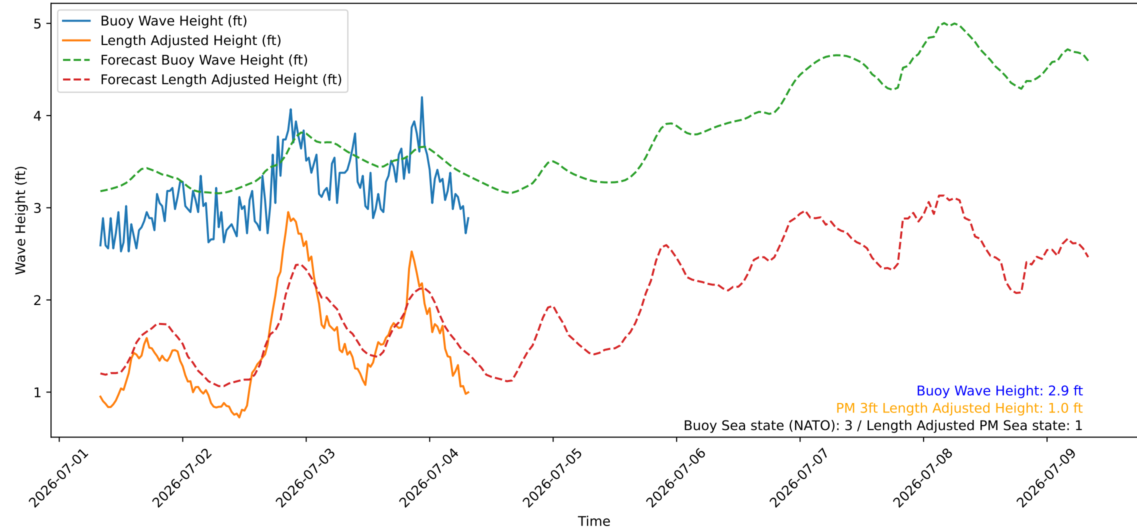
Wave Heights over Time for Green Beach at 2026-07-04 08:11:08
