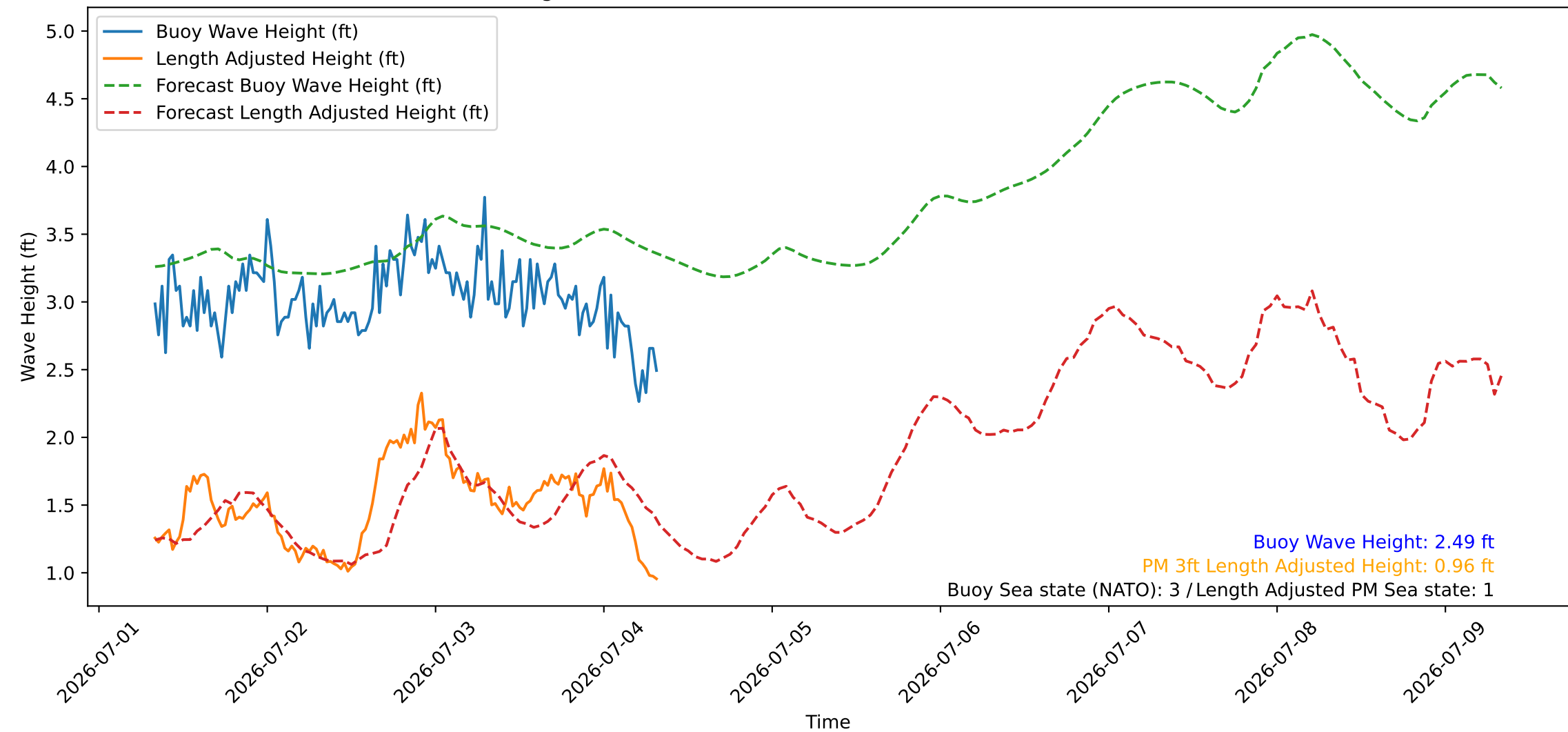
Wave Heights over Time for Oceanside Harbor at 2026-07-04 08:10:26
