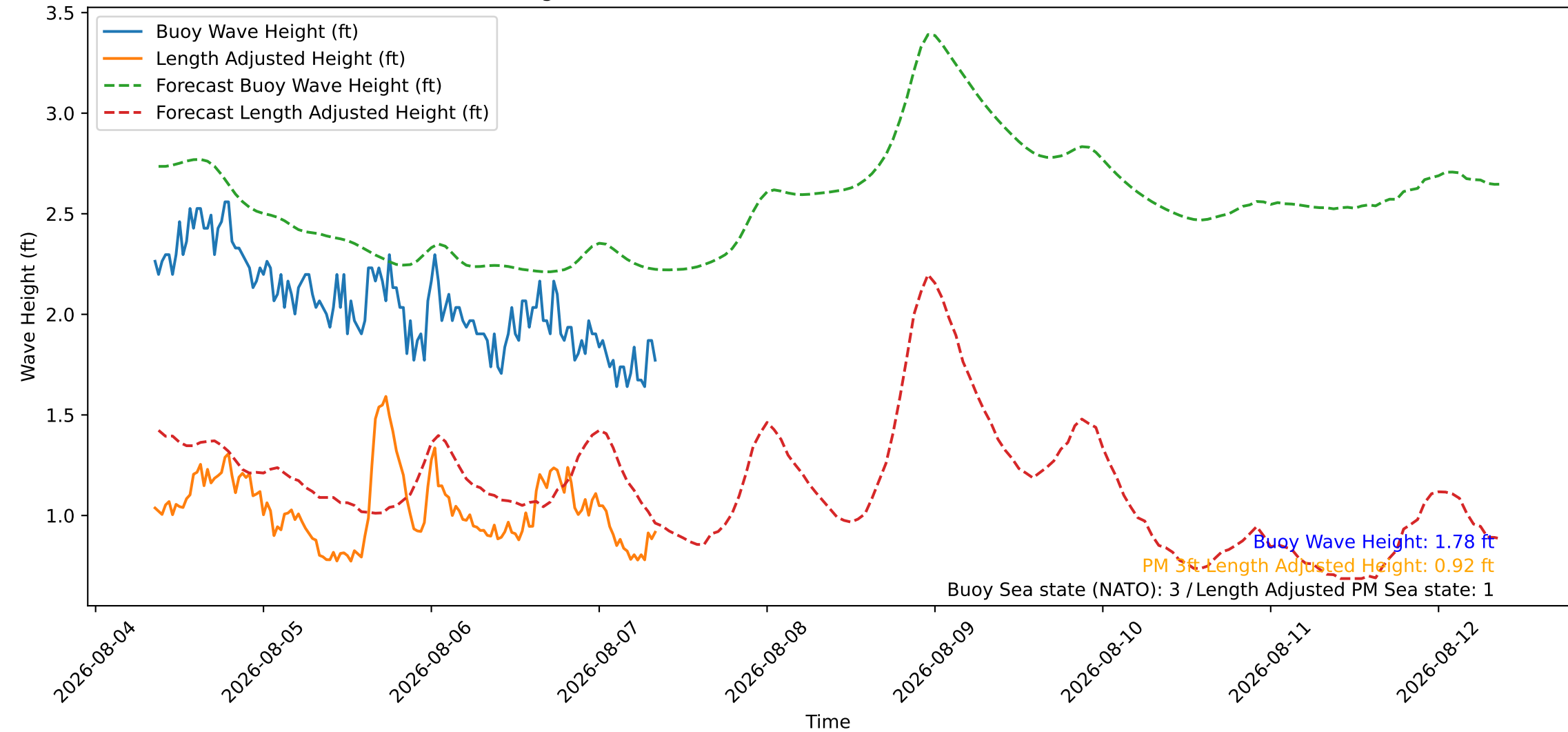
Wave Heights over Time for Oceanside Harbor at 2026-08-07 08:40:26
