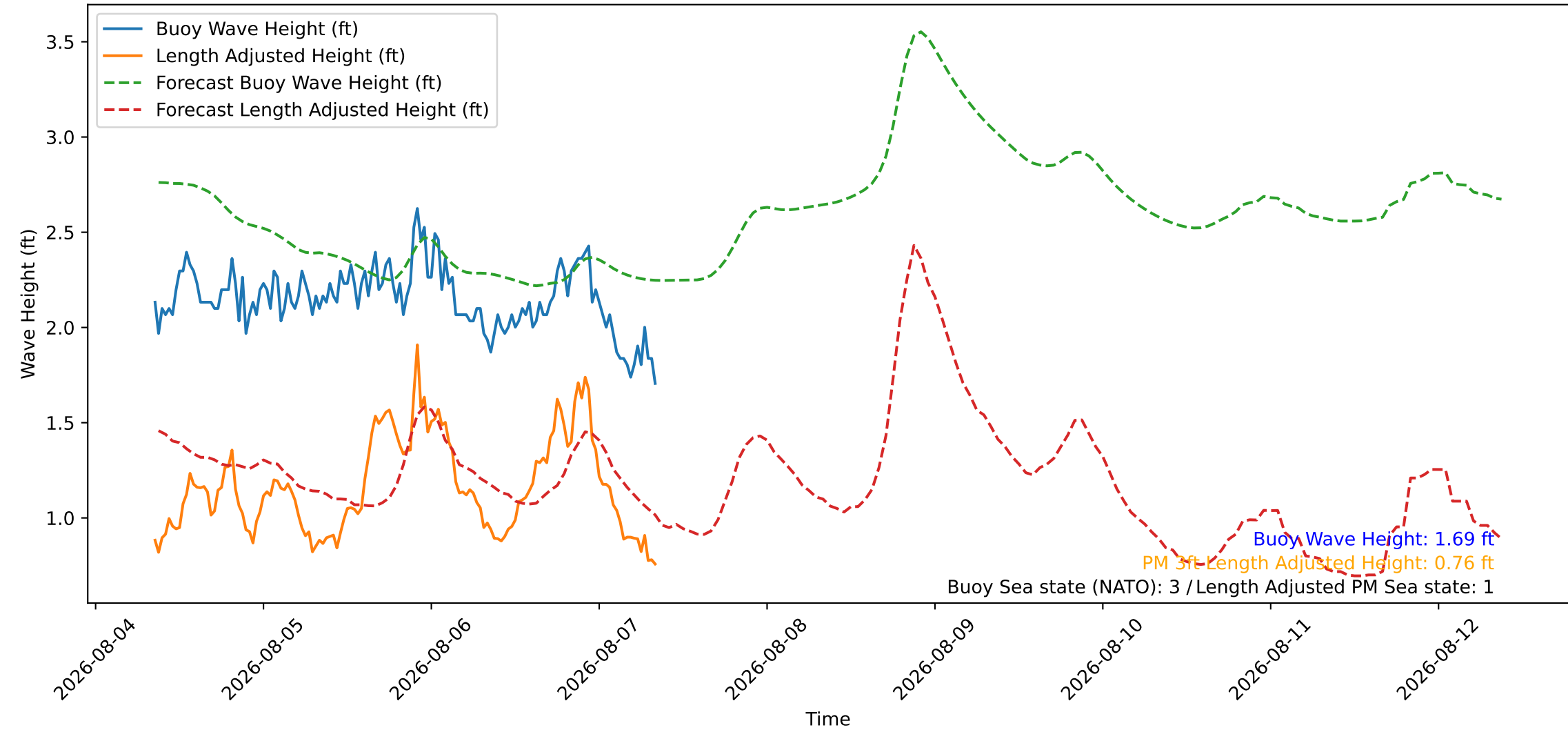
Wave Heights over Time for Green Beach at 2026-08-07 08:41:09
