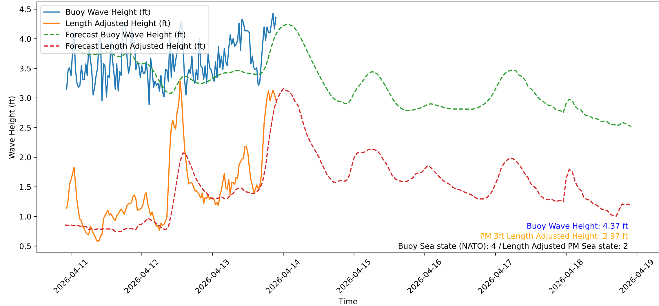
Wave Heights over Time for Red Beach at 2026-04-13 22:10:50
