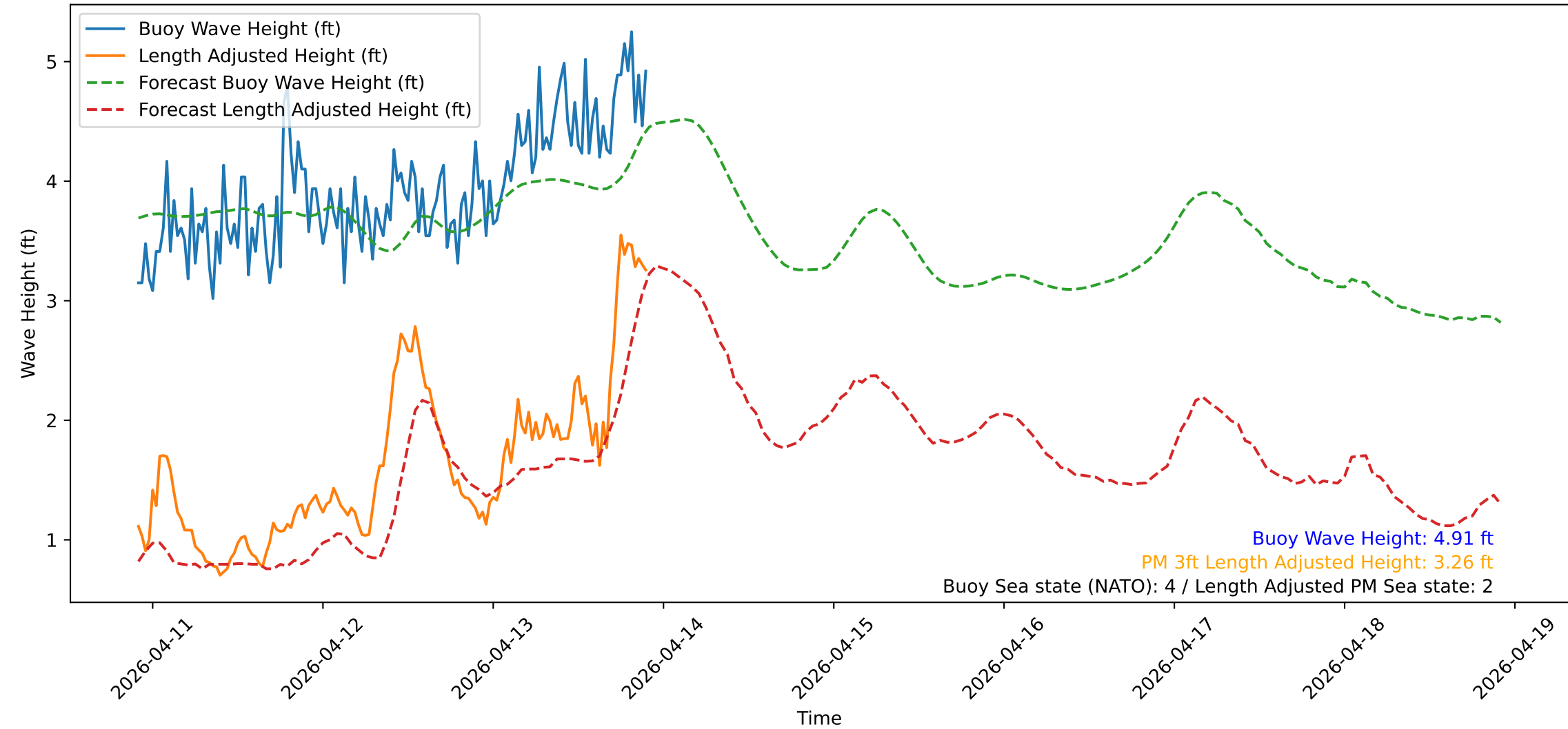
Wave Heights over Time for Oceanside Harbor at 2026-04-13 22:10:31
