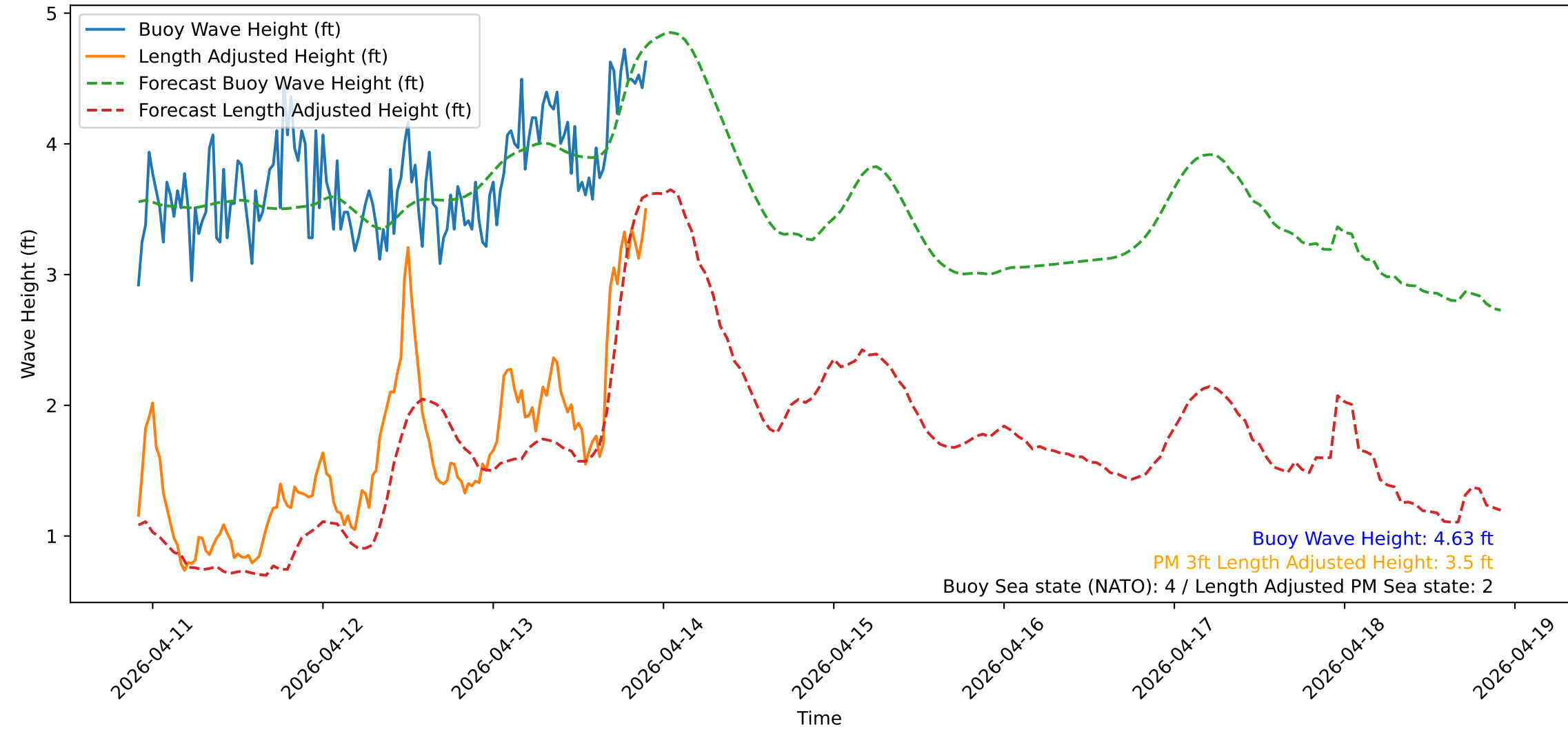
Wave Heights over Time for Green Beach at 2026-04-13 22:11:13
