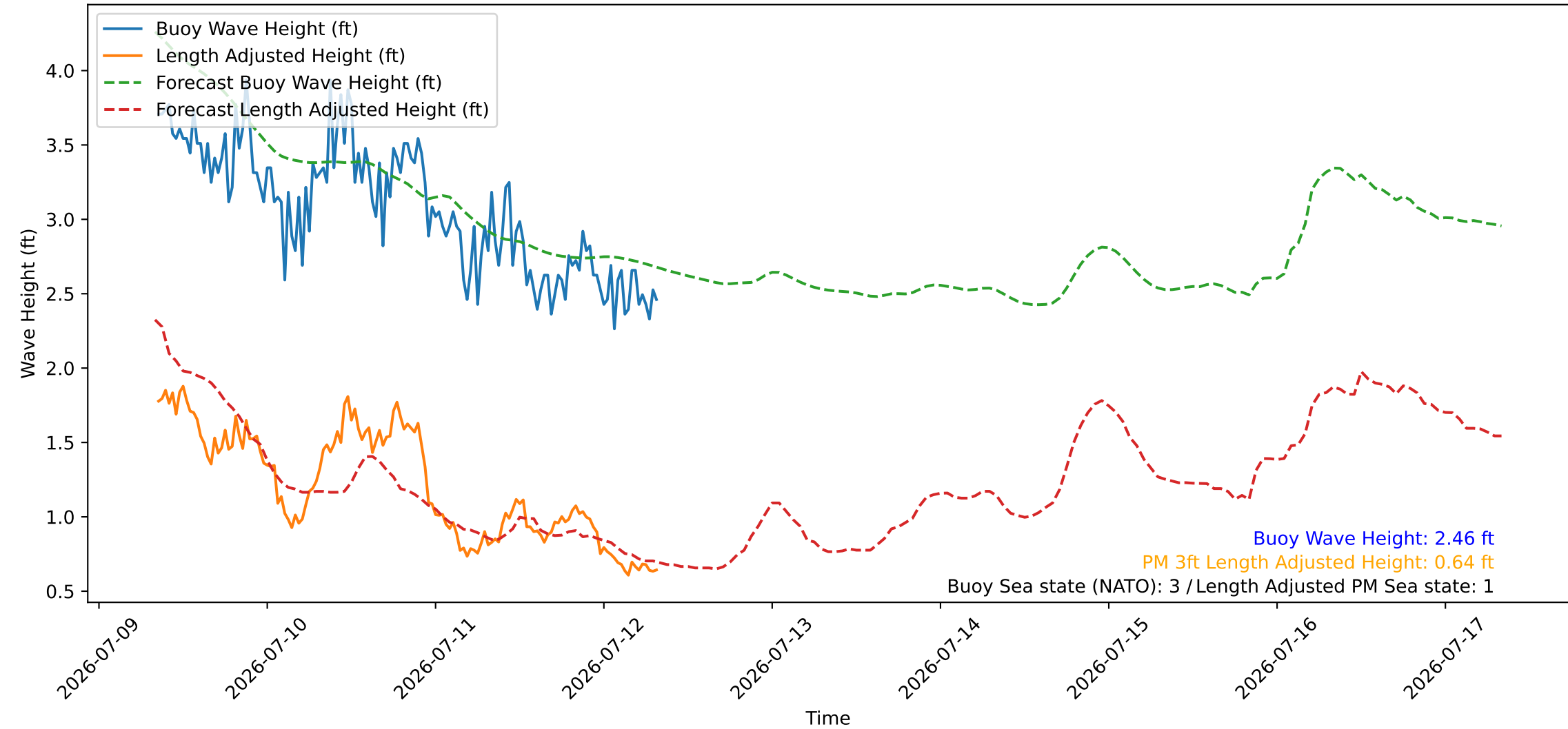
Wave Heights over Time for Red Beach at 2026-07-12 08:20:47
