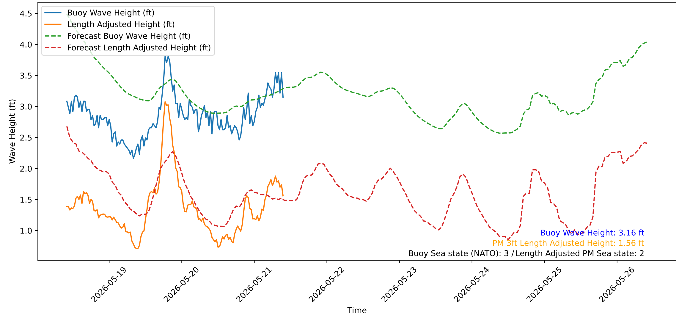
Wave Heights over Time for Green Beach at 2026-05-21 10:11:14
