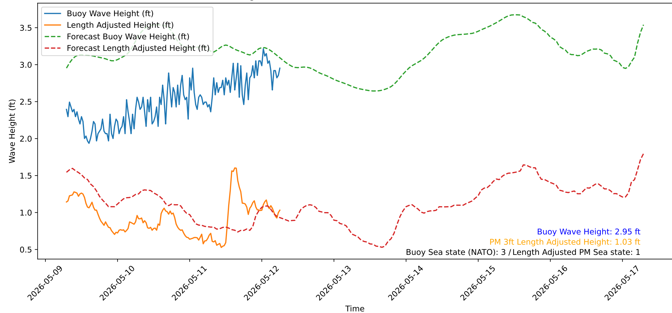
Wave Heights over Time for Red Beach at 2026-05-12 06:40:51
