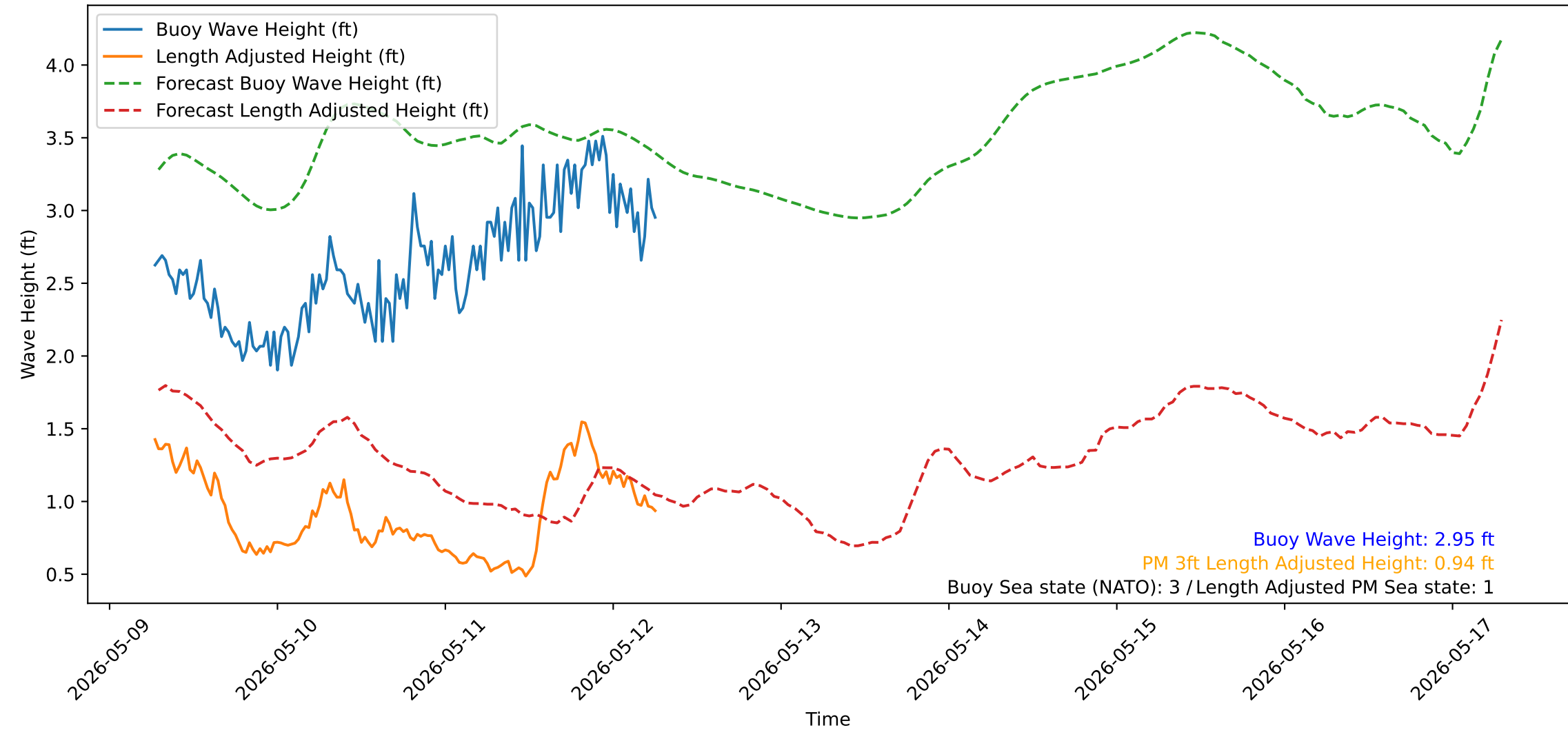
Wave Heights over Time for Green Beach at 2026-05-12 06:41:13
