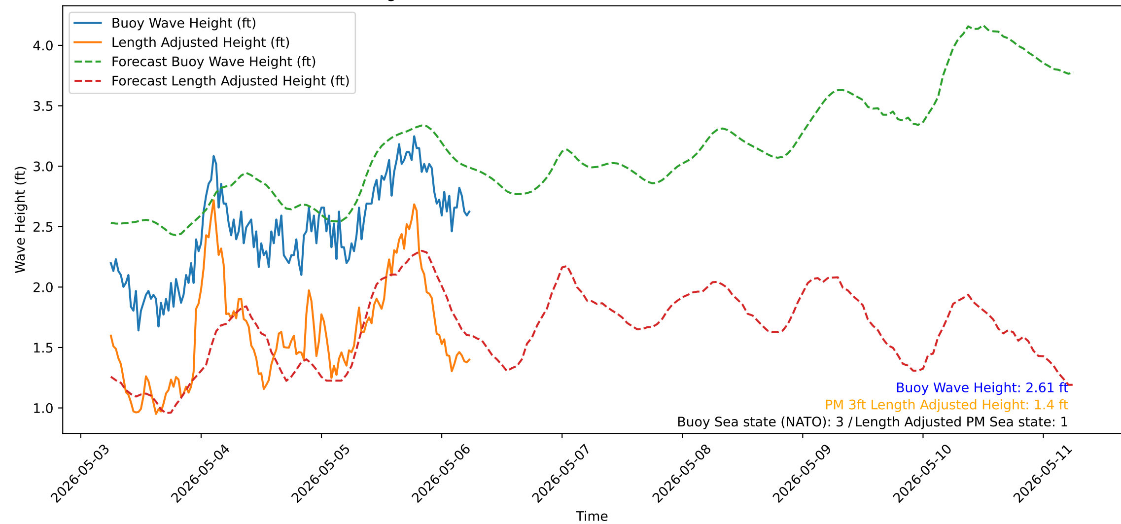
Wave Heights over Time for Oceanside Harbor at 2026-05-06 06:10:31
