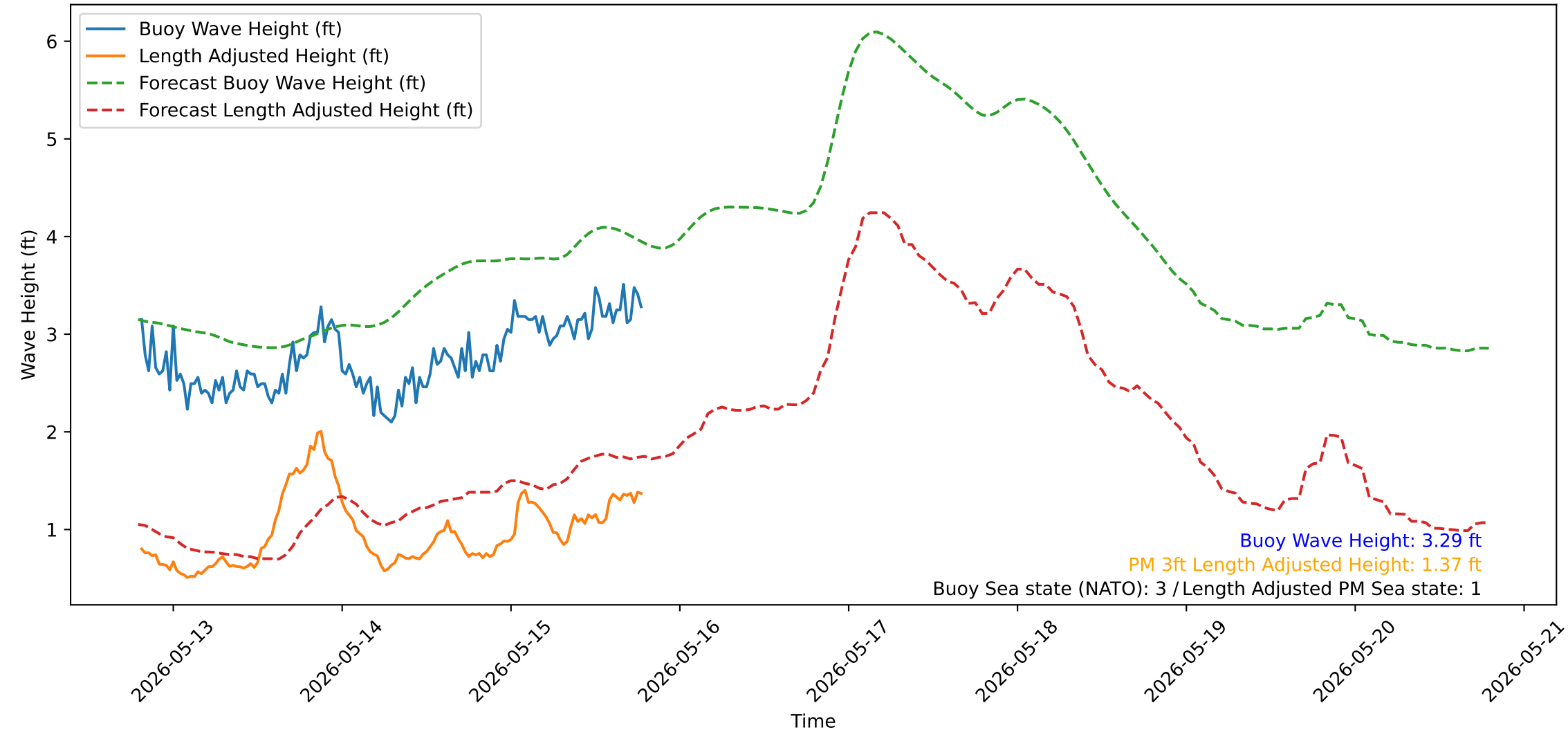
Wave Heights over Time for Green Beach at 2026-05-15 19:21:15
