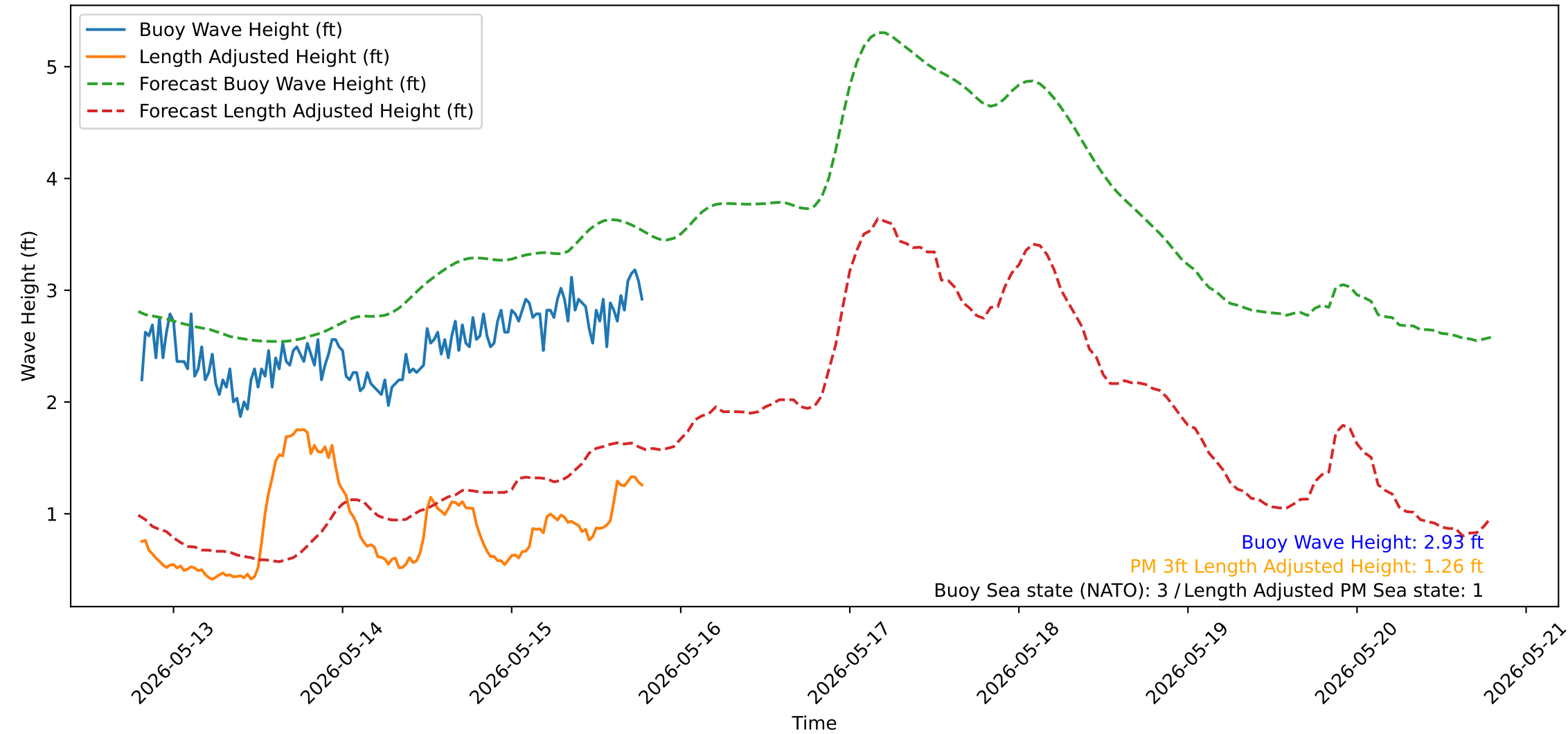
Wave Heights over Time for Red Beach at 2026-05-15 19:20:52
