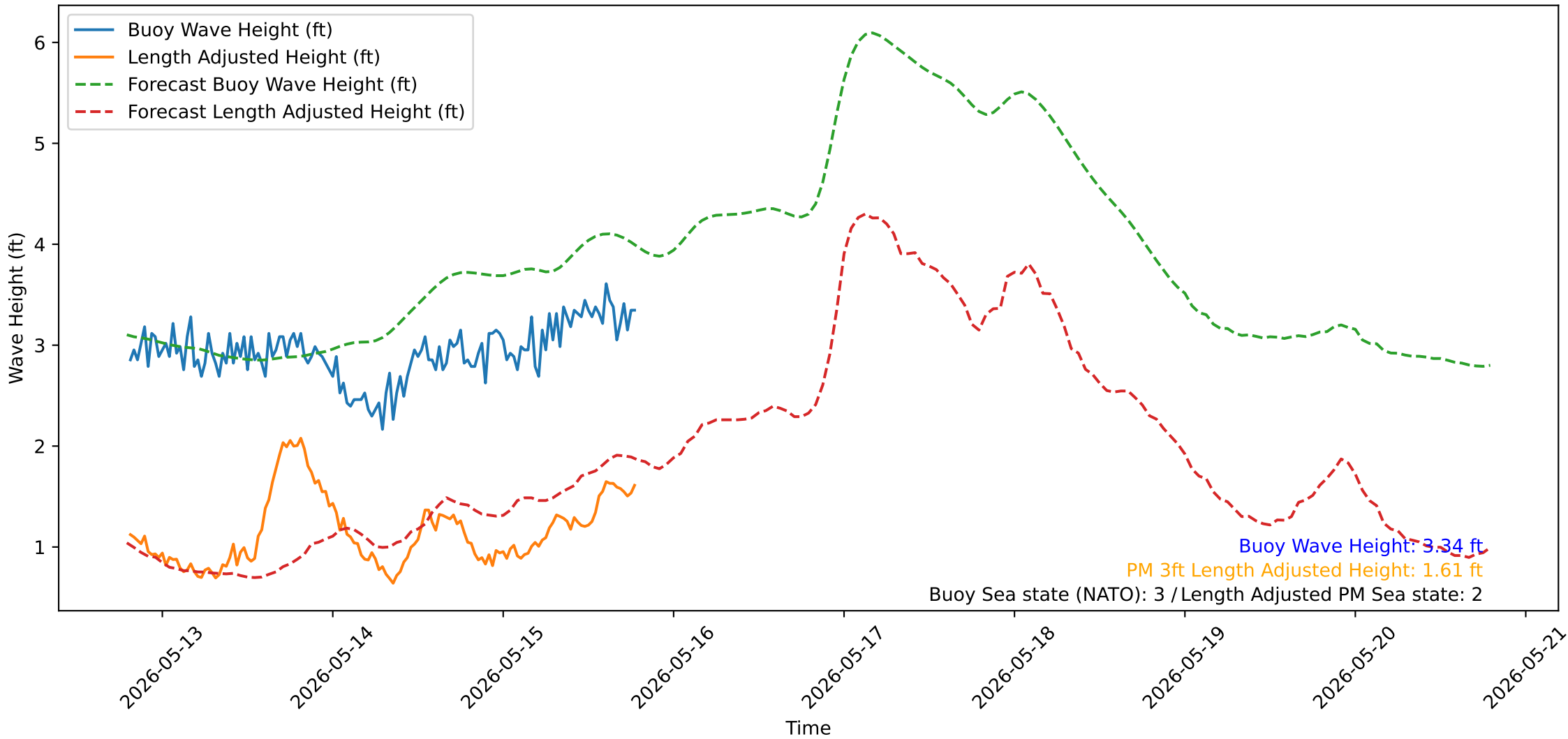
Wave Heights over Time for Oceanside Harbor at 2026-05-15 19:20:32
