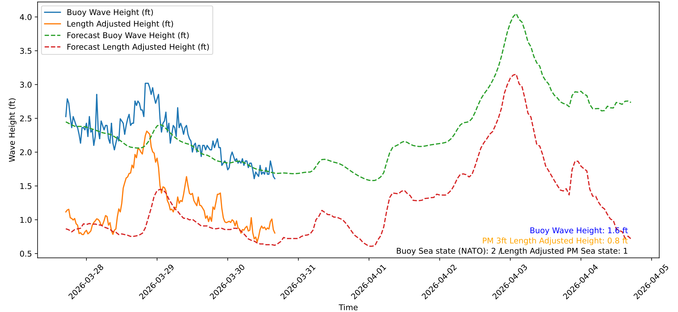
Wave Heights over Time for Red Beach at 2026-03-30 16:40:47
