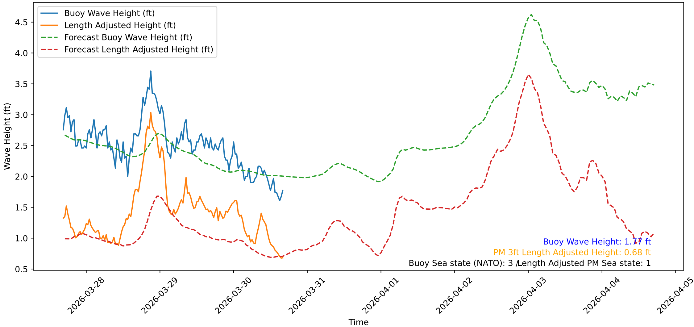
Wave Heights over Time for Green Beach at 2026-03-30 16:41:10
