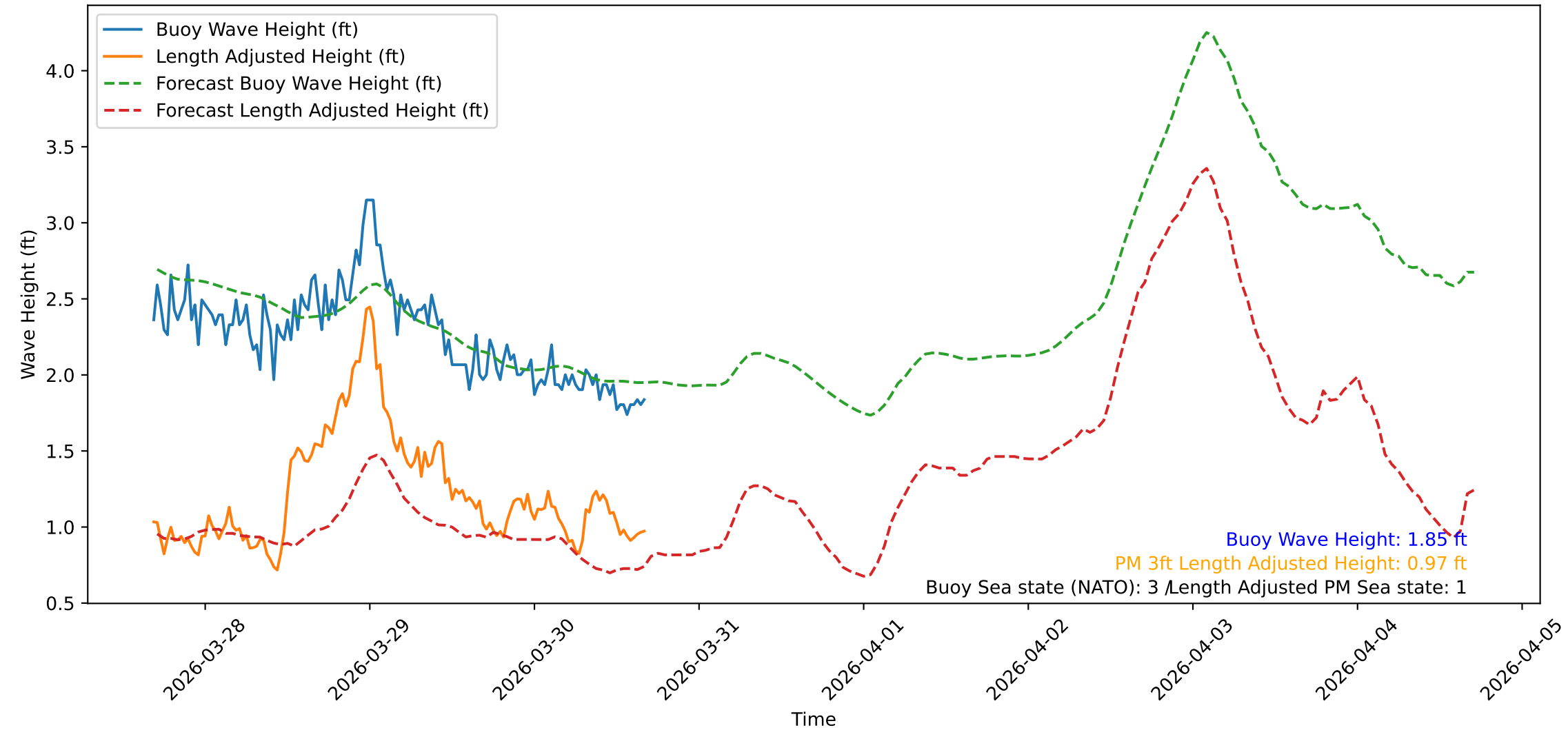
Wave Heights over Time for Oceanside Harbor at 2026-03-30 16:40:31
