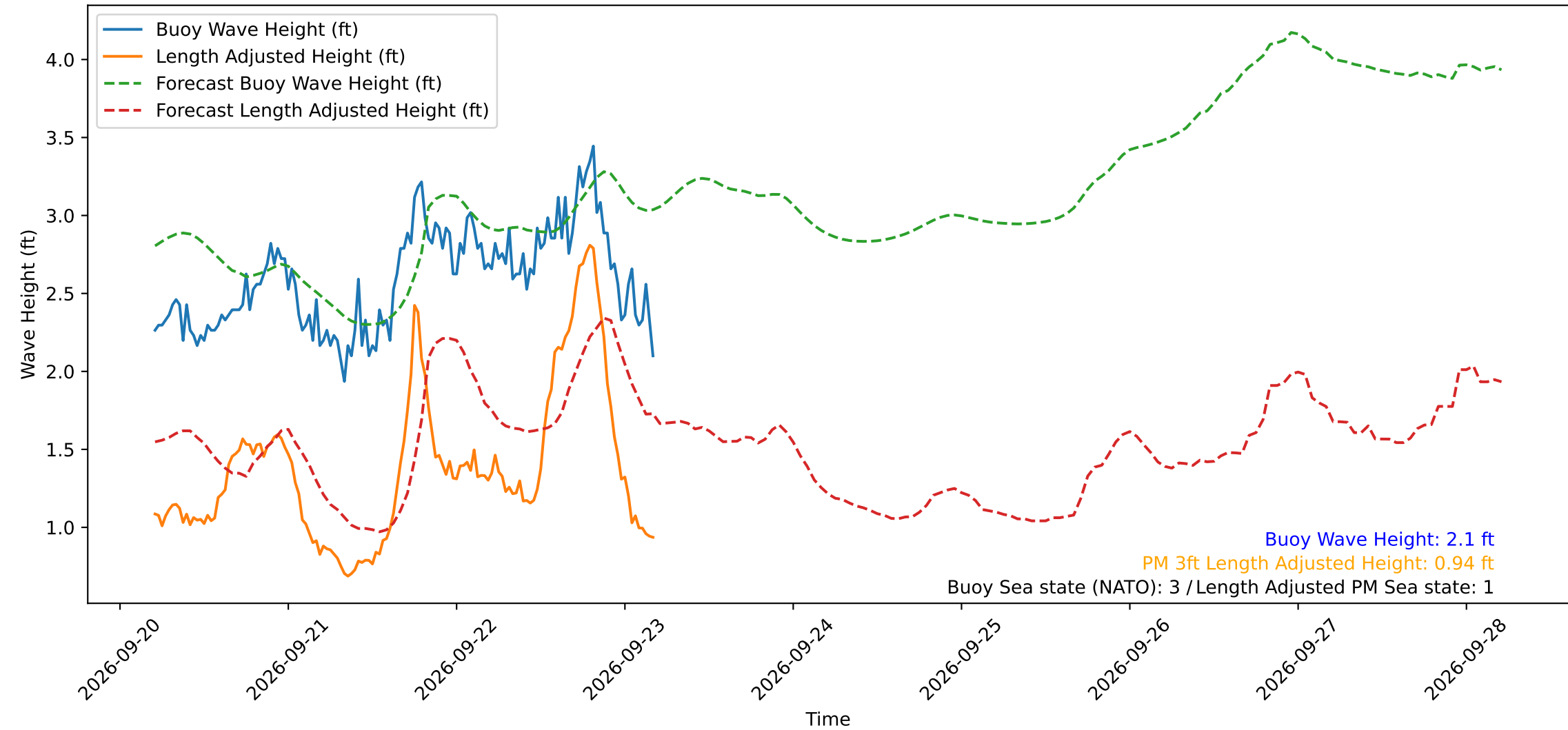
Wave Heights over Time for Green Beach at 2026-09-23 04:41:12
