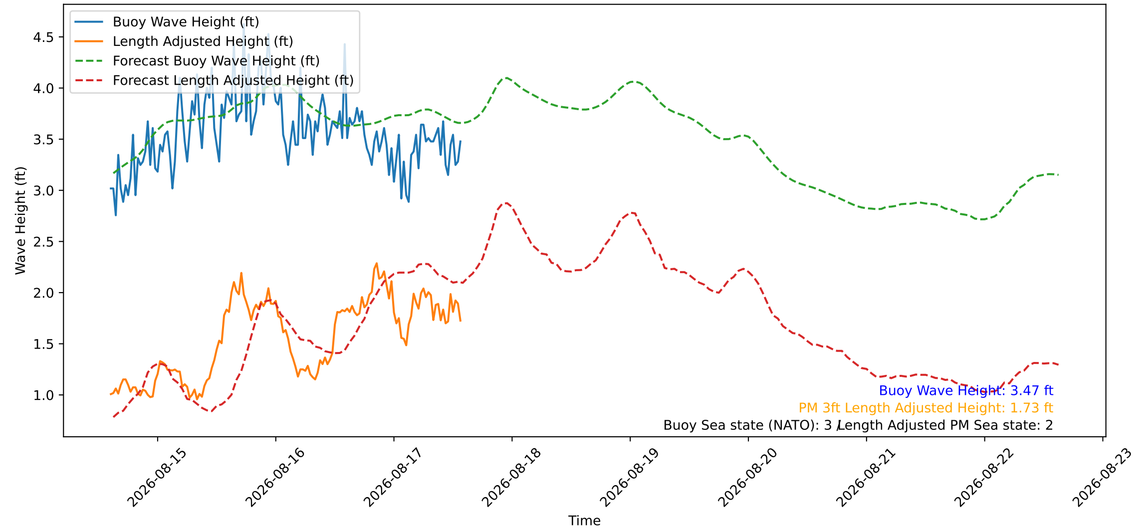
Wave Heights over Time for Oceanside Harbor at 2026-08-17 14:30:26
