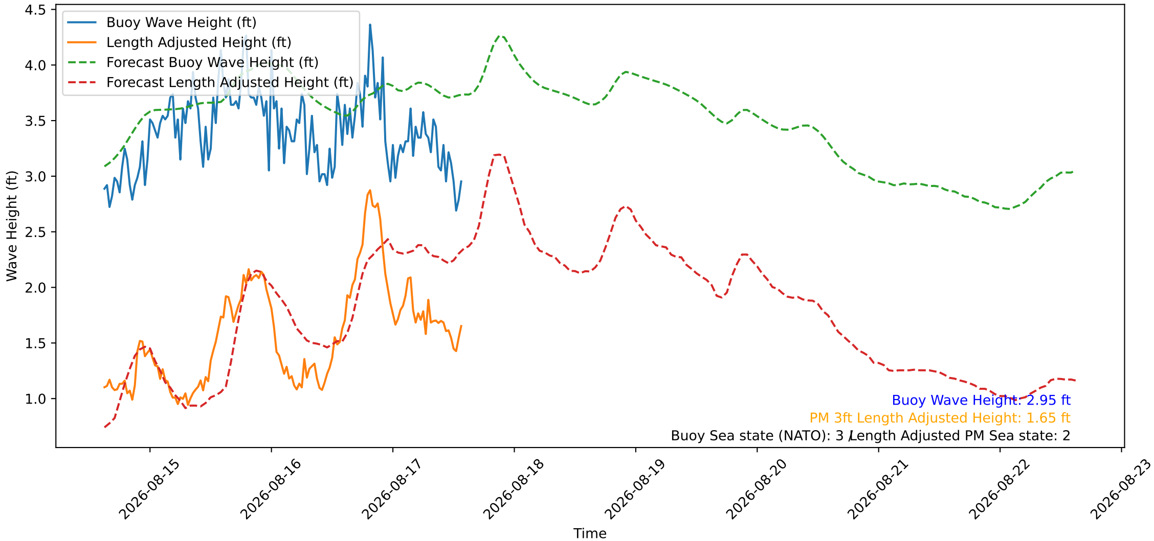
Wave Heights over Time for Green Beach at 2026-08-17 14:31:08
