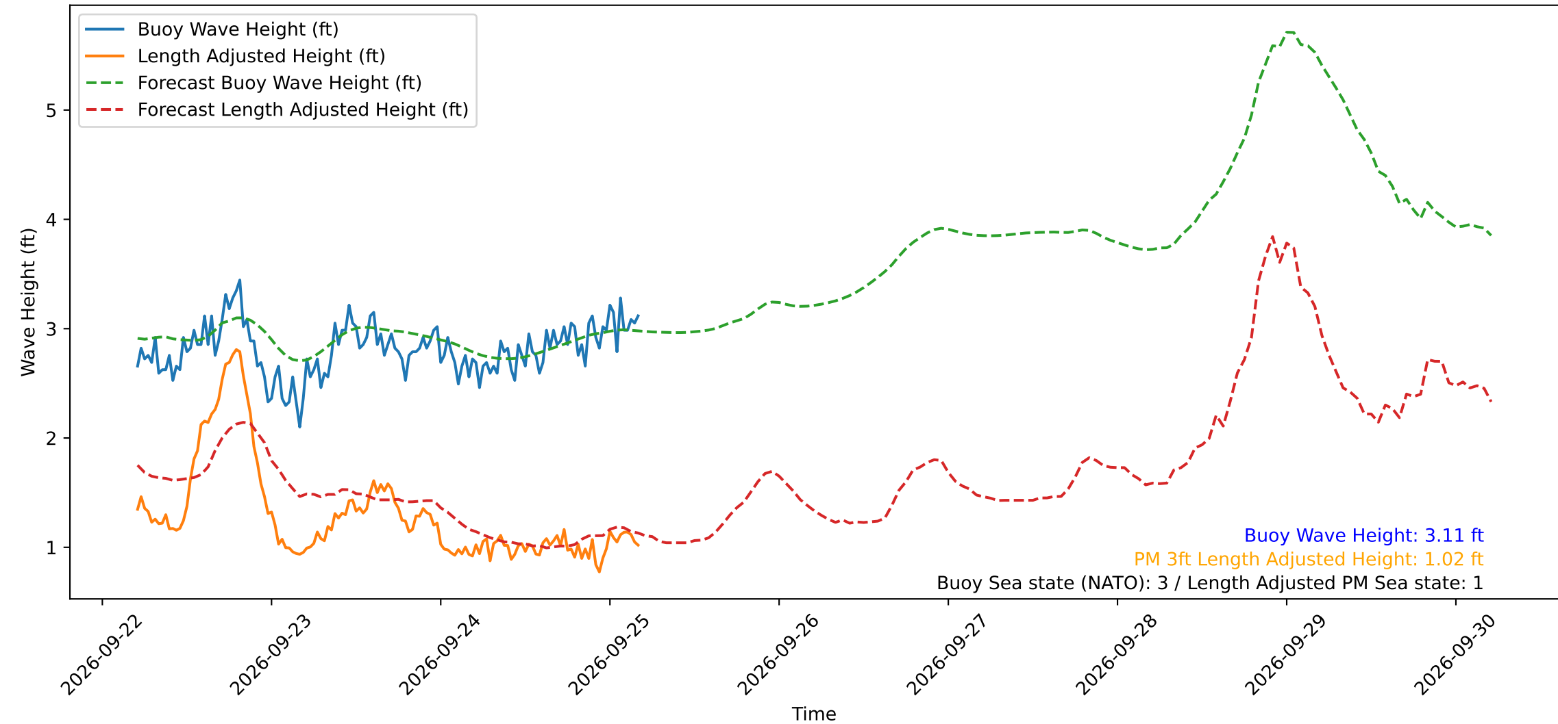
Wave Heights over Time for Green Beach at 2026-09-25 04:41:11
