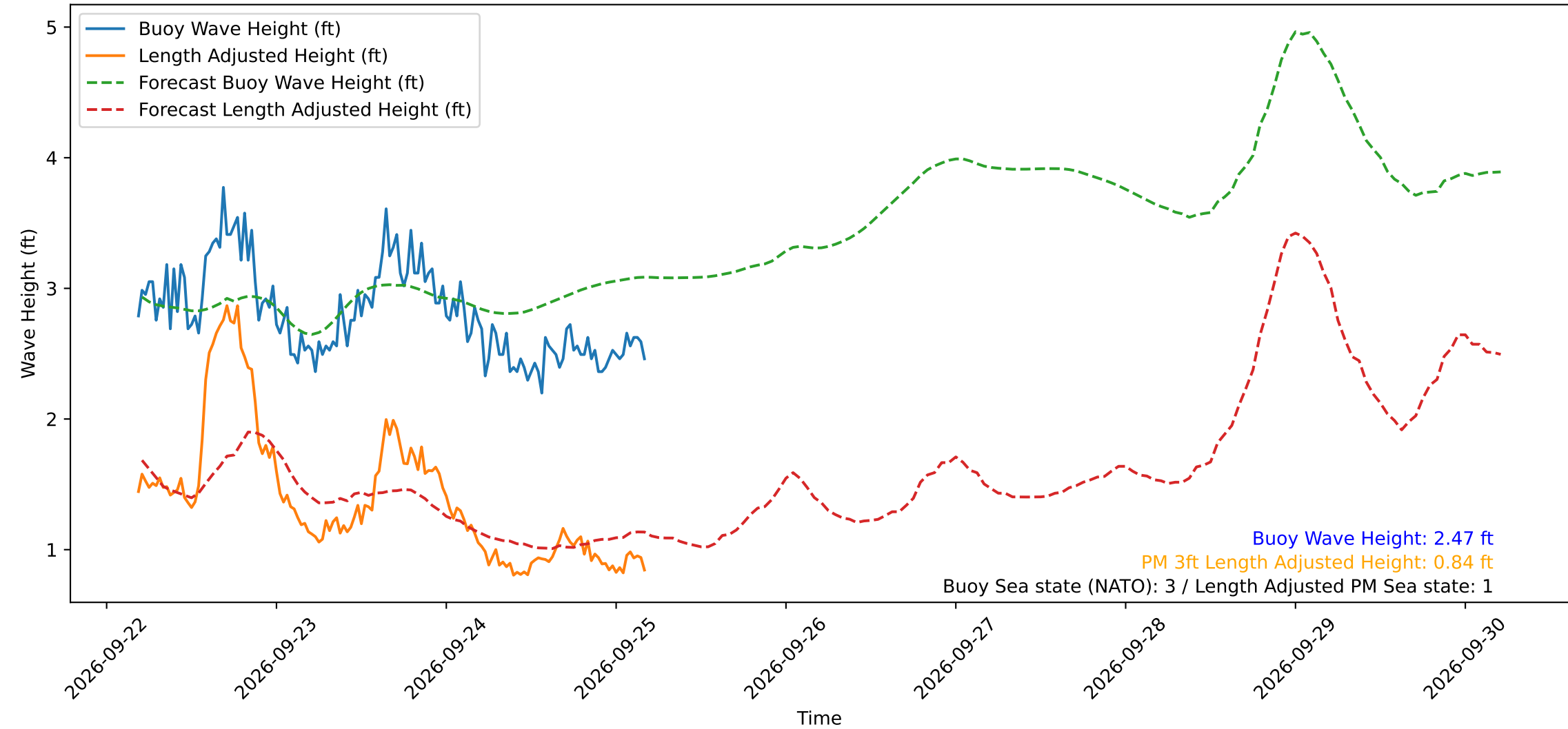
Wave Heights over Time for Oceanside Harbor at 2026-09-25 04:40:30
