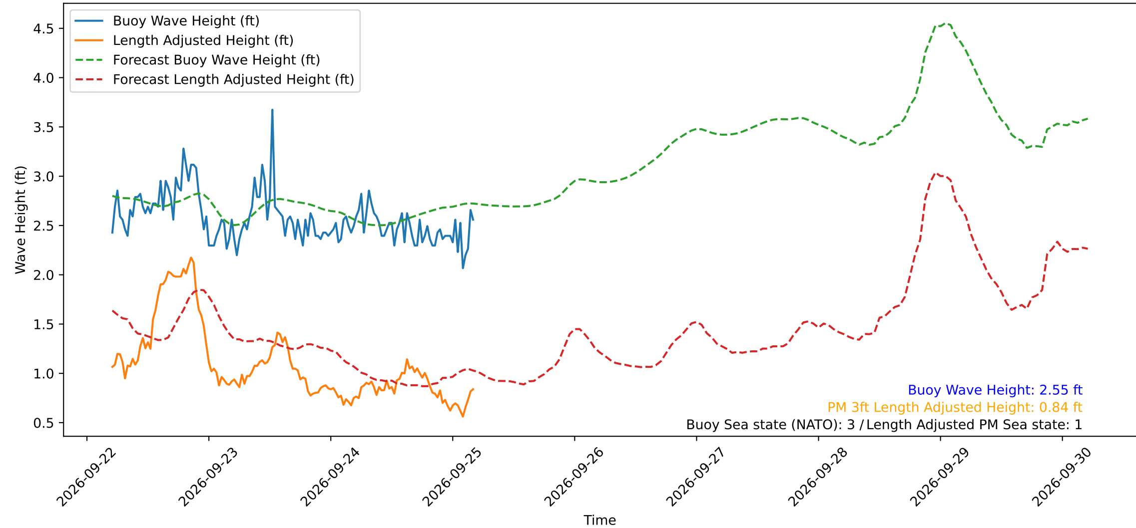
Wave Heights over Time for Red Beach at 2026-09-25 04:40:49
