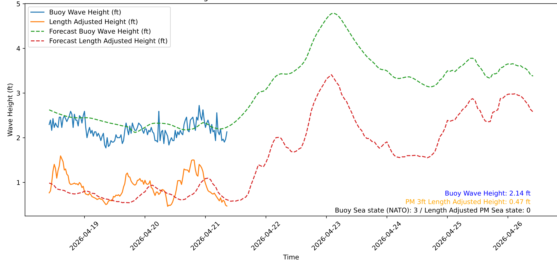
Wave Heights over Time for Red Beach at 2026-04-21 09:30:51
