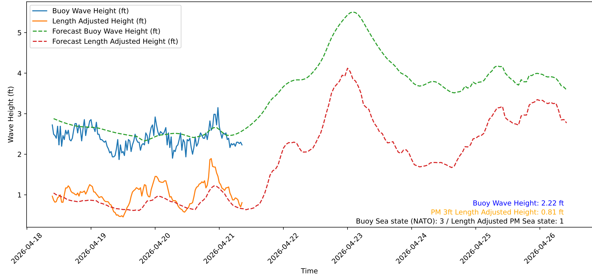
Wave Heights over Time for Green Beach at 2026-04-21 09:31:14
