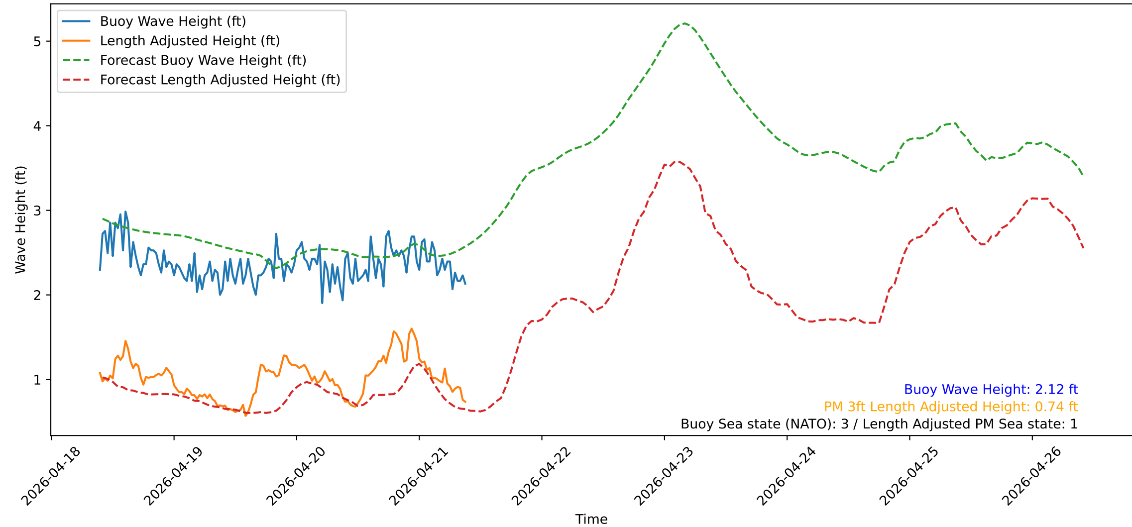
Wave Heights over Time for Oceanside Harbor at 2026-04-21 09:30:31
