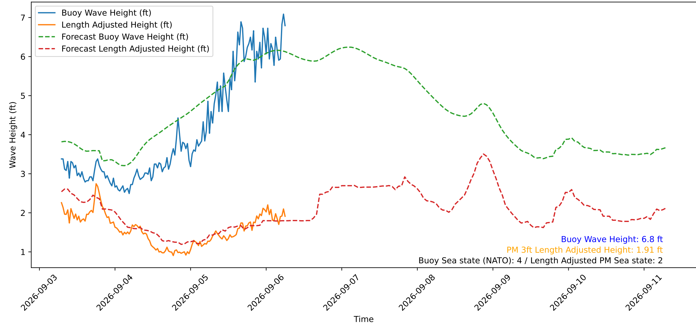
Wave Heights over Time for Green Beach at 2026-09-06 06:51:15
