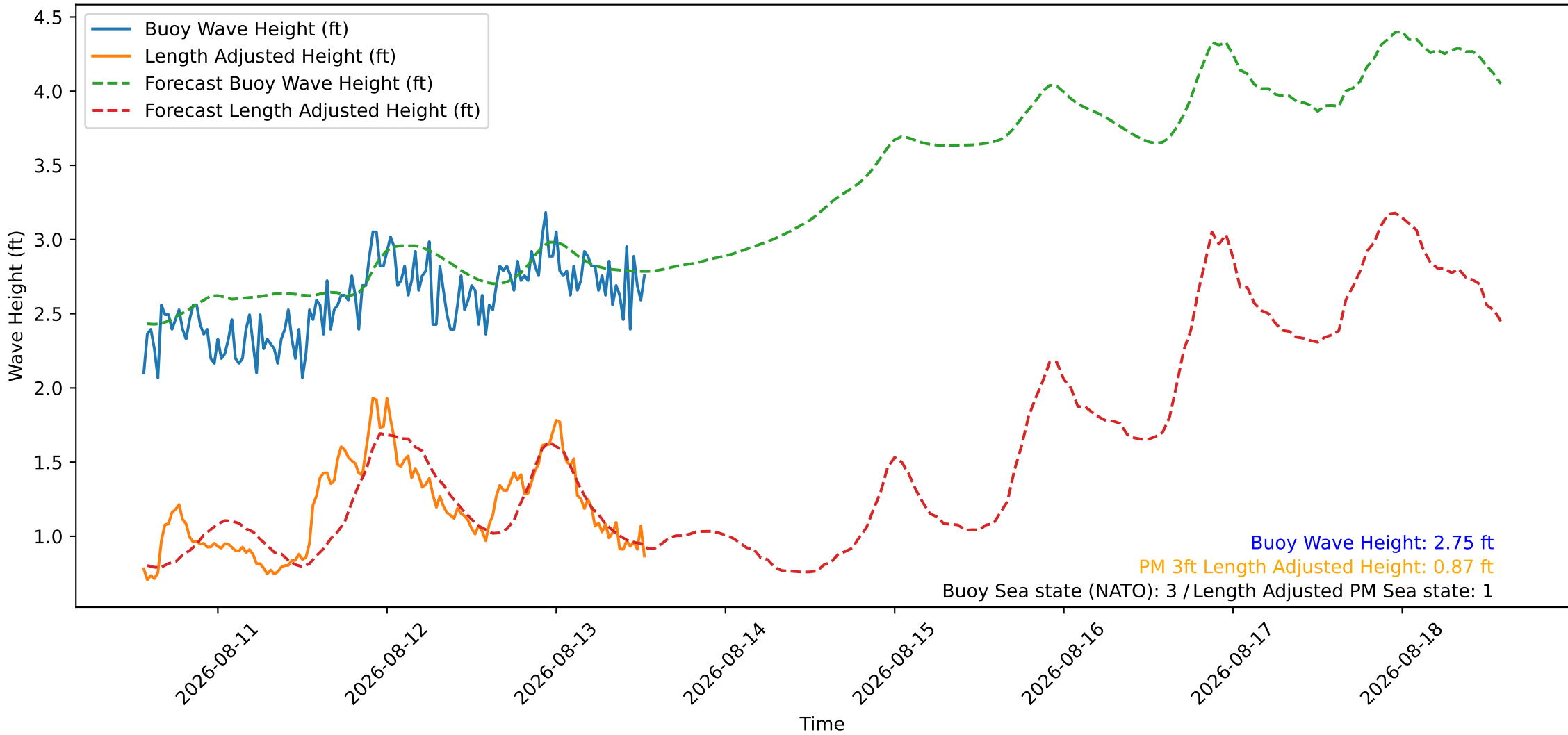
Wave Heights over Time for Oceanside Harbor at 2026-08-13 13:30:27
