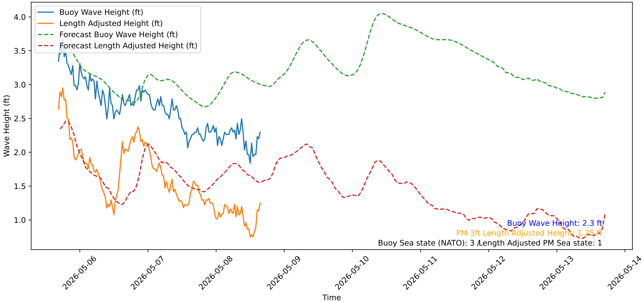
Wave Heights over Time for Green Beach at 2026-05-08 16:31:13
