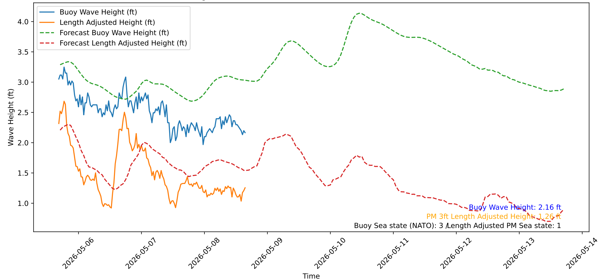
Wave Heights over Time for Oceanside Harbor at 2026-05-08 16:30:32
