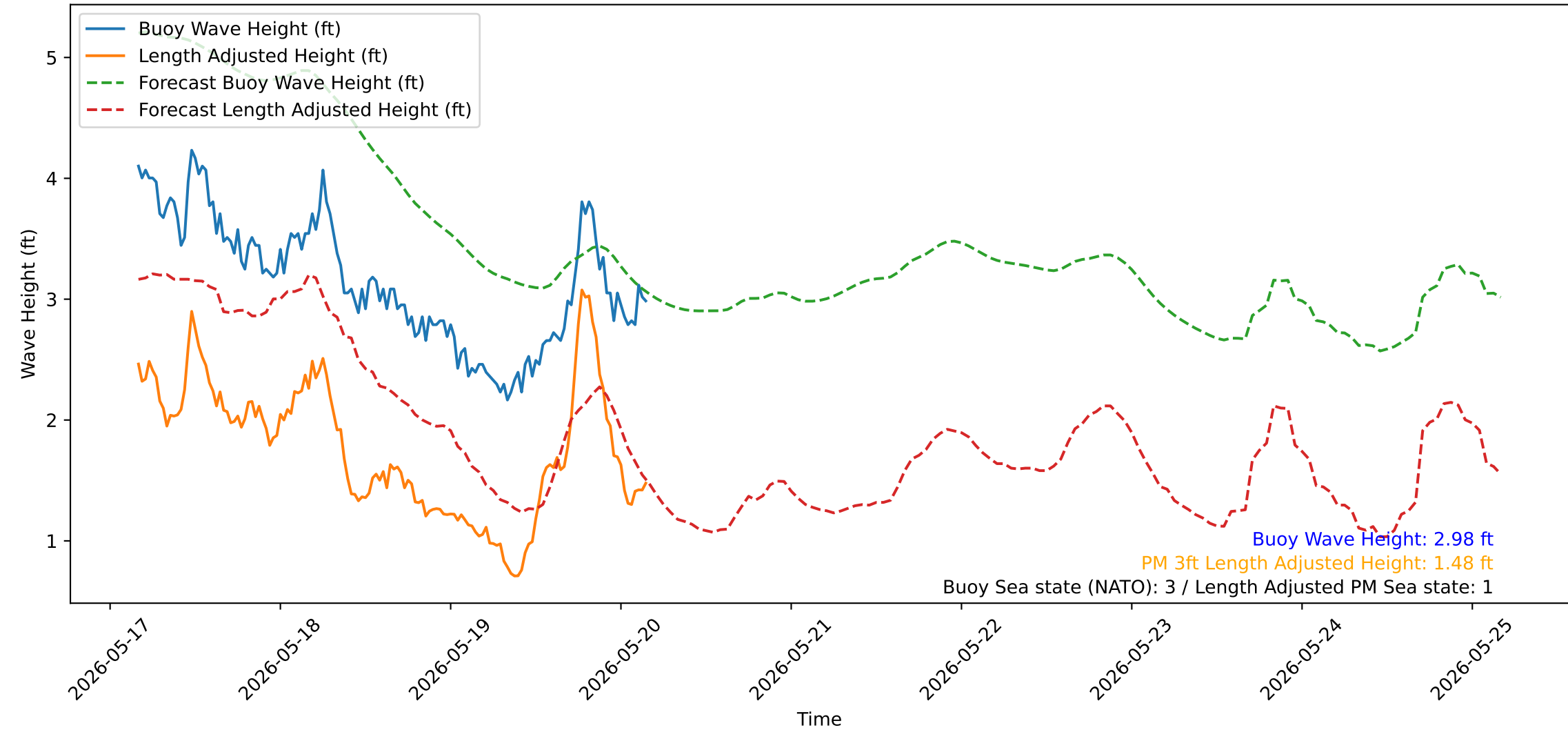
Wave Heights over Time for Green Beach at 2026-05-20 04:11:14
