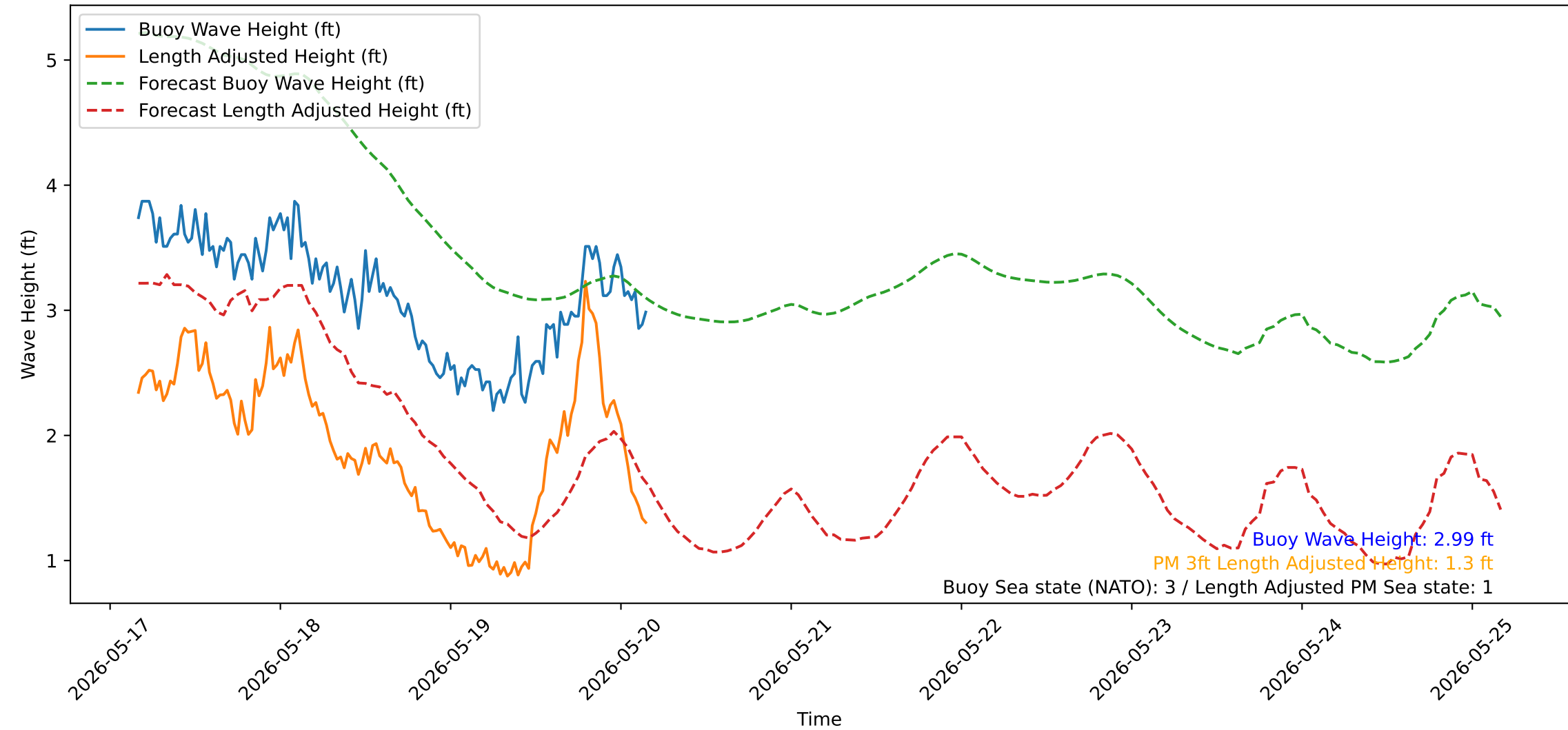
Wave Heights over Time for Oceanside Harbor at 2026-05-20 04:10:32
