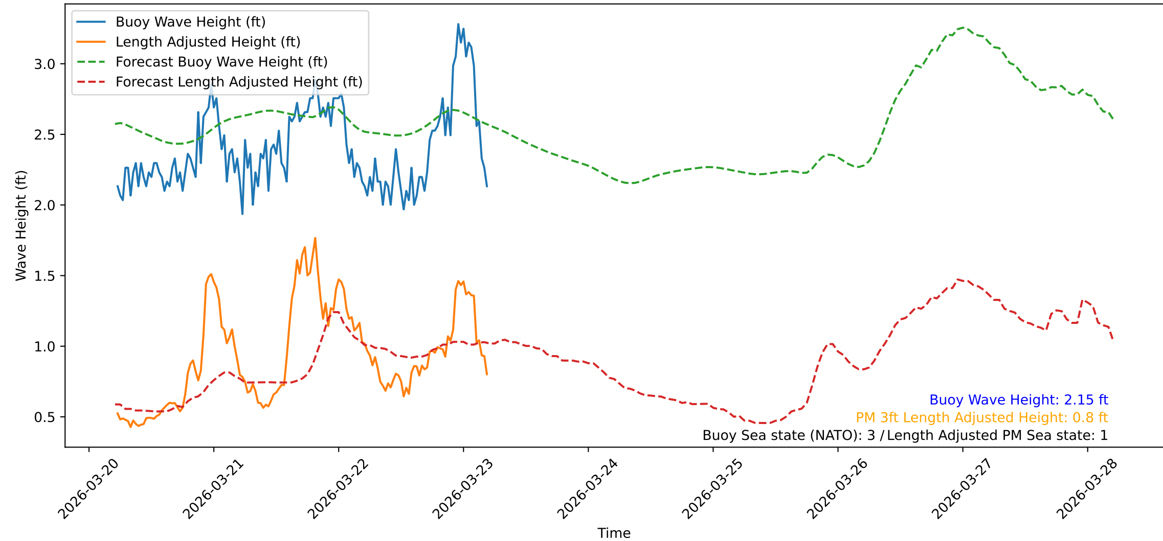
Wave Heights over Time for Green Beach at 2026-03-23 05:21:10
