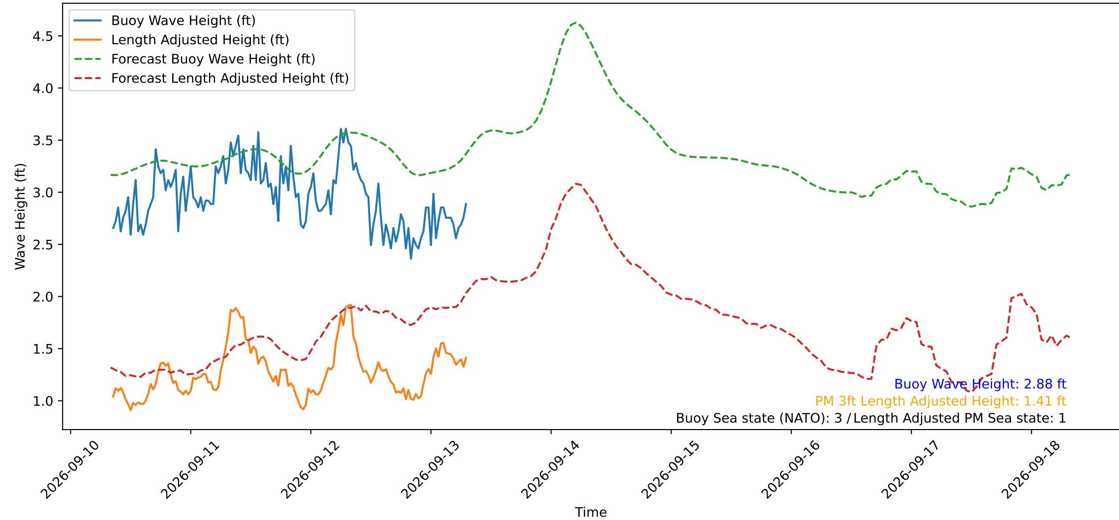
Wave Heights over Time for Green Beach at 2026-09-13 08:01:11
