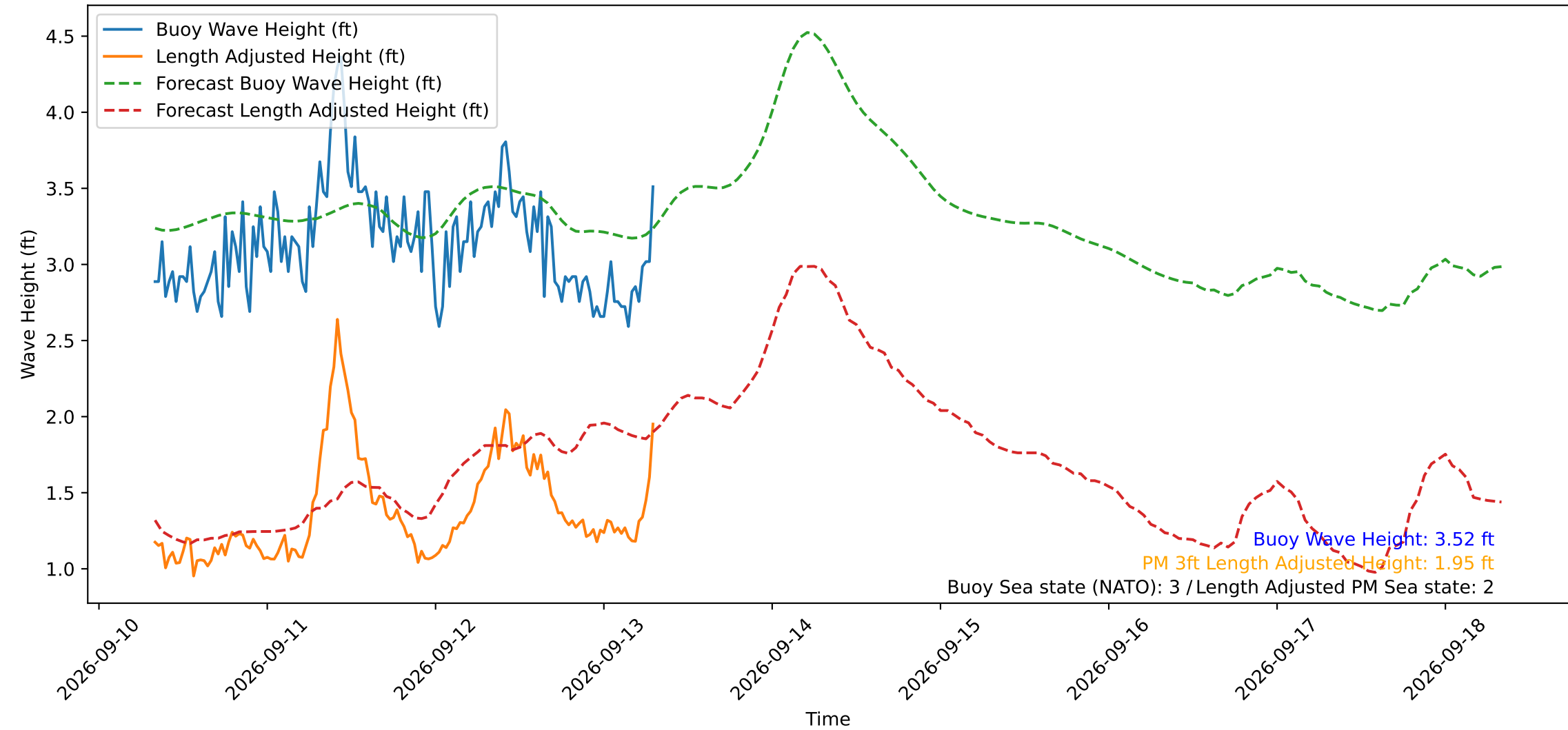
Wave Heights over Time for Oceanside Harbor at 2026-09-13 08:00:29
