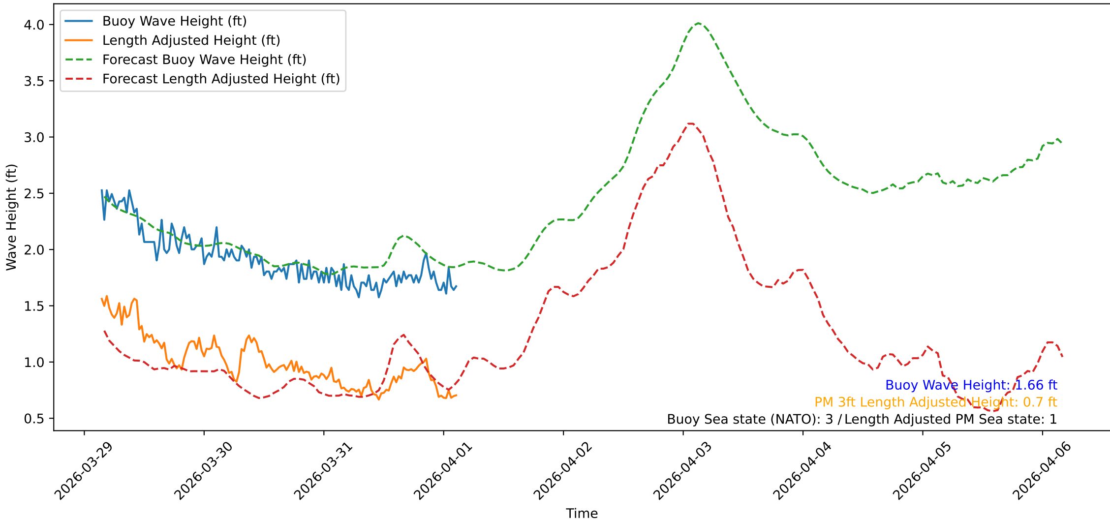
Wave Heights over Time for Oceanside Harbor at 2026-04-01 03:30:32
