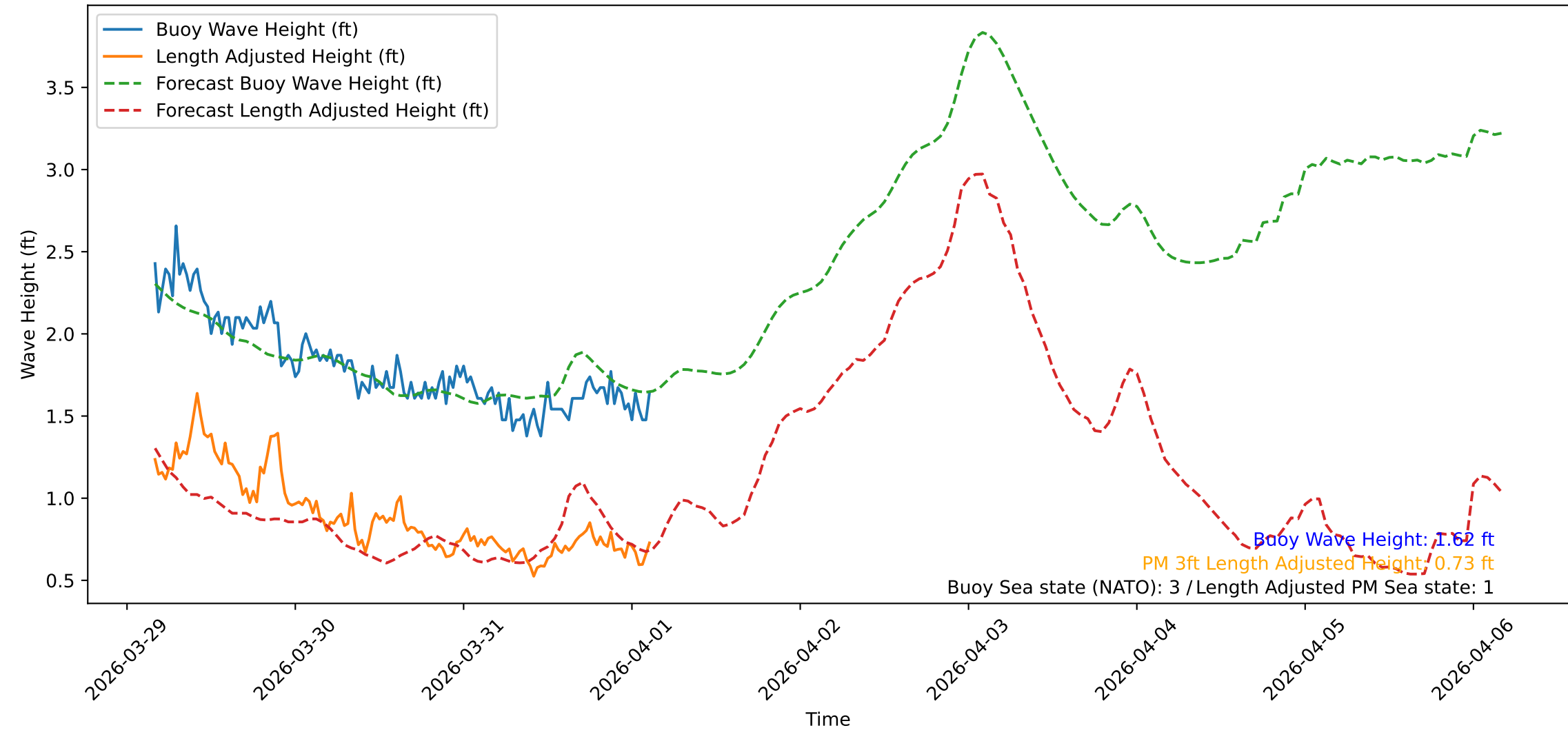
Wave Heights over Time for Red Beach at 2026-04-01 03:30:48
