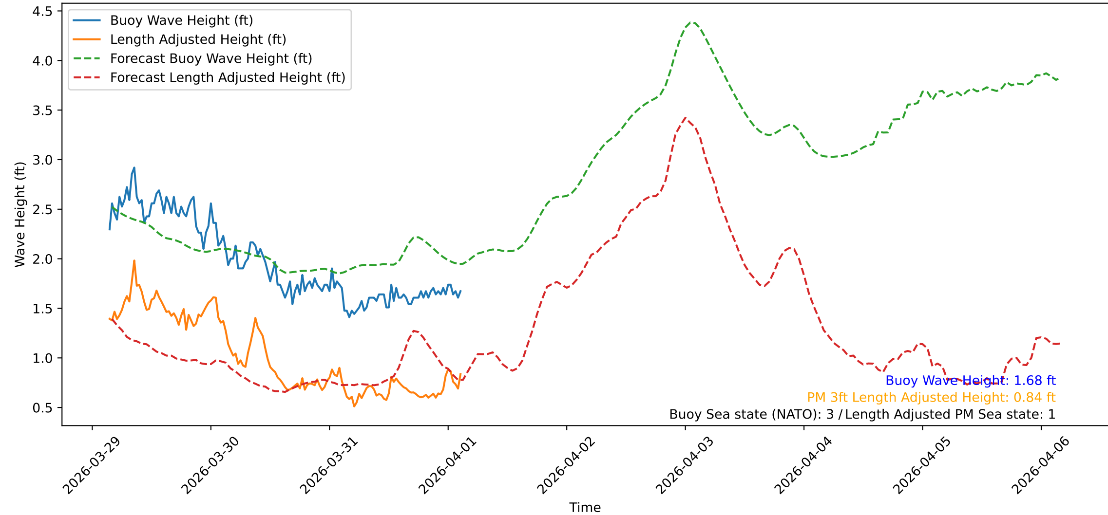
Wave Heights over Time for Green Beach at 2026-04-01 03:31:11
