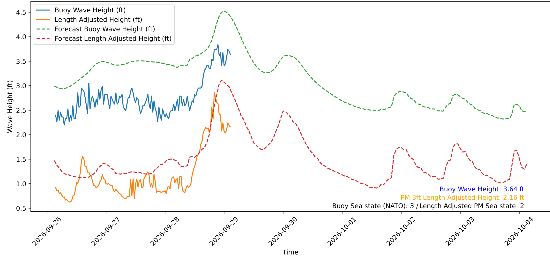
Wave Heights over Time for Red Beach at 2026-09-29 03:10:50
