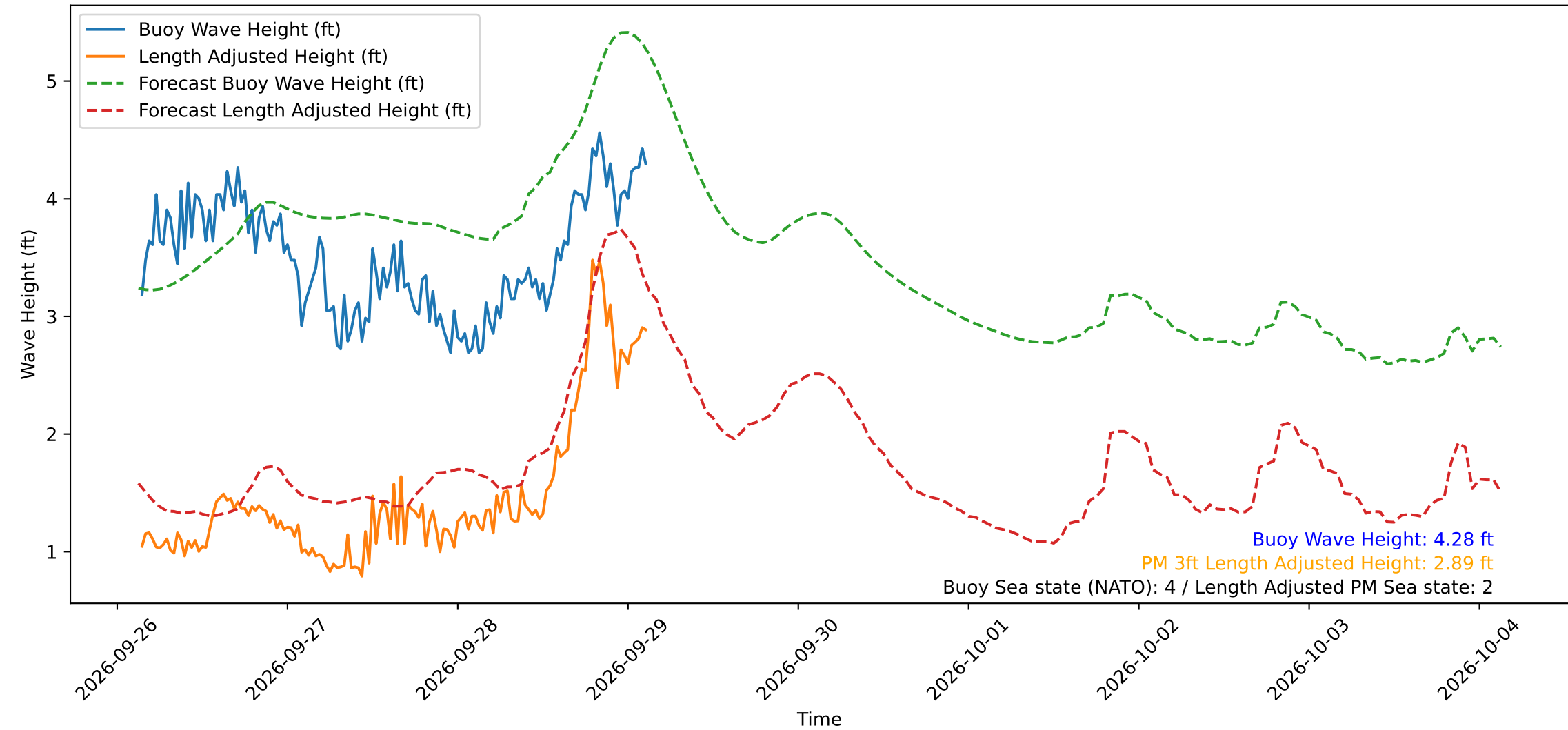
Wave Heights over Time for Green Beach at 2026-09-29 03:11:13
