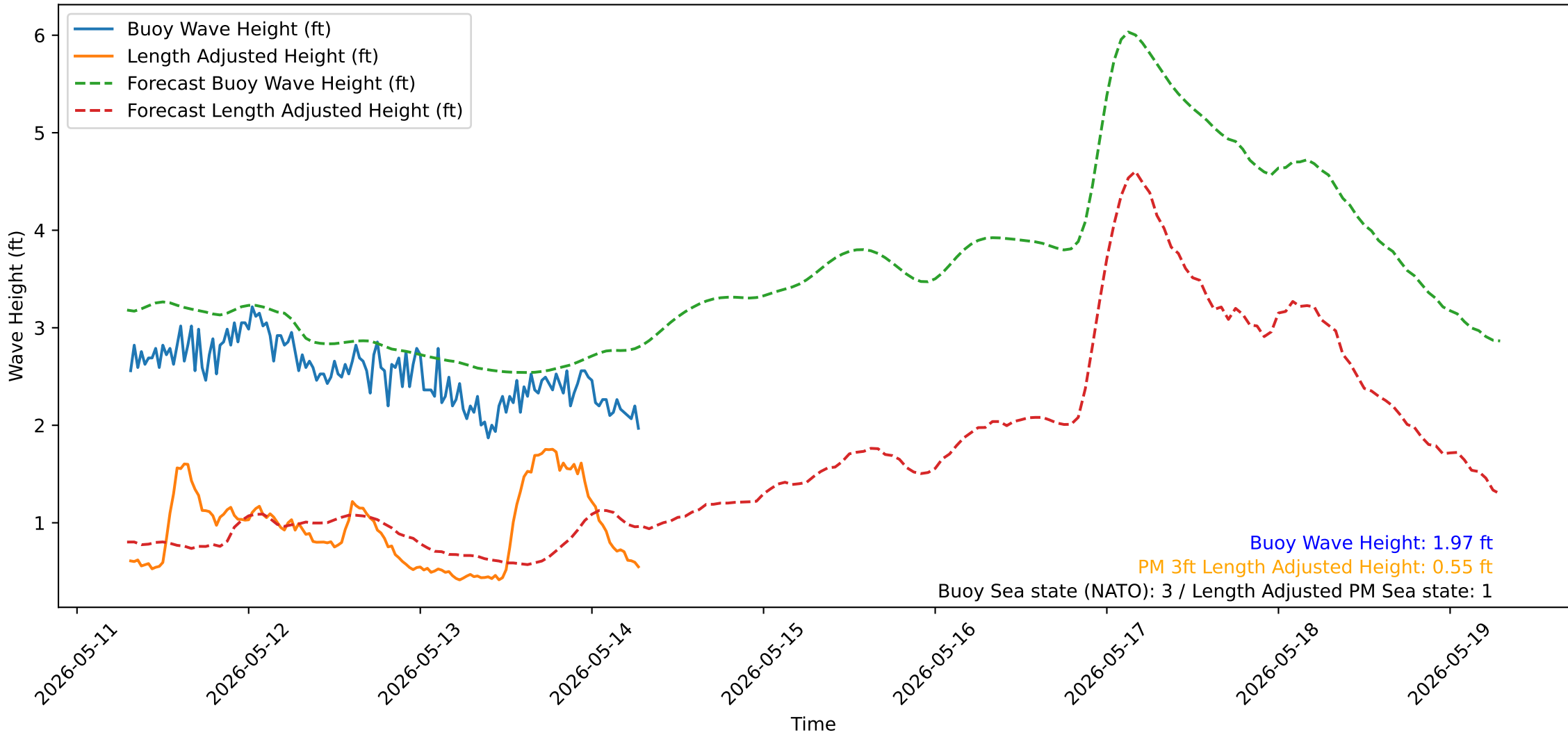
Wave Heights over Time for Red Beach at 2026-05-14 07:10:52
