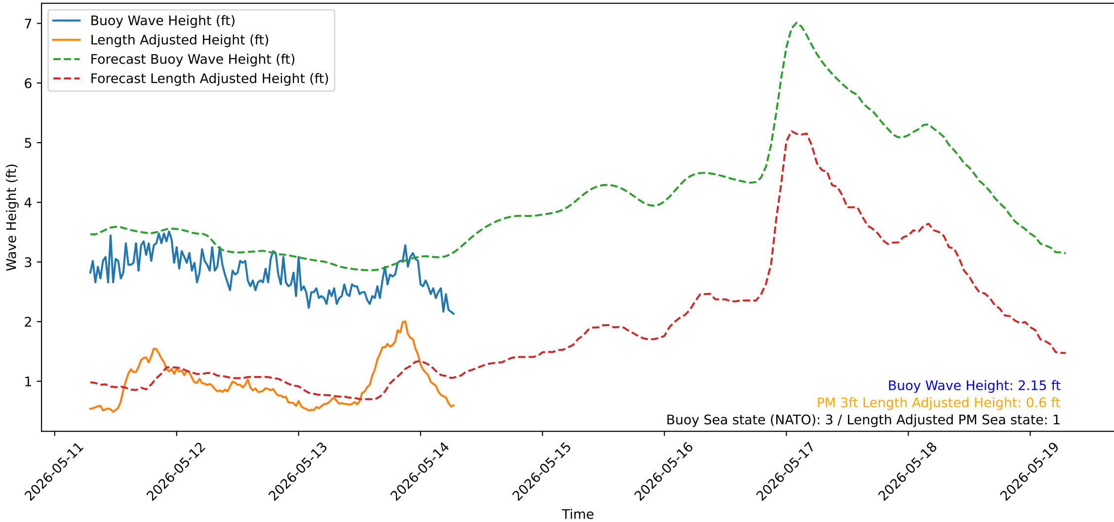
Wave Heights over Time for Green Beach at 2026-05-14 07:11:15
