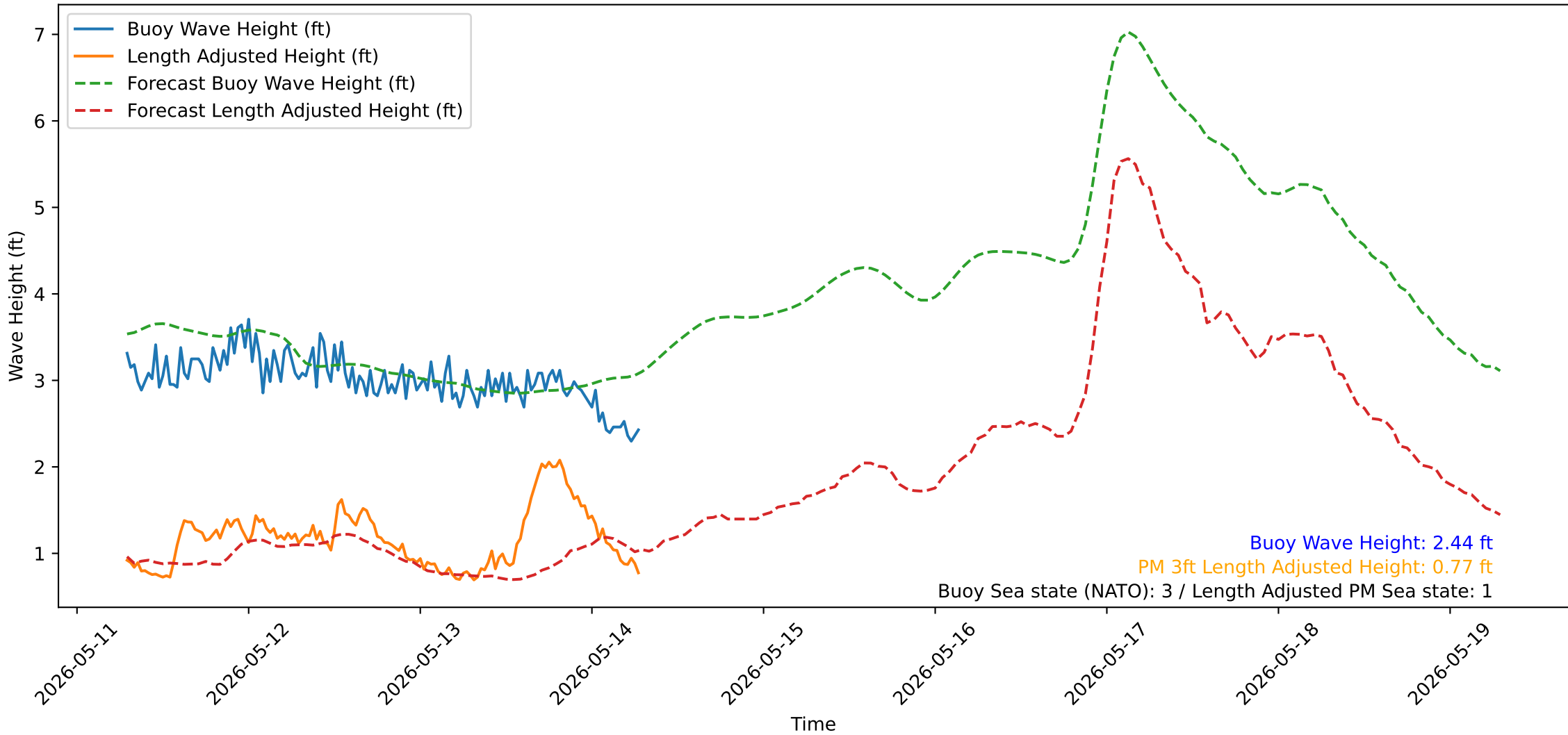
Wave Heights over Time for Oceanside Harbor at 2026-05-14 07:10:32
