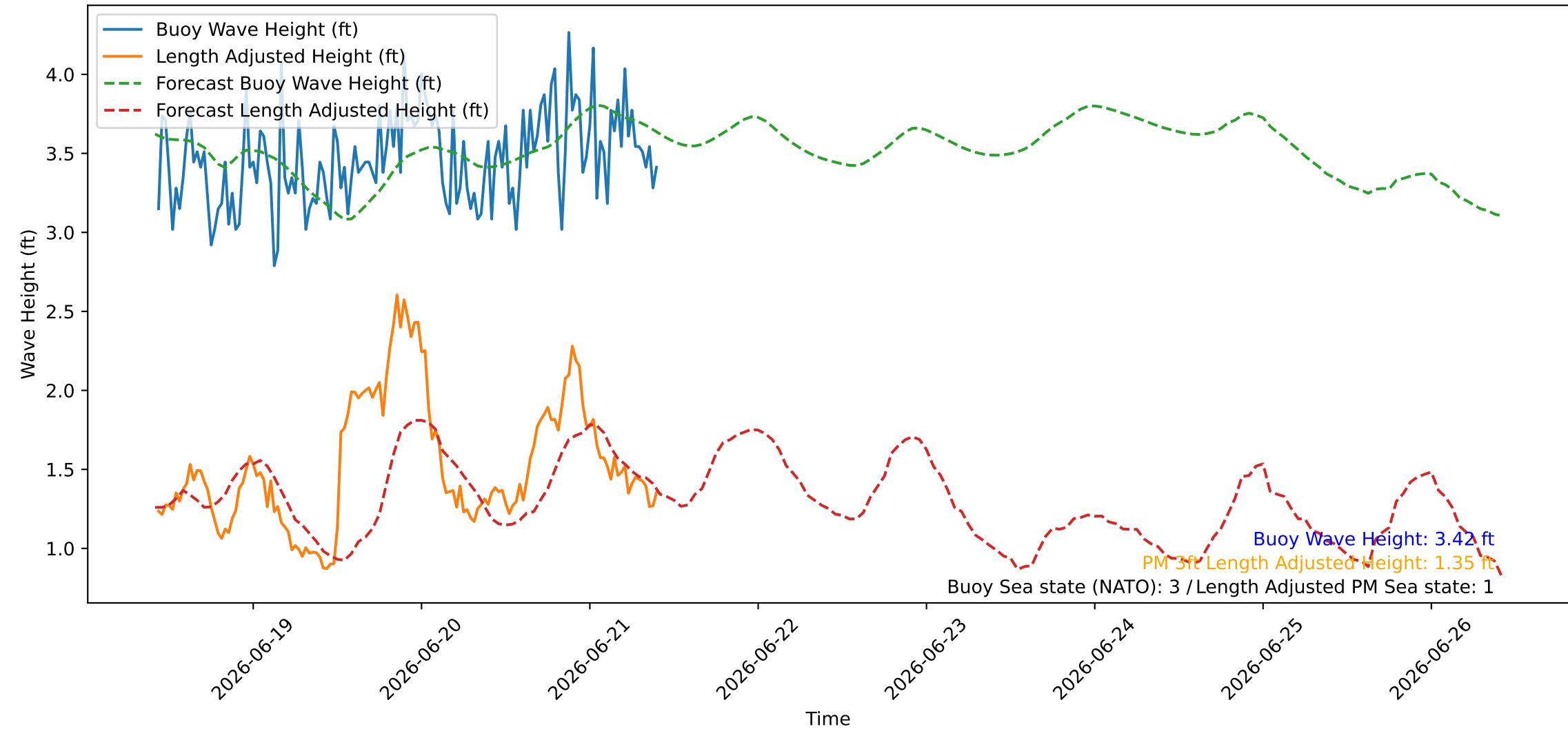
Wave Heights over Time for Oceanside Harbor at 2026-06-21 10:20:25
