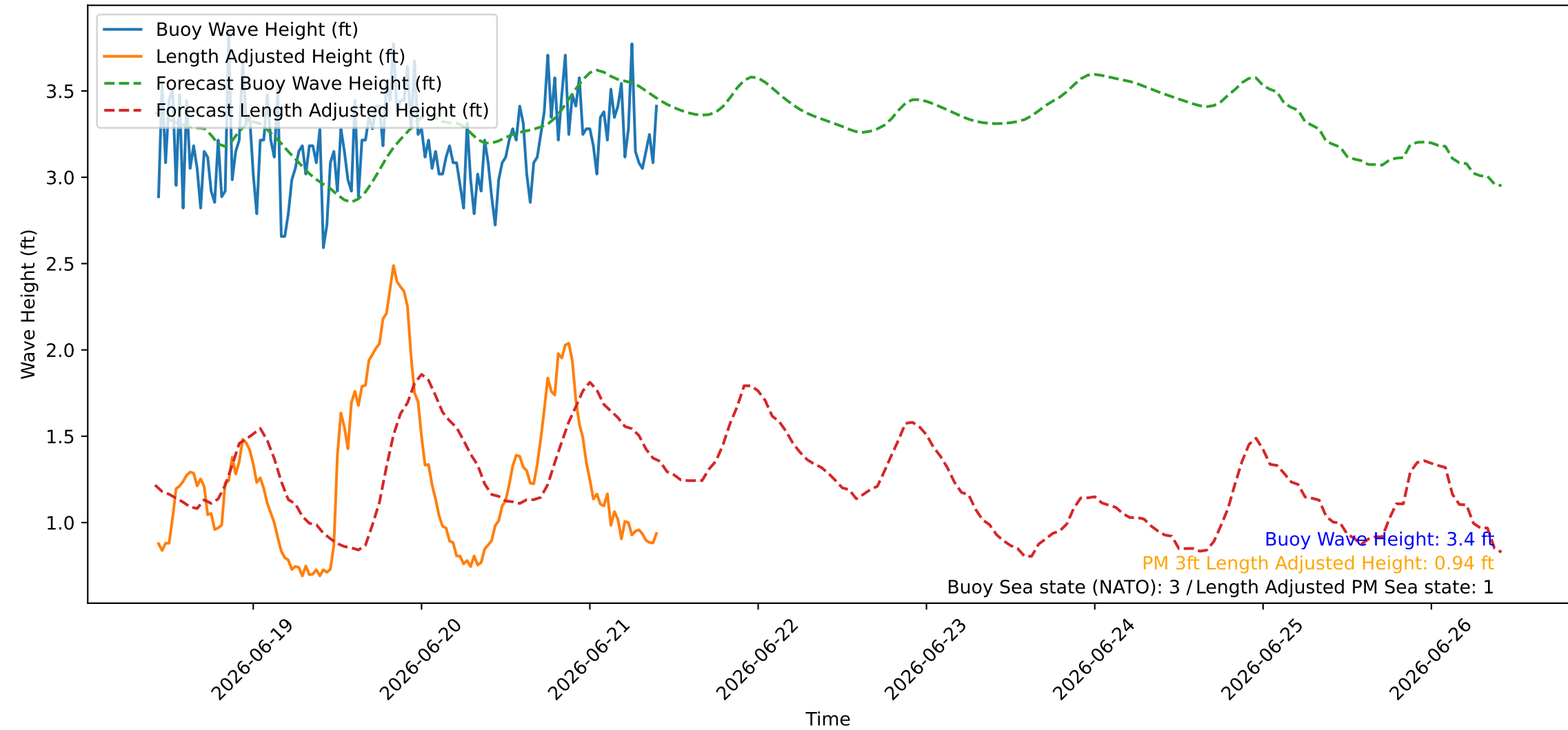
Wave Heights over Time for Red Beach at 2026-06-21 10:20:46
