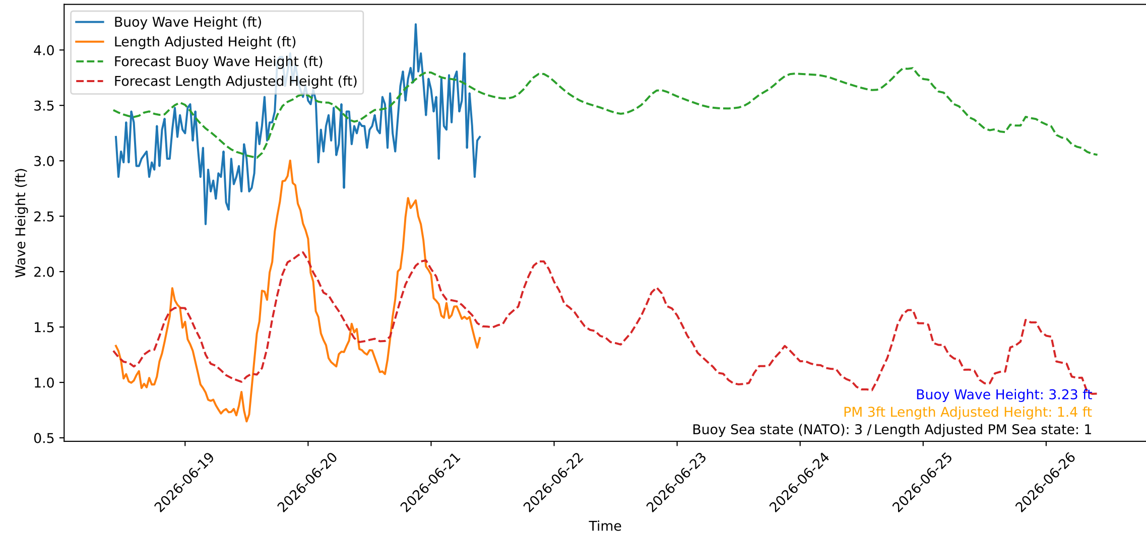
Wave Heights over Time for Green Beach at 2026-06-21 10:21:08
