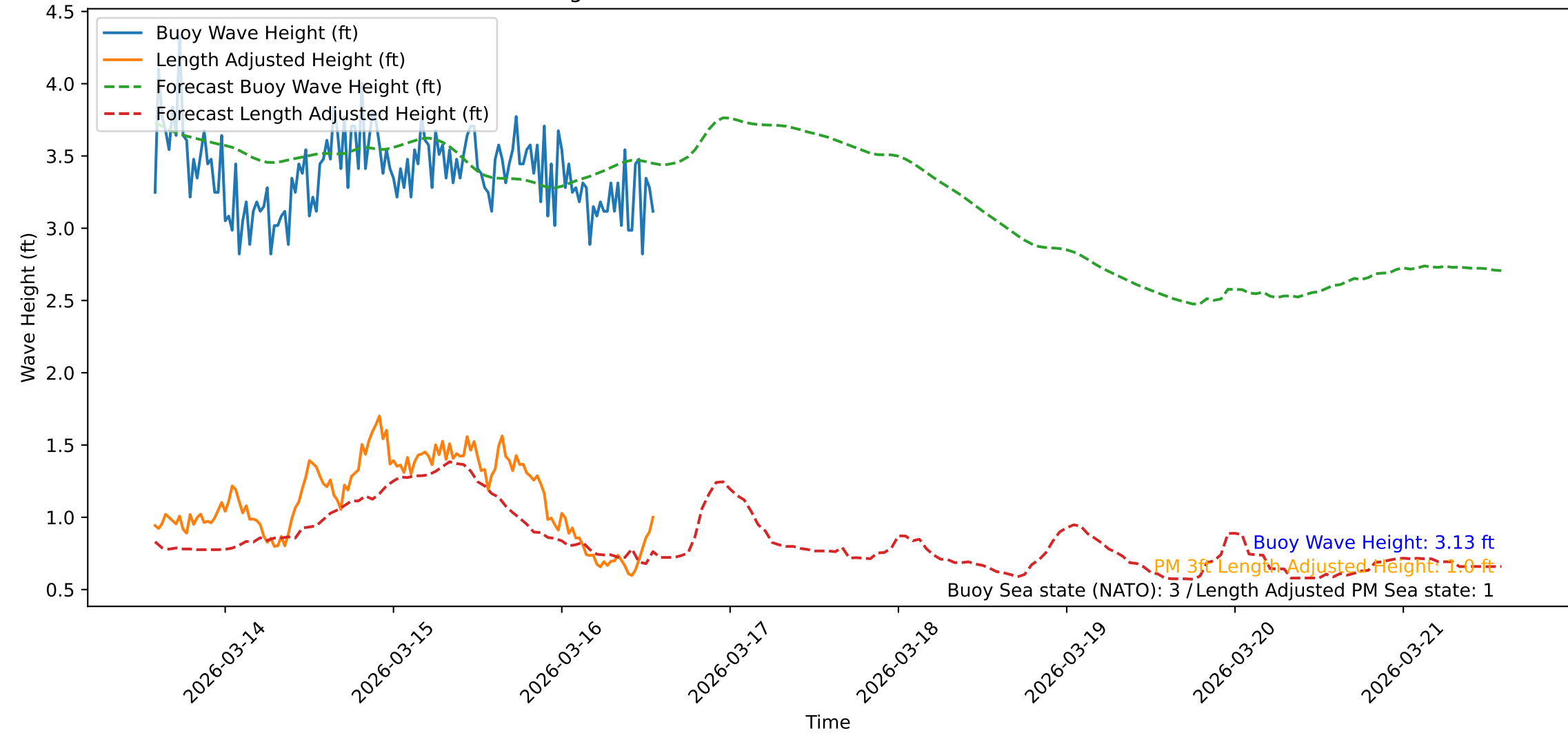
Wave Heights over Time for Green Beach at 2026-03-16 13:51:50
