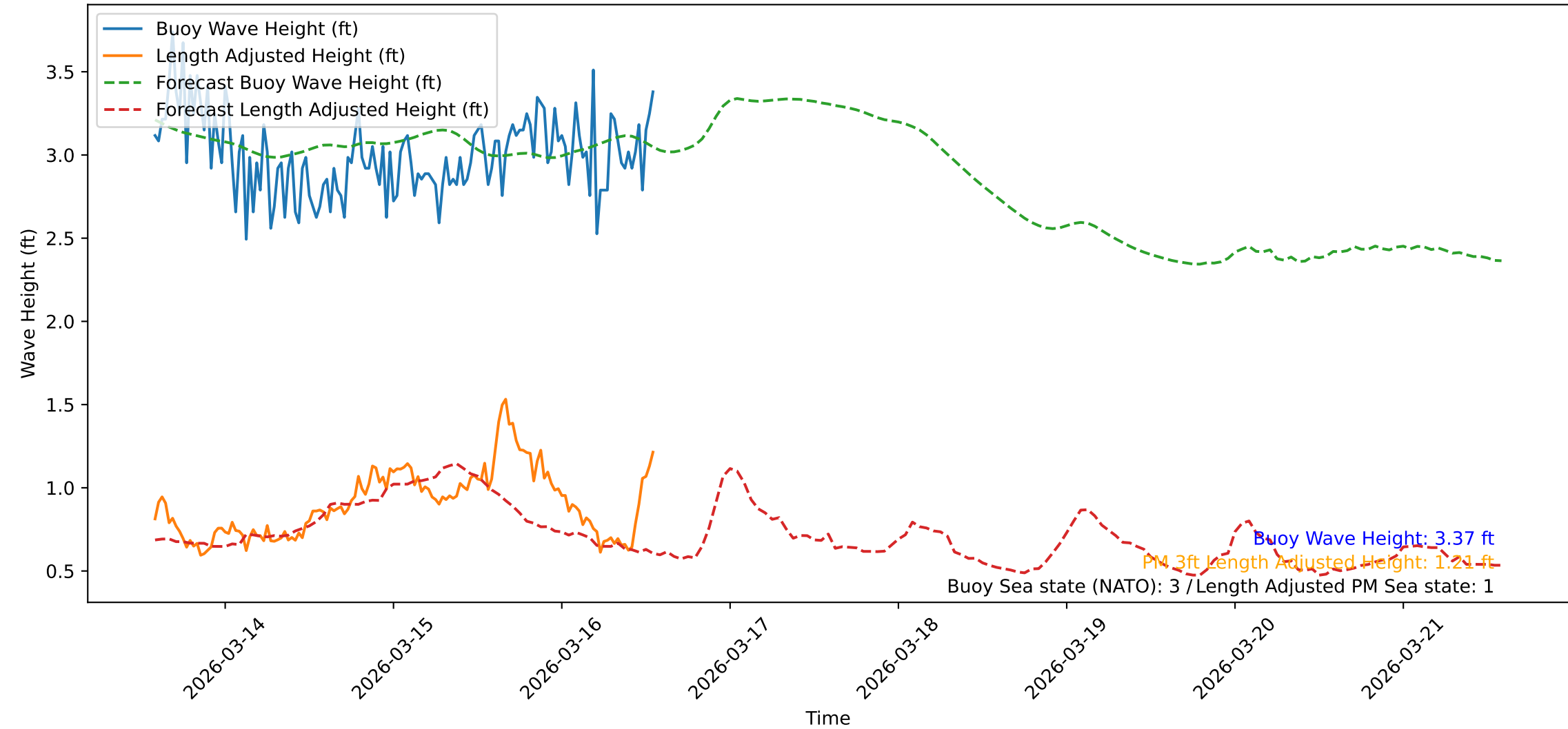
Wave Heights over Time for Red Beach at 2026-03-16 13:51:14
