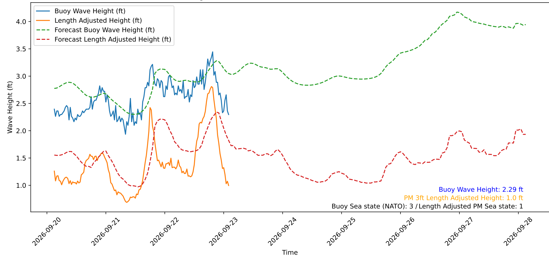
Wave Heights over Time for Green Beach at 2026-09-23 02:41:11
