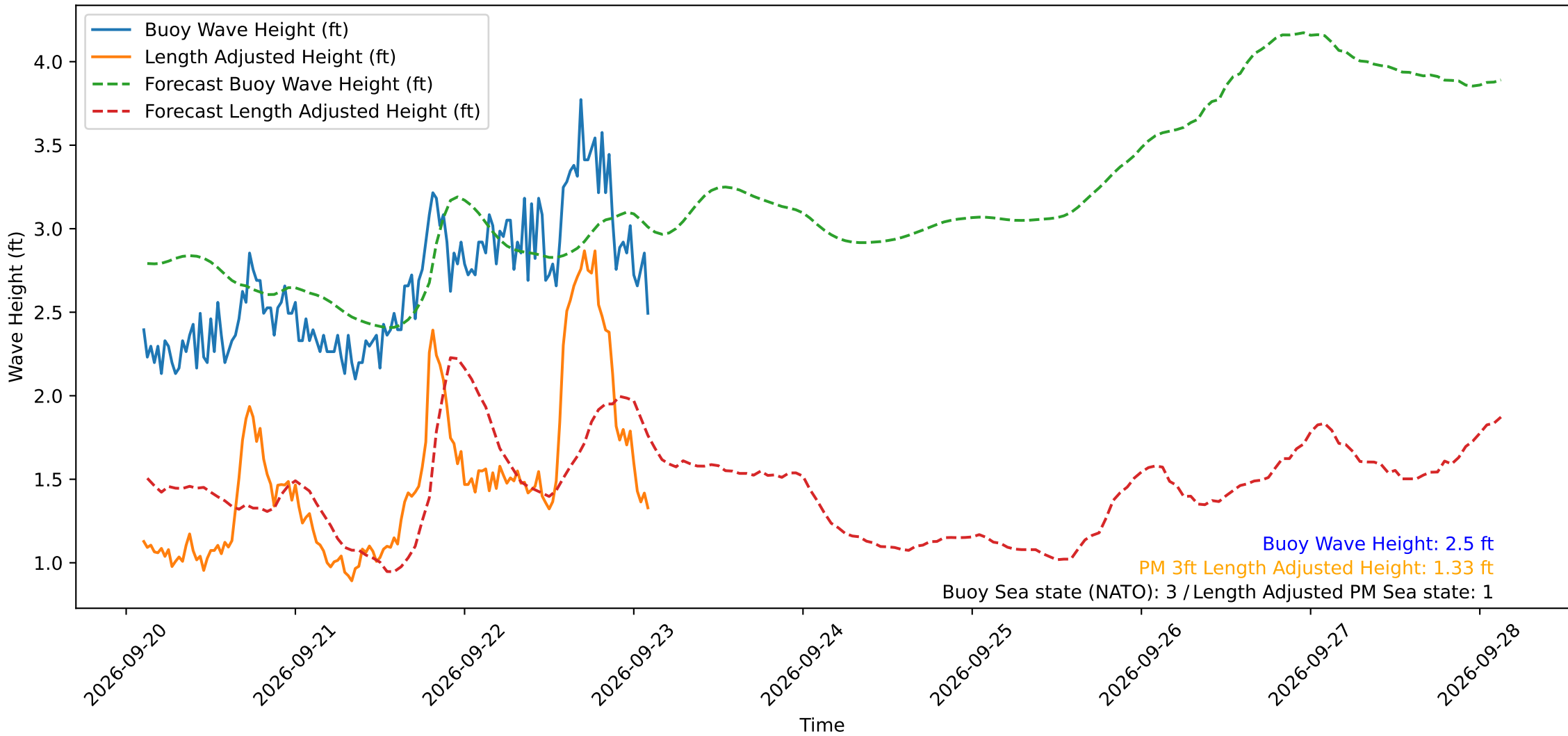
Wave Heights over Time for Oceanside Harbor at 2026-09-23 02:40:29
