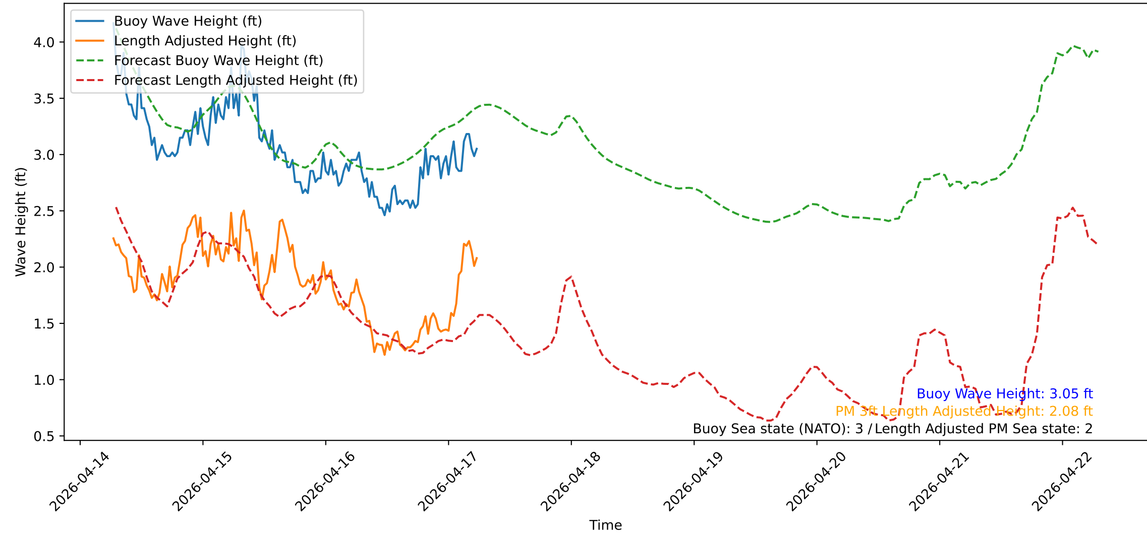
Wave Heights over Time for Green Beach at 2026-04-17 06:31:15
