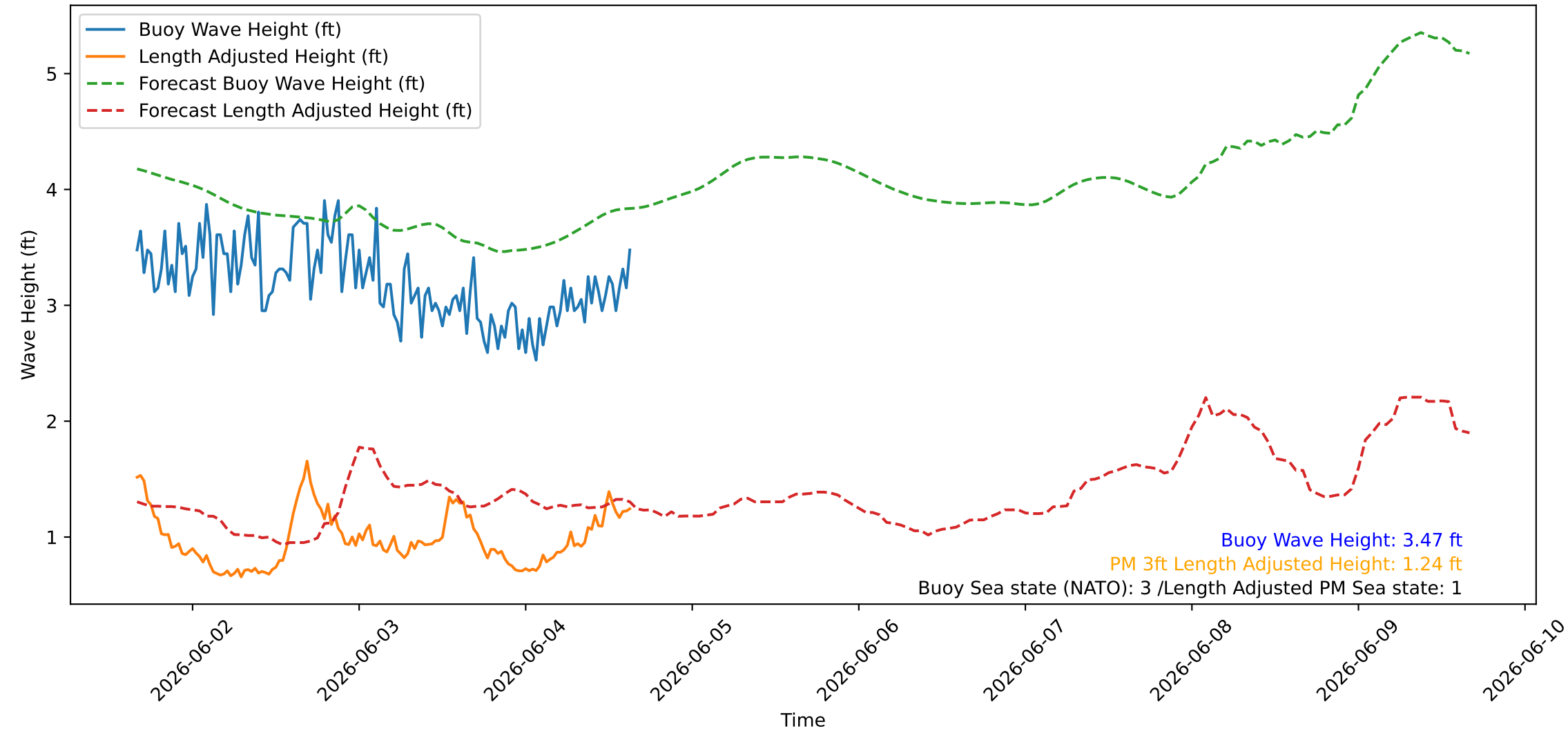
Wave Heights over Time for Red Beach at 2026-06-04 15:50:47
