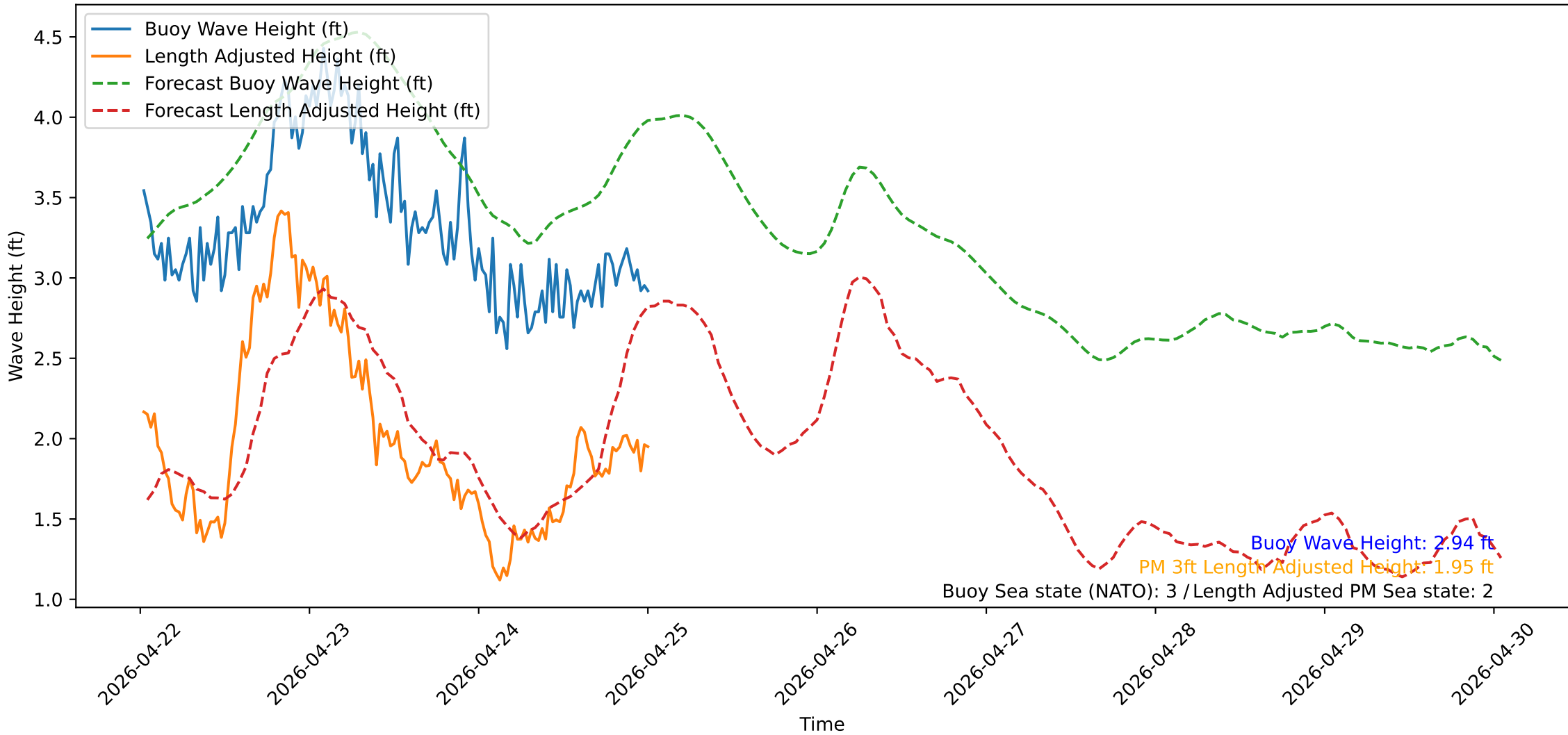
Wave Heights over Time for Oceanside Harbor at 2026-04-25 00:30:31
