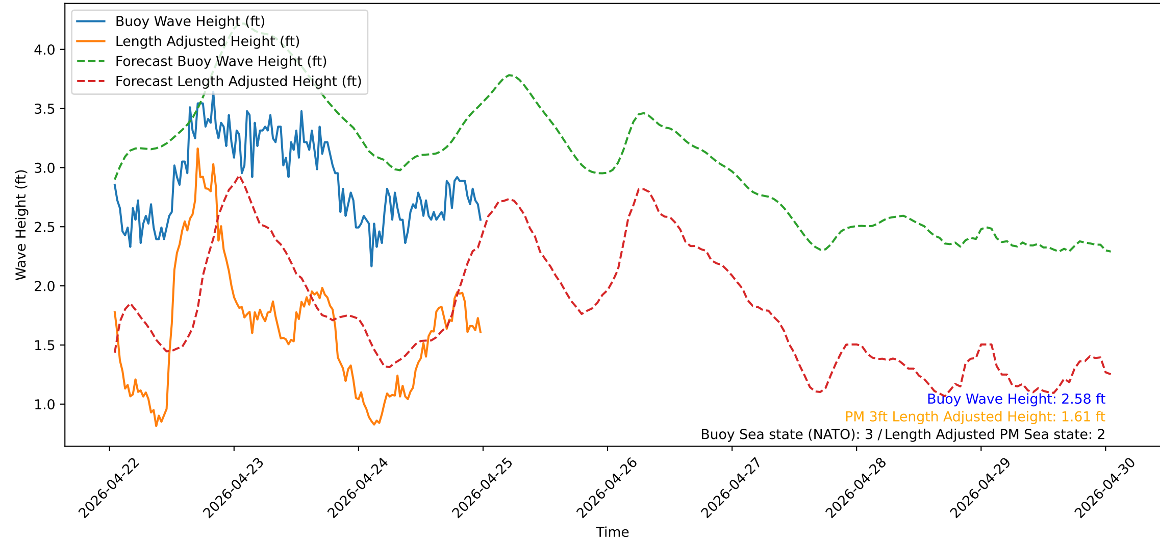
Wave Heights over Time for Red Beach at 2026-04-25 00:30:50
