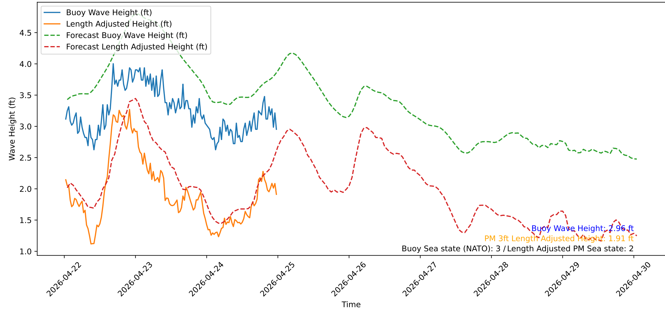
Wave Heights over Time for Green Beach at 2026-04-25 00:31:12
