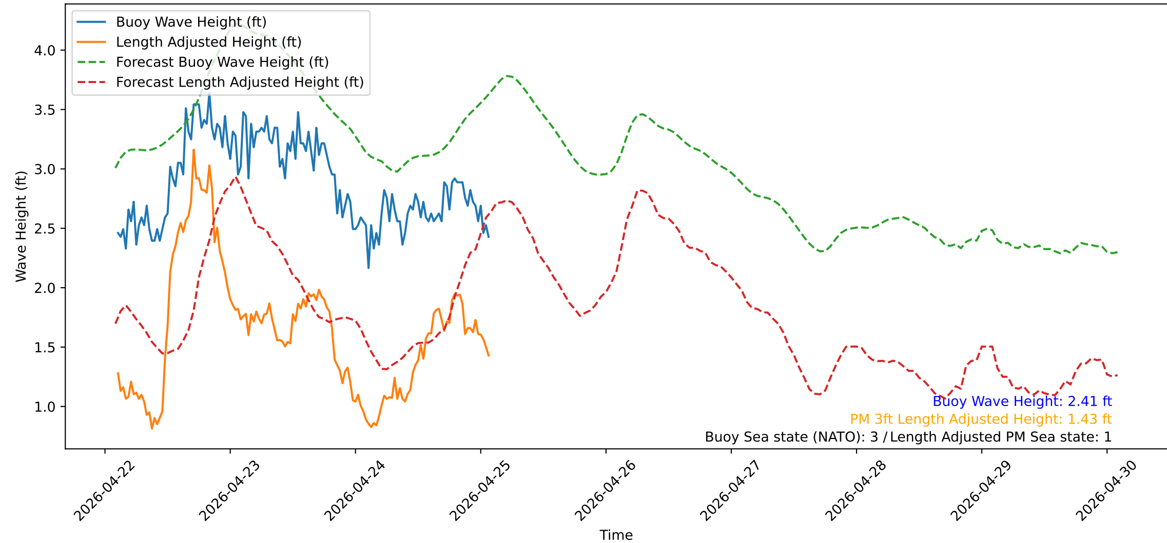
Wave Heights over Time for Red Beach at 2026-04-25 02:10:51
