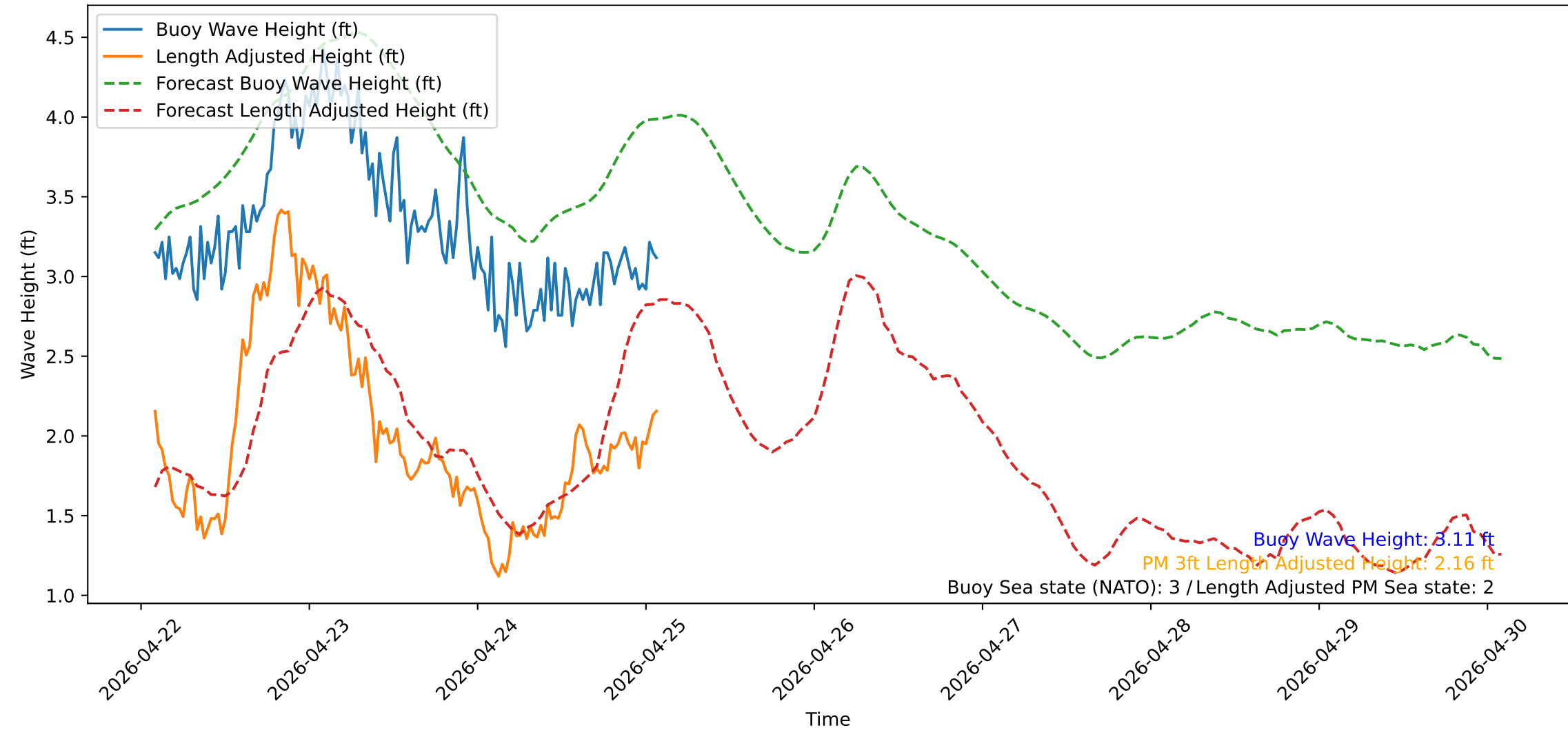
Wave Heights over Time for Oceanside Harbor at 2026-04-25 02:10:32
