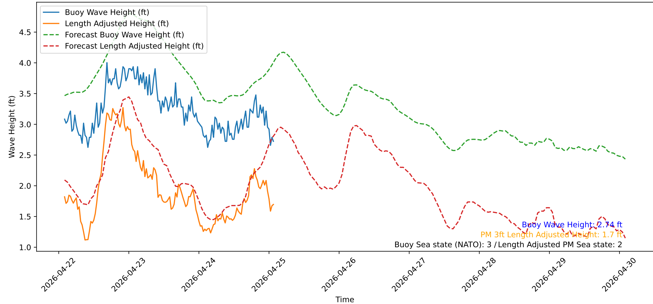
Wave Heights over Time for Green Beach at 2026-04-25 02:11:13
