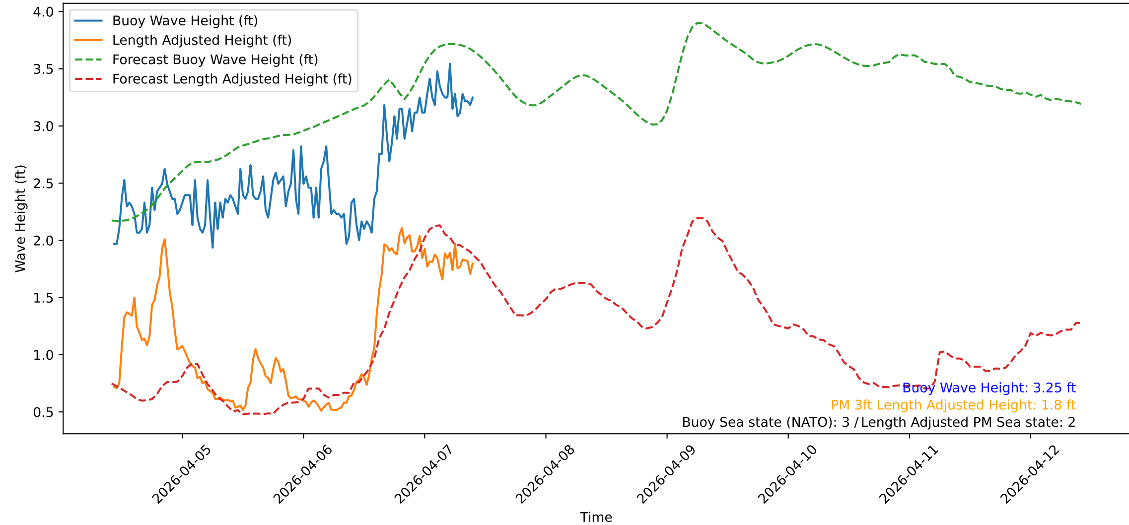
Wave Heights over Time for Red Beach at 2026-04-07 10:20:47
