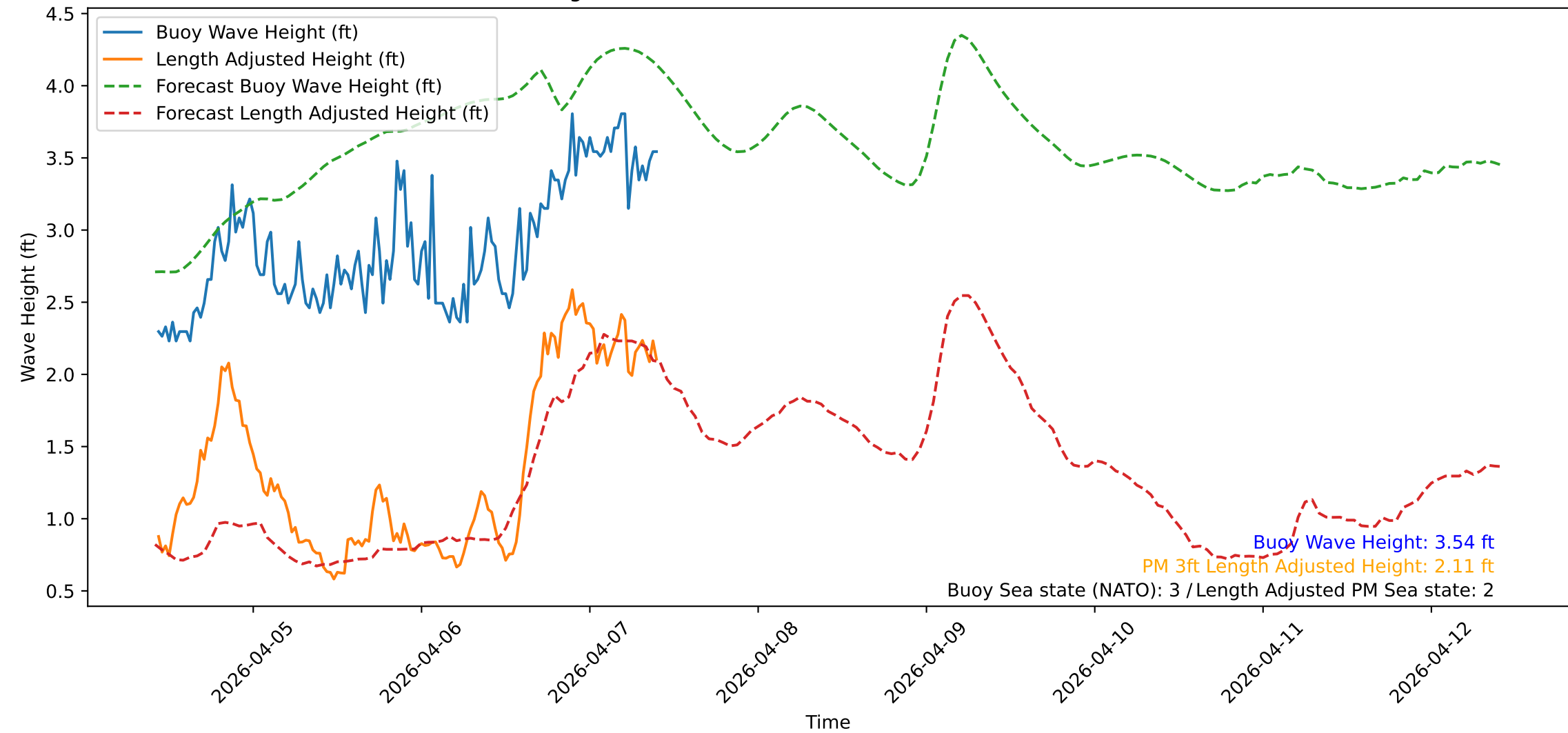
Wave Heights over Time for Green Beach at 2026-04-07 10:21:10
