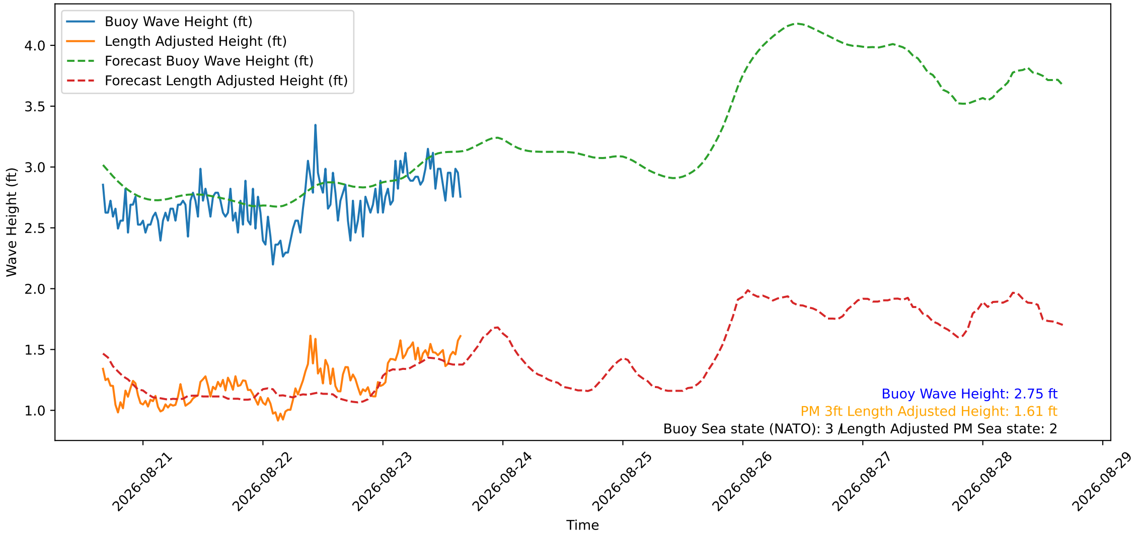
Wave Heights over Time for Oceanside Harbor at 2026-08-23 16:10:29
