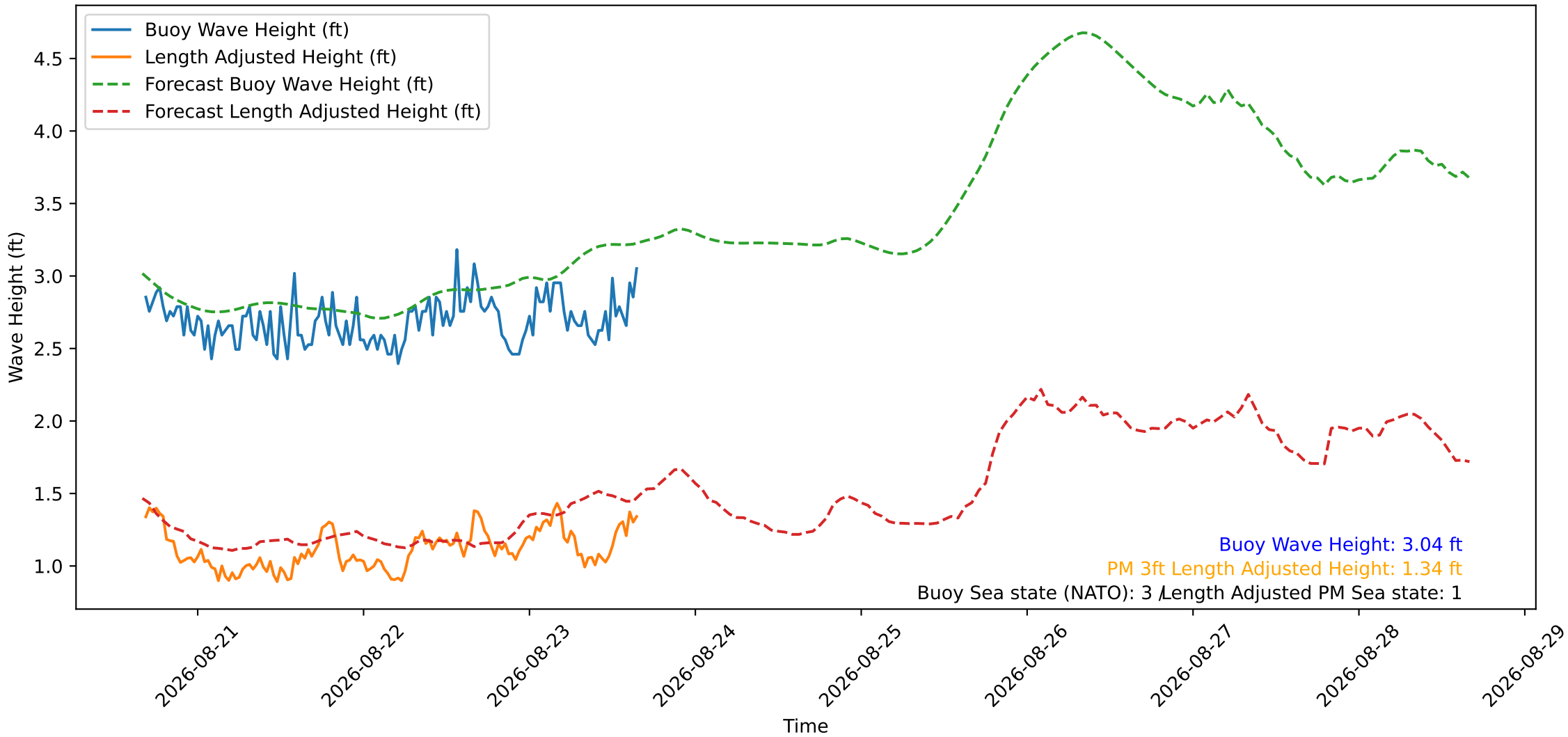
Wave Heights over Time for Green Beach at 2026-08-23 16:11:11
