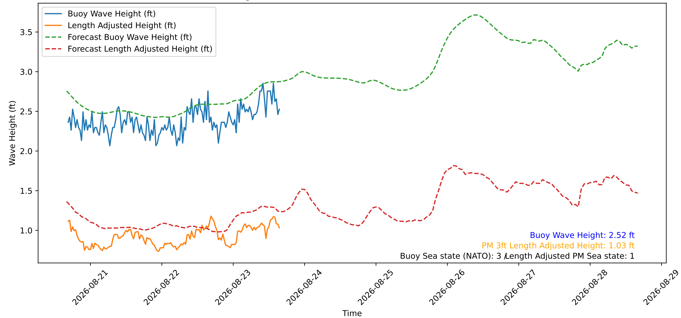
Wave Heights over Time for Red Beach at 2026-08-23 16:10:48
