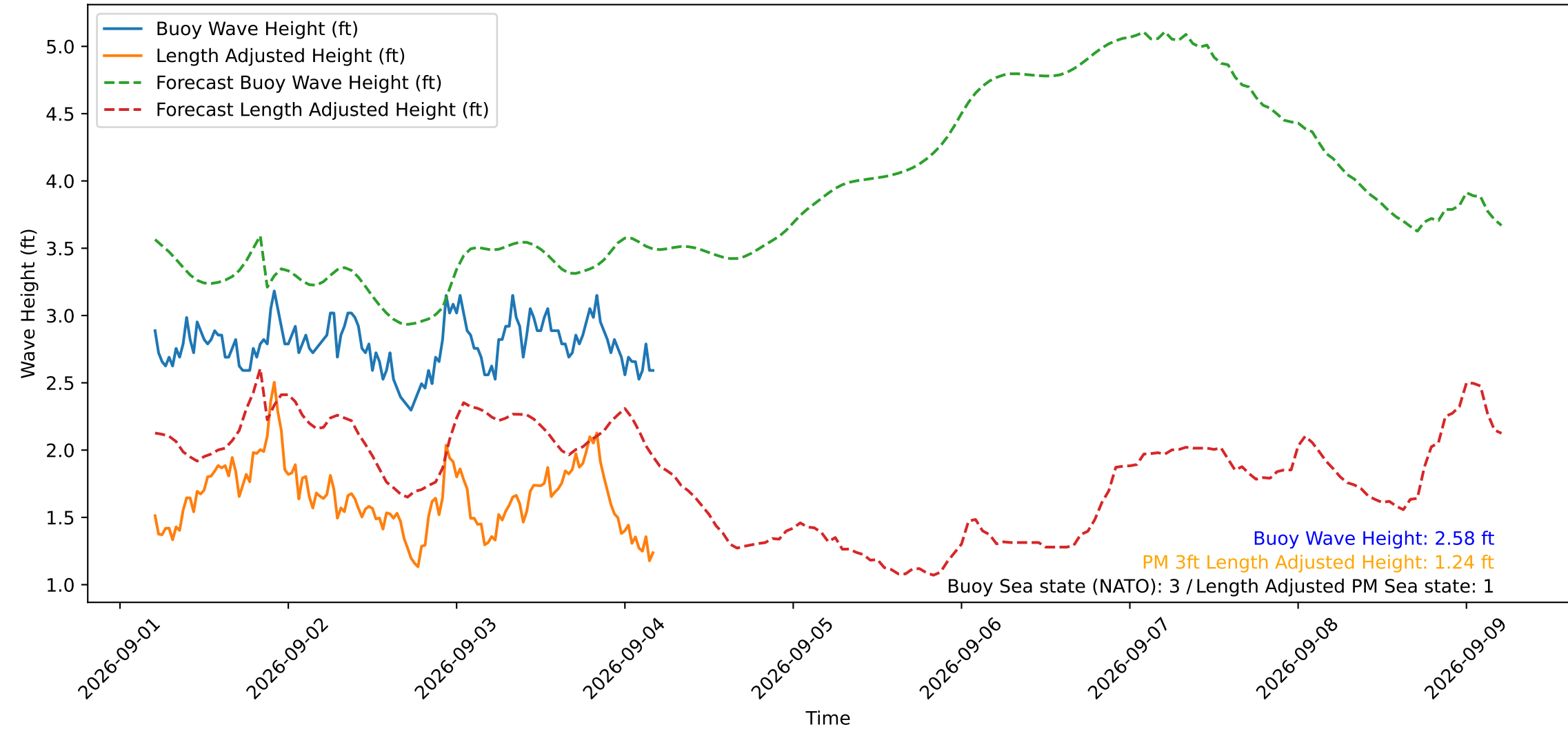
Wave Heights over Time for Red Beach at 2026-09-04 04:40:49
