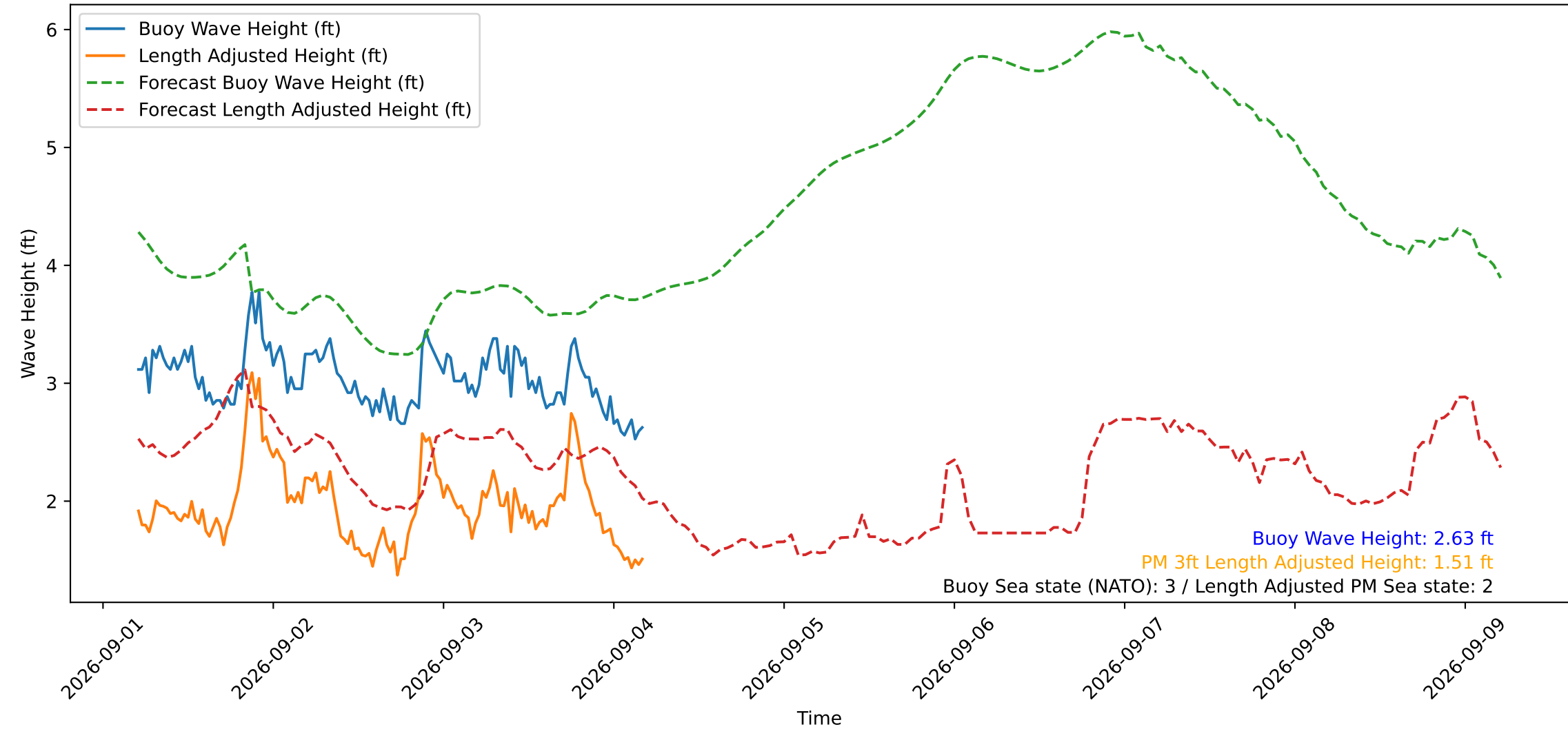
Wave Heights over Time for Green Beach at 2026-09-04 04:41:11
