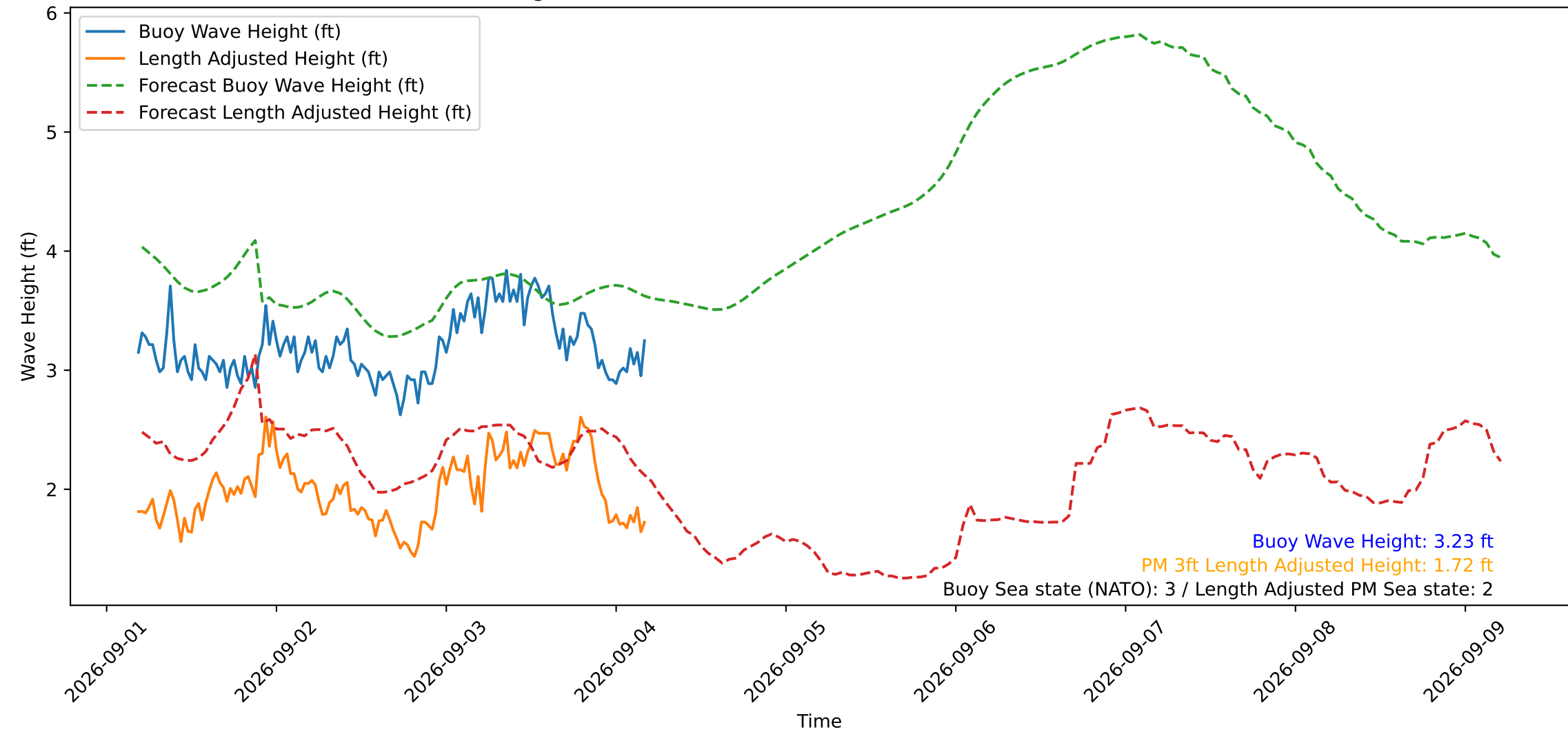
Wave Heights over Time for Oceanside Harbor at 2026-09-04 04:40:29
