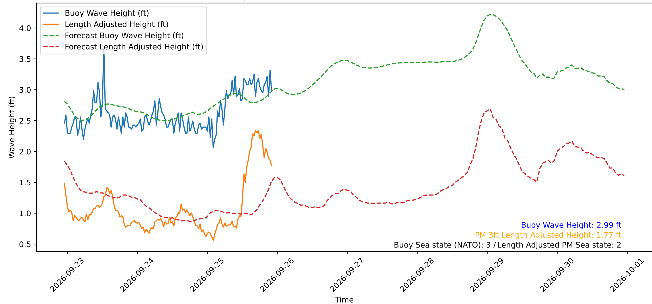
Wave Heights over Time for Red Beach at 2026-09-25 22:50:51
