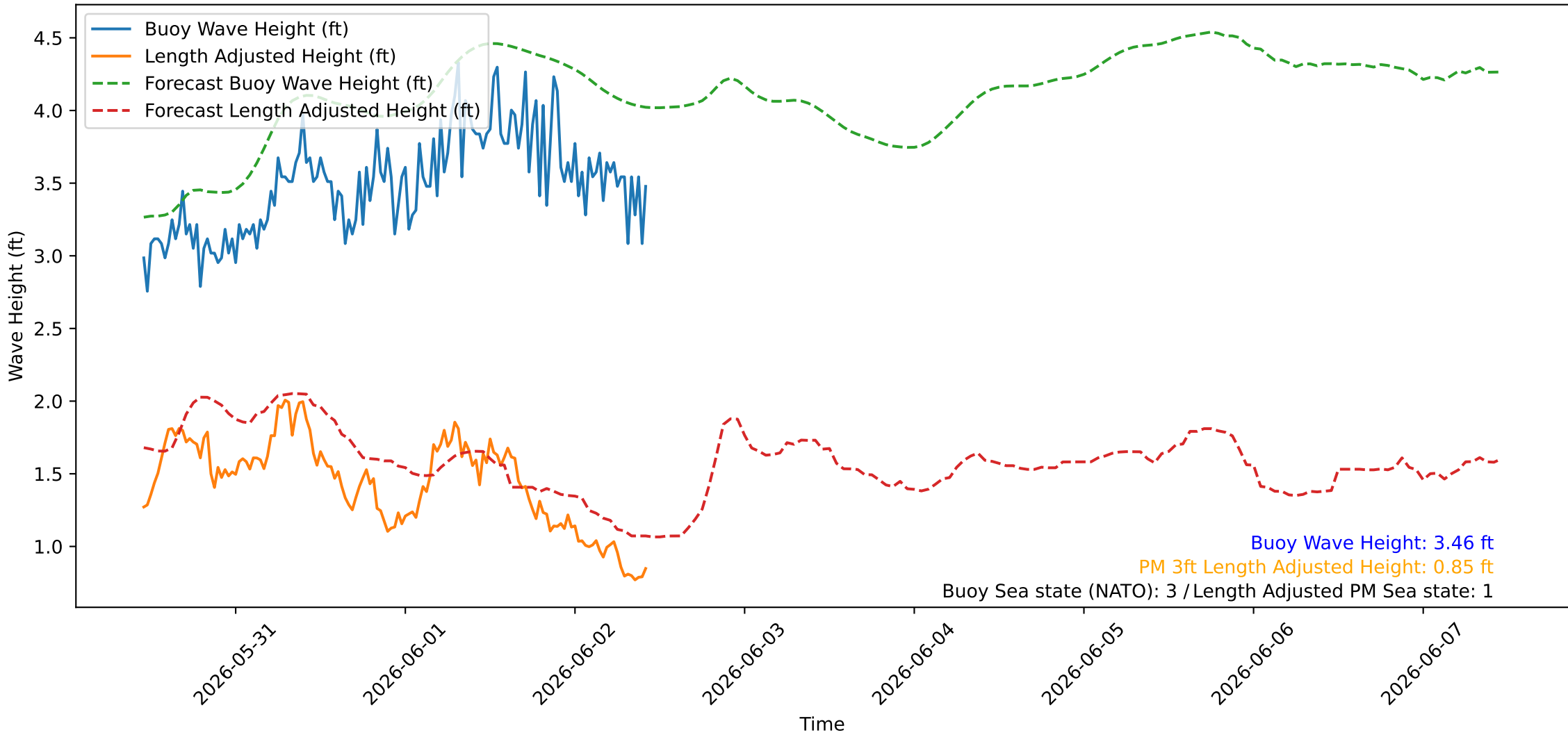
Wave Heights over Time for Green Beach at 2026-06-02 10:51:08
