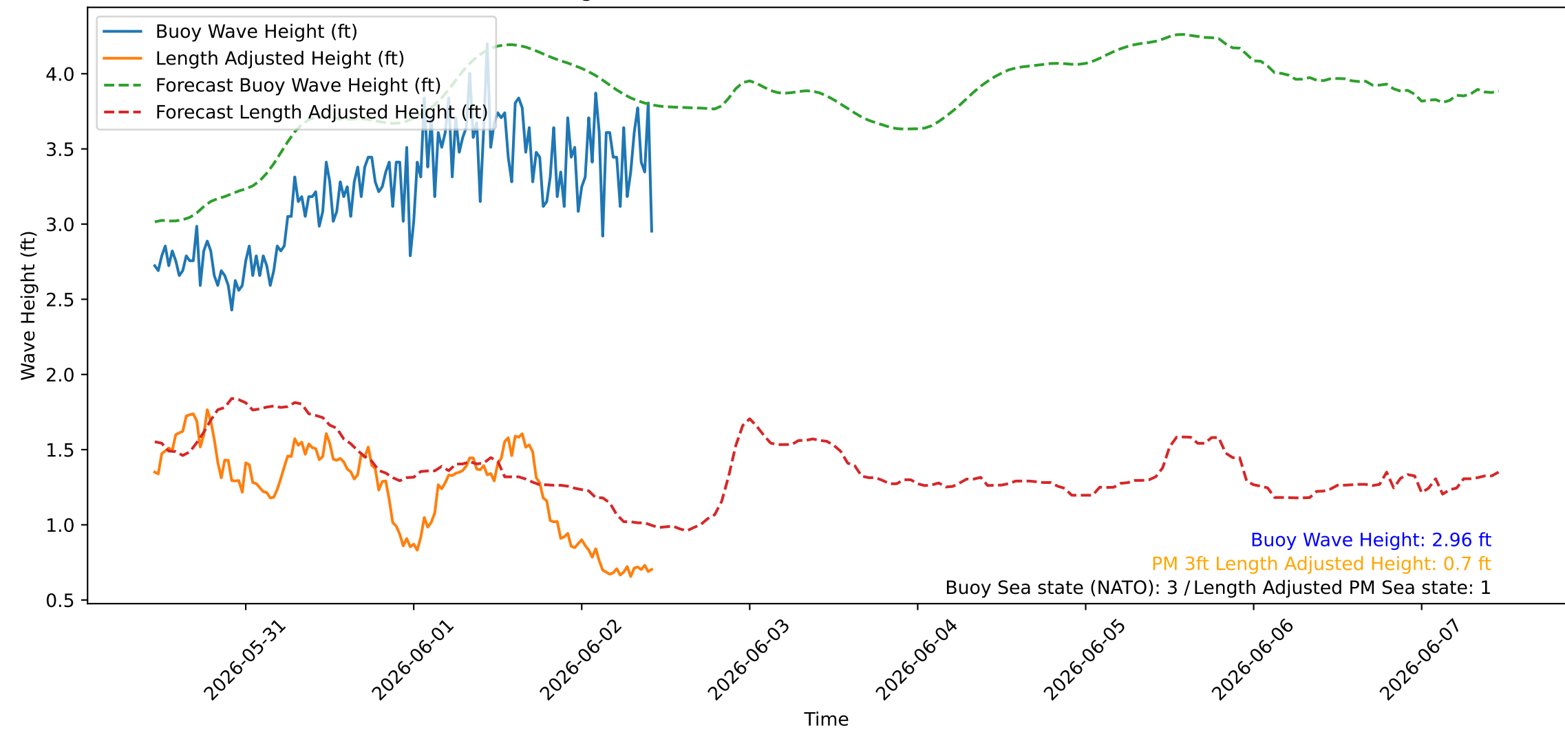
Wave Heights over Time for Red Beach at 2026-06-02 10:50:46
