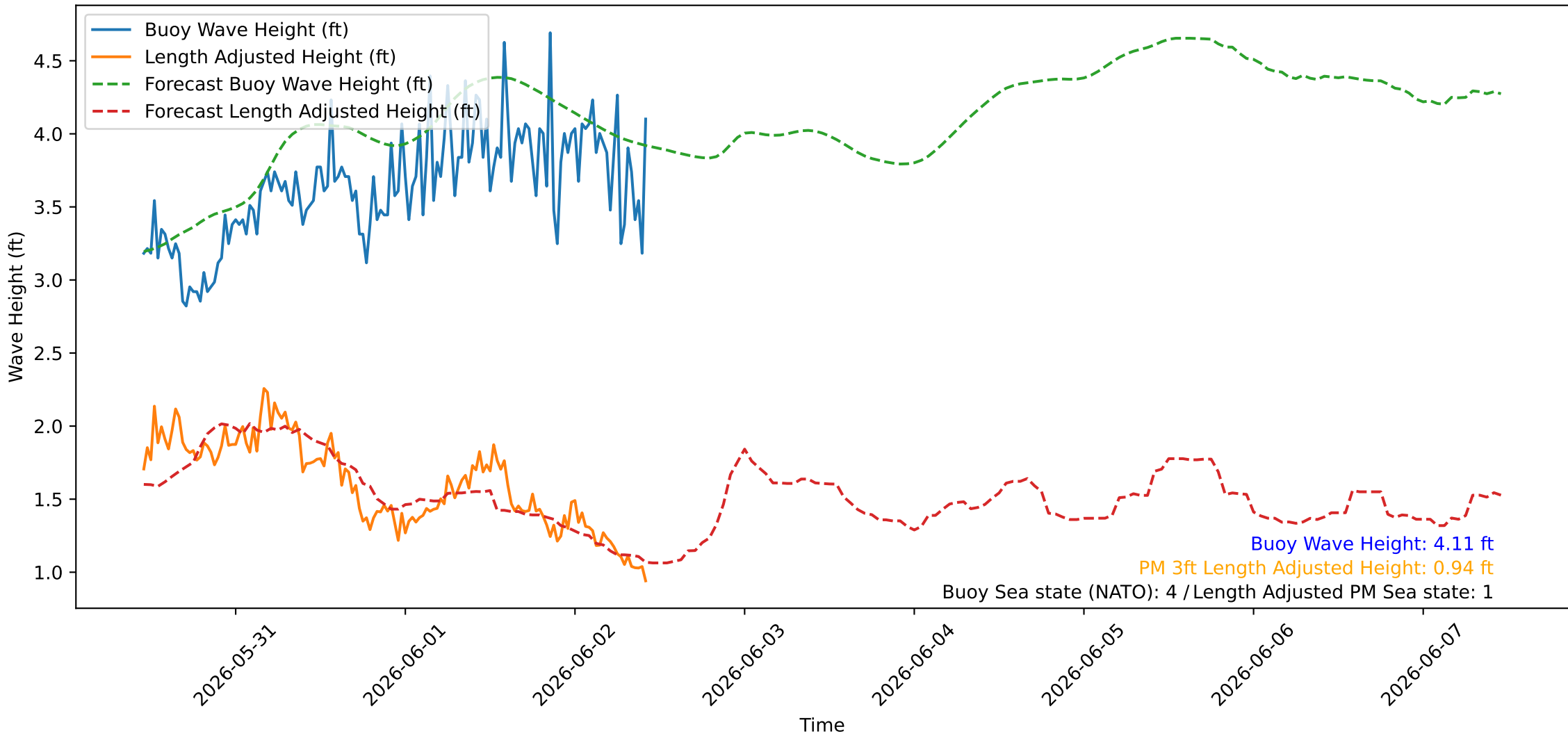
Wave Heights over Time for Oceanside Harbor at 2026-06-02 10:50:26
