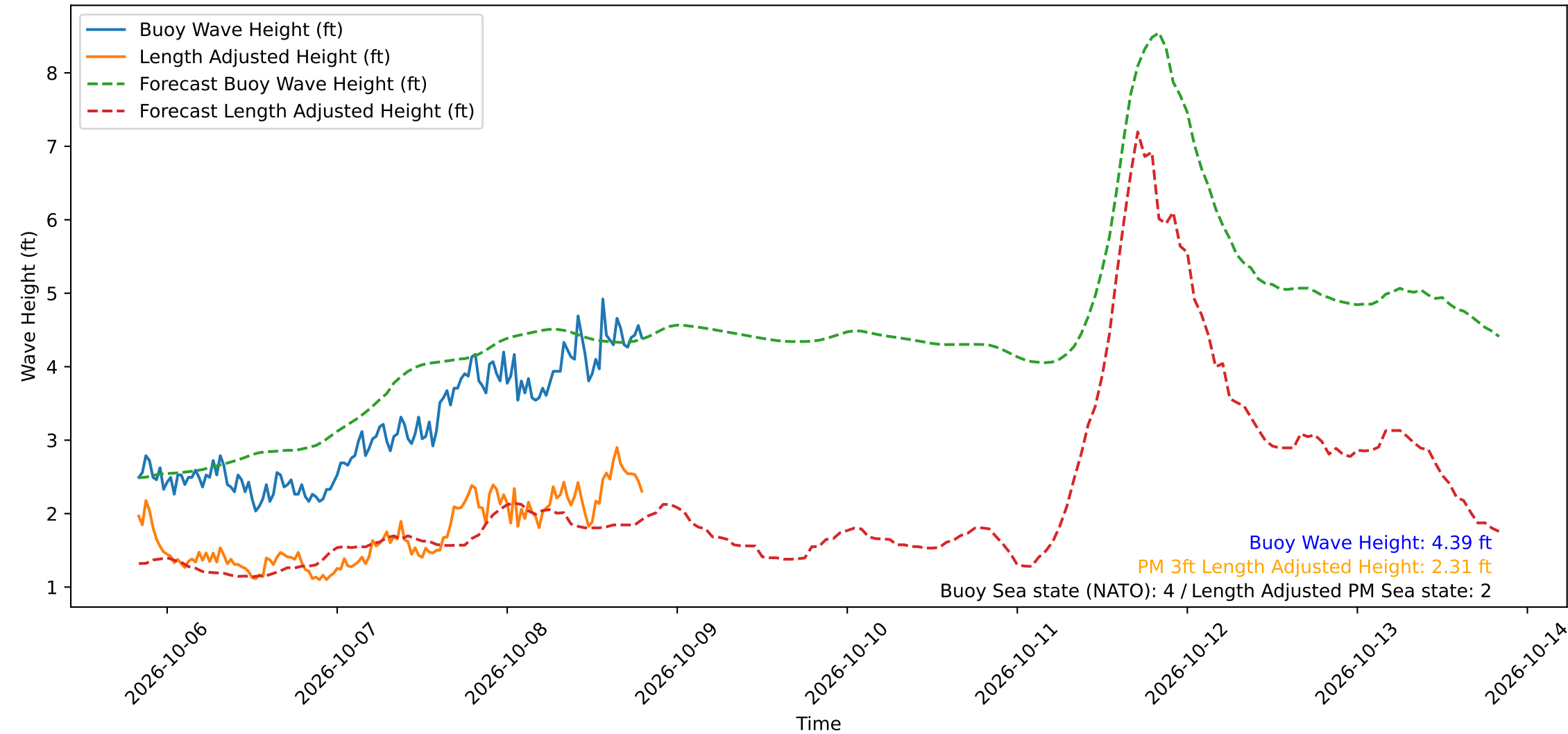
Wave Heights over Time for Oceanside Harbor at 2026-10-08 20:10:29
