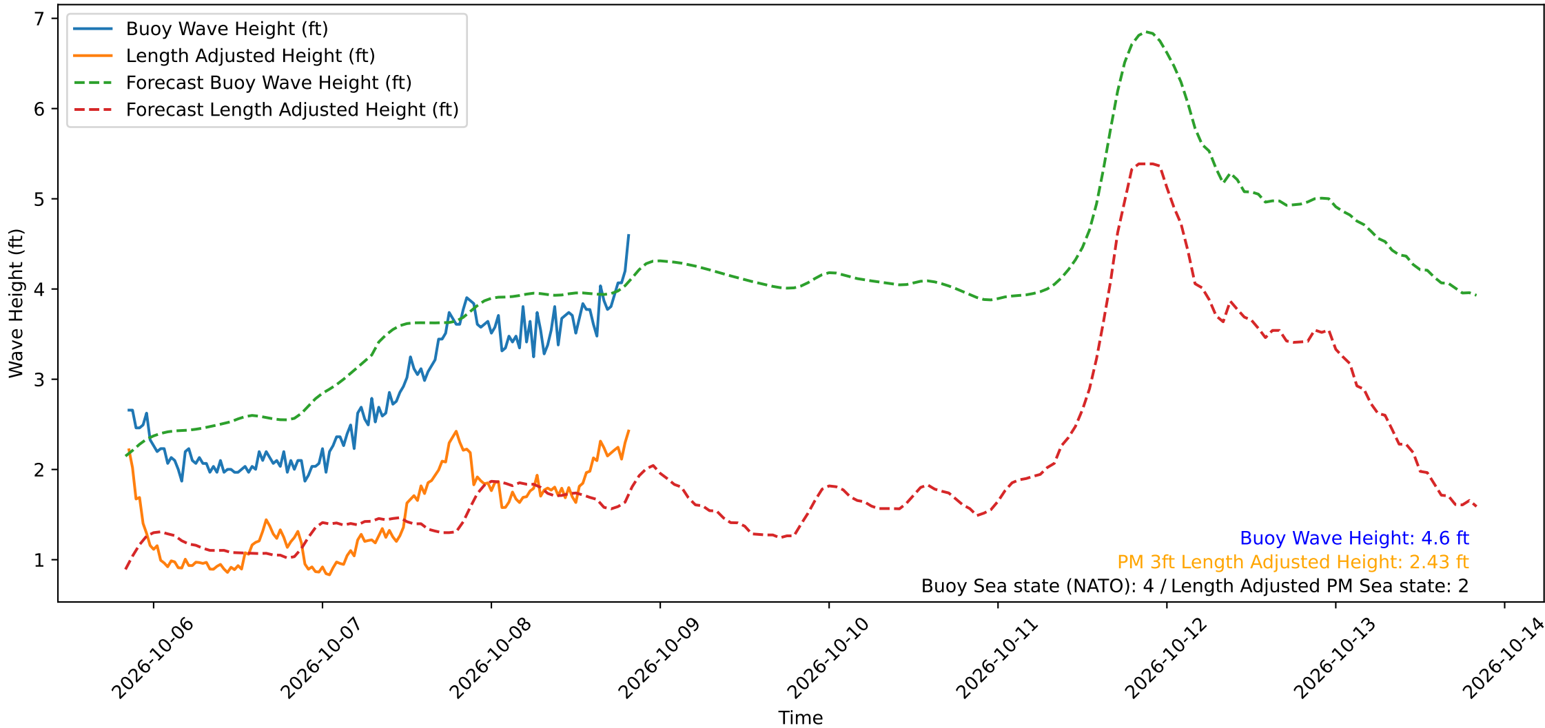
Wave Heights over Time for Red Beach at 2026-10-08 20:10:49
