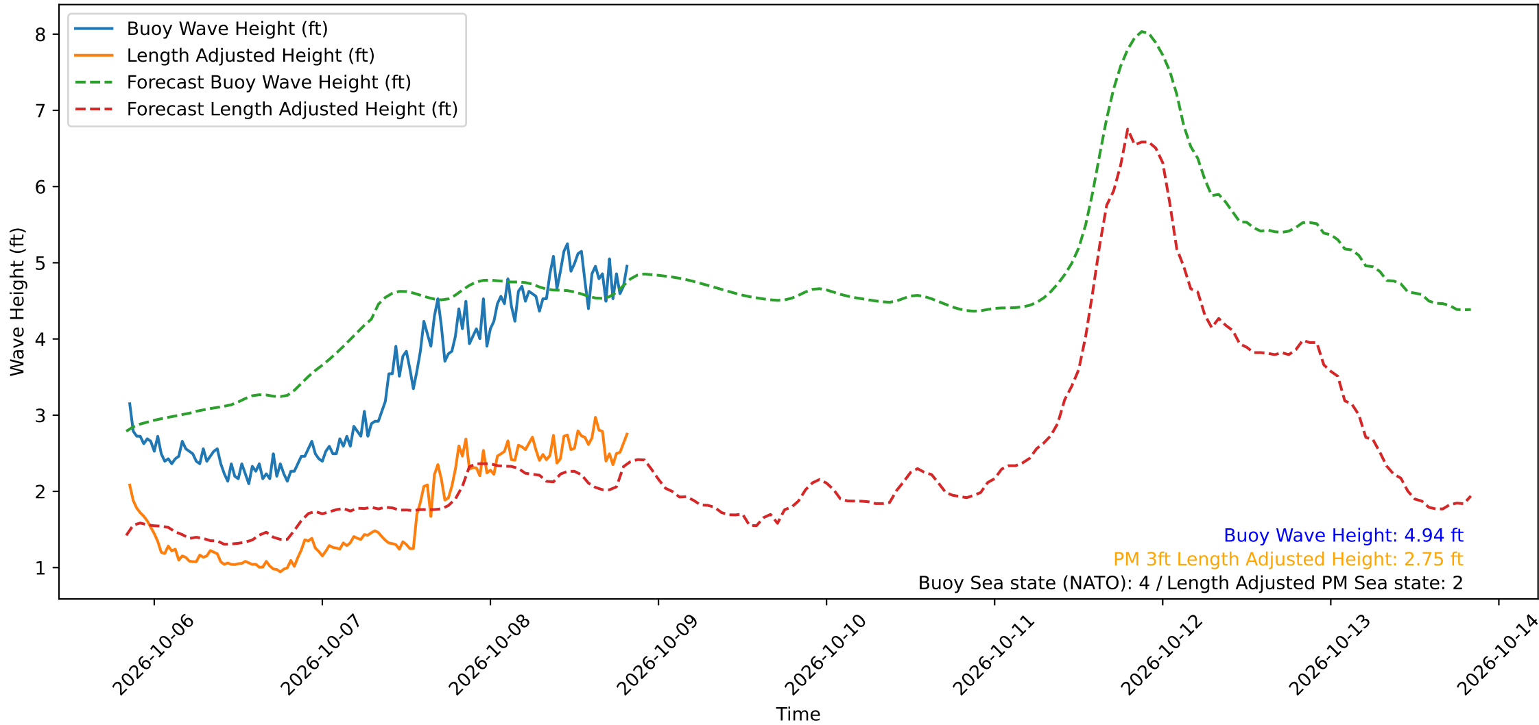
Wave Heights over Time for Green Beach at 2026-10-08 20:11:12
