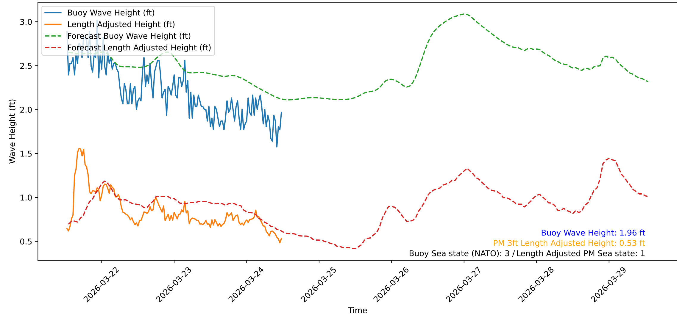
Wave Heights over Time for Oceanside Harbor at 2026-03-24 12:30:32
