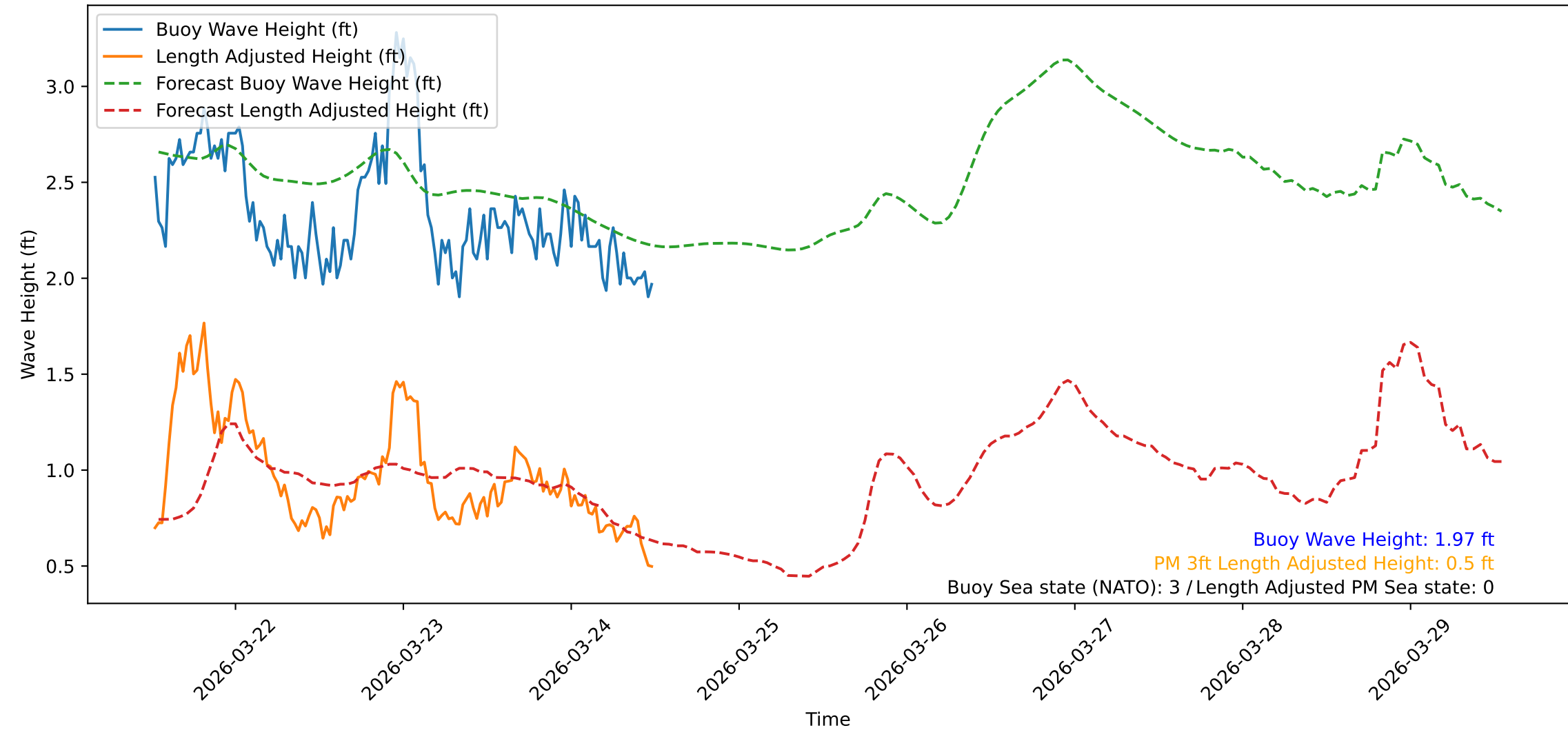
Wave Heights over Time for Green Beach at 2026-03-24 12:31:10
