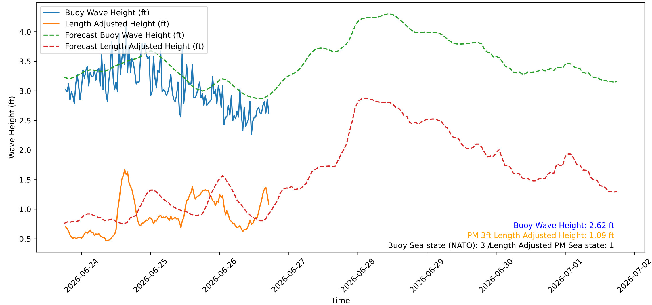
Wave Heights over Time for Red Beach at 2026-06-26 18:10:45
