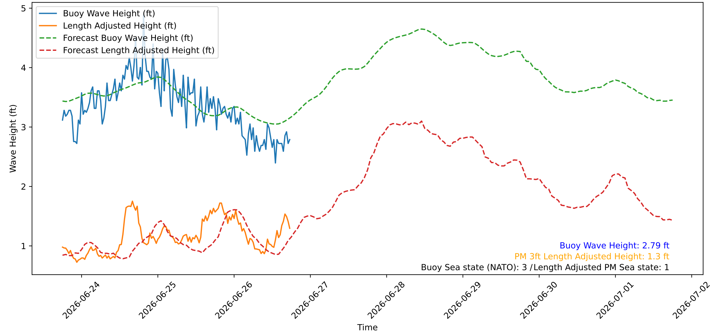
Wave Heights over Time for Oceanside Harbor at 2026-06-26 18:10:26
