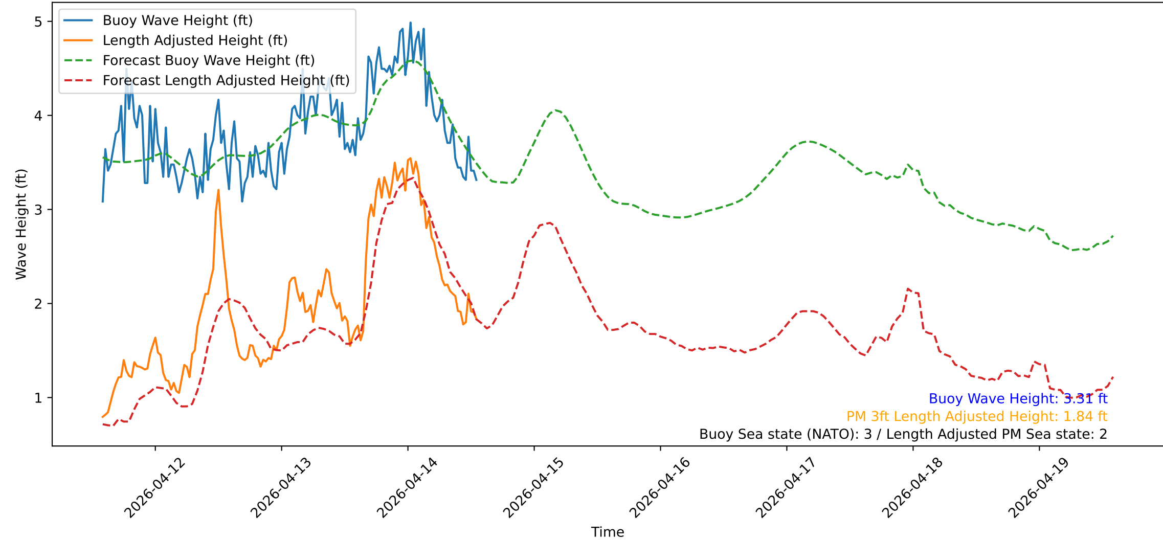
Wave Heights over Time for Green Beach at 2026-04-14 14:01:12
