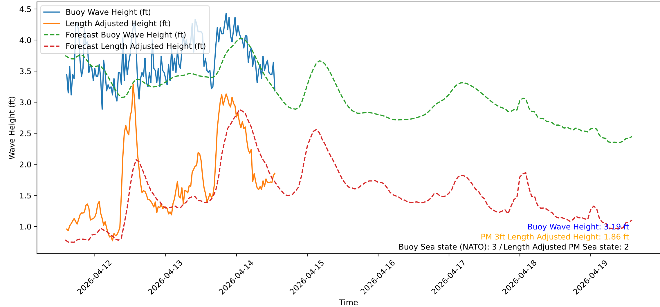
Wave Heights over Time for Red Beach at 2026-04-14 14:00:50
