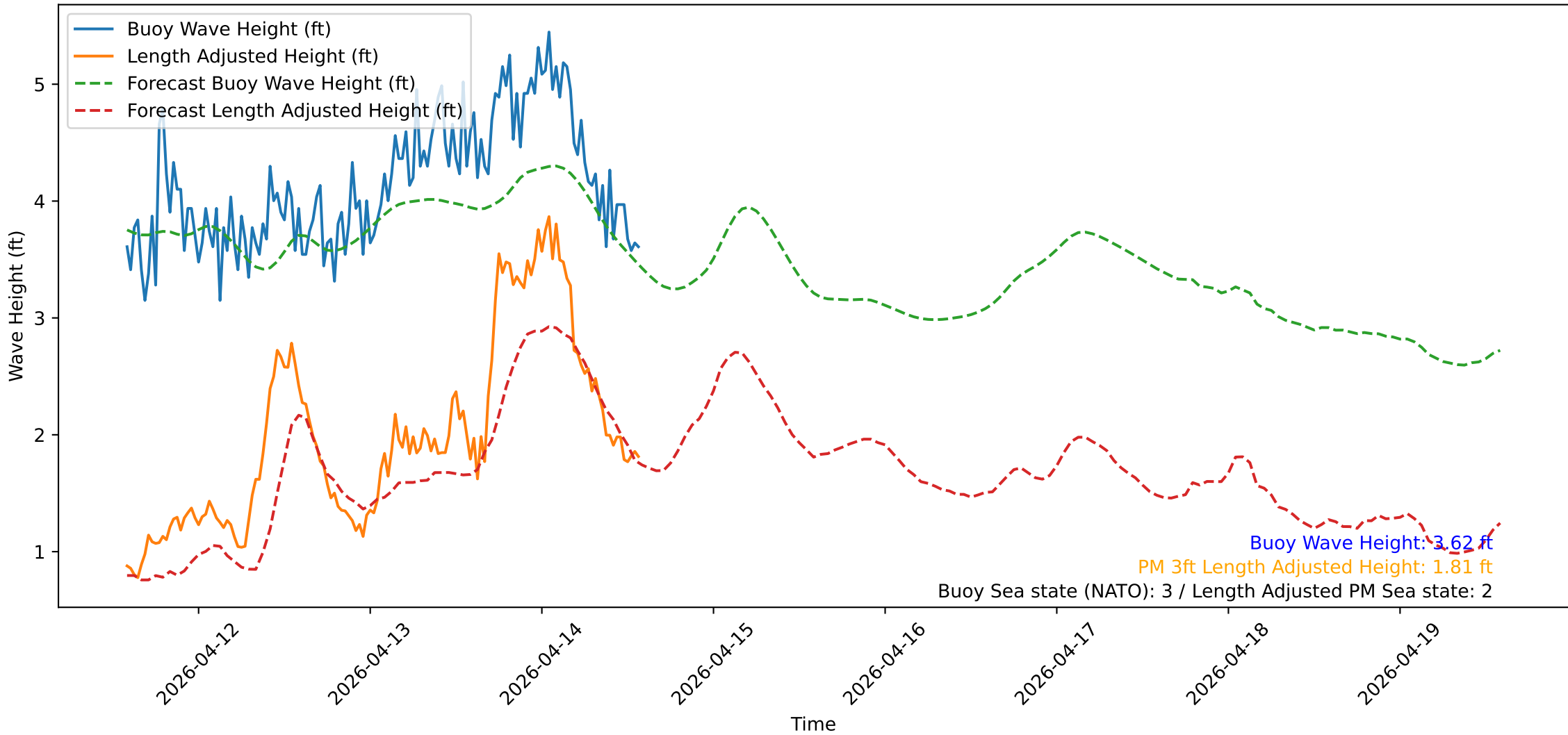
Wave Heights over Time for Oceanside Harbor at 2026-04-14 14:00:31
