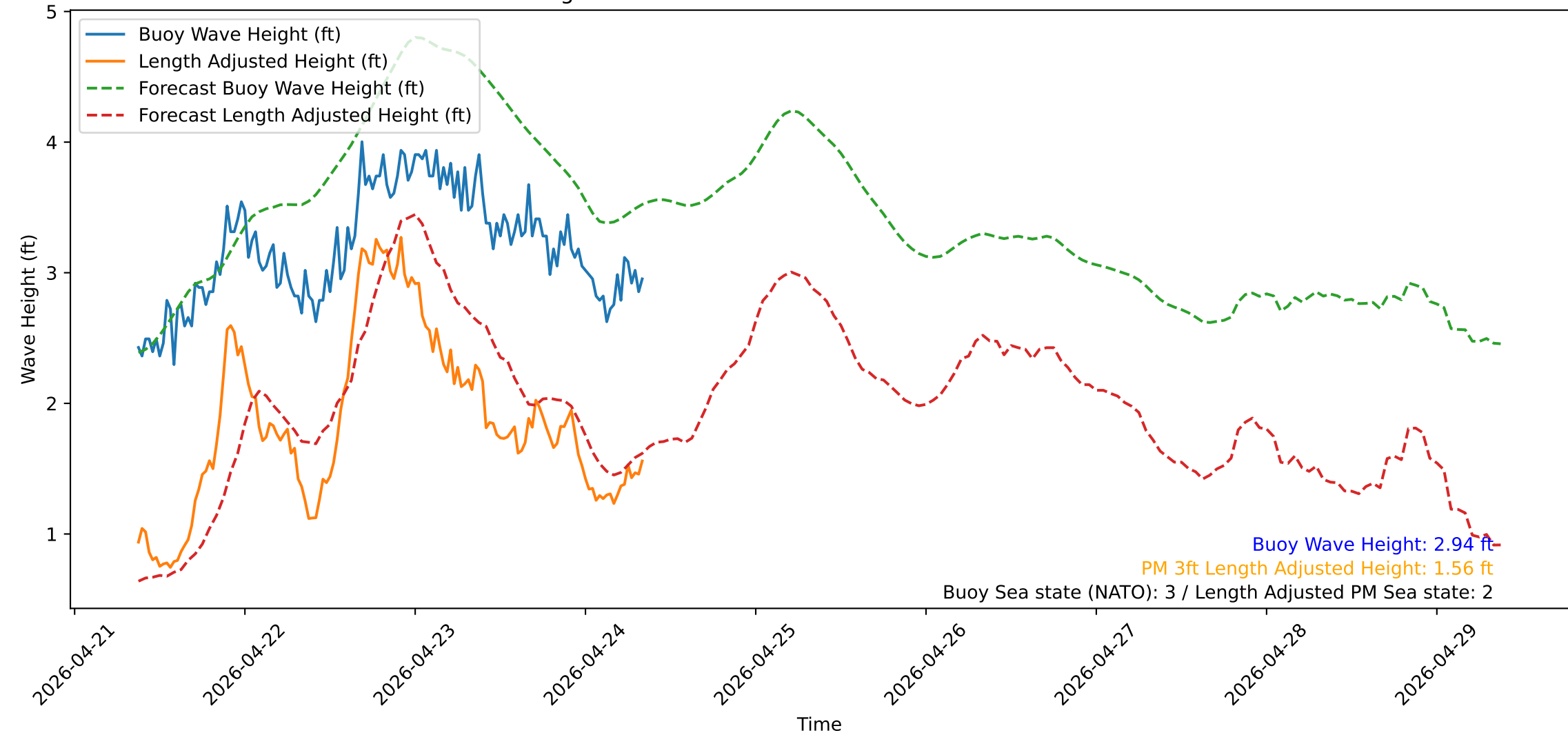
Wave Heights over Time for Green Beach at 2026-04-24 09:01:13
