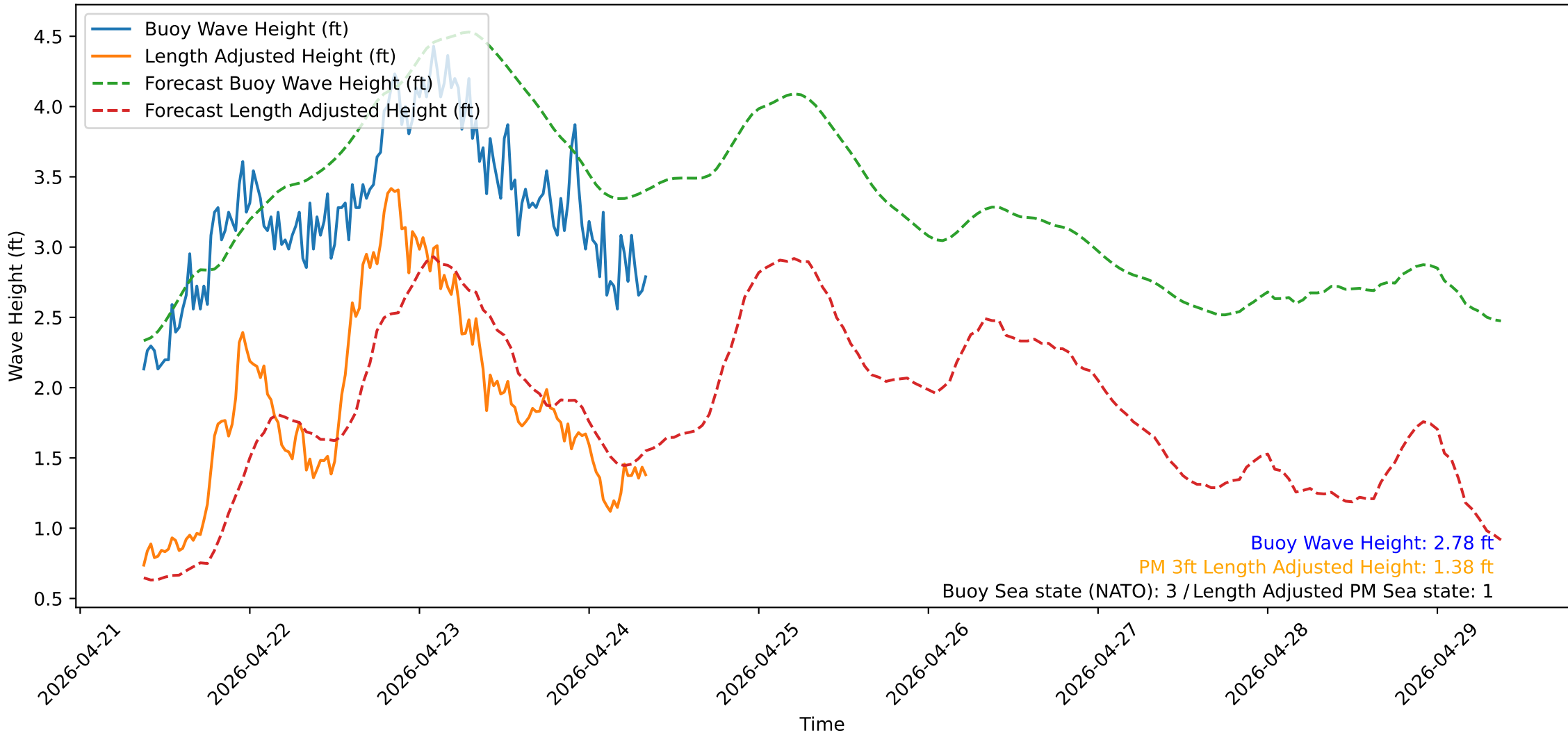
Wave Heights over Time for Oceanside Harbor at 2026-04-24 09:00:32
