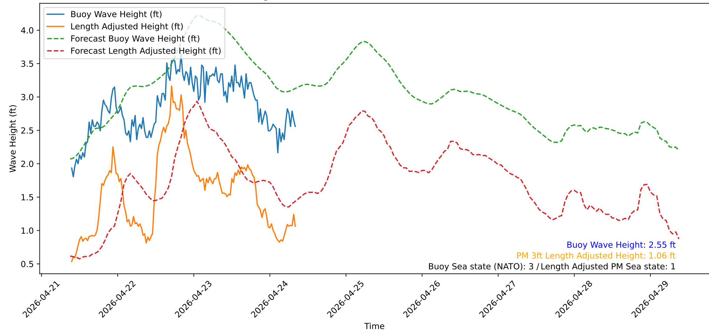
Wave Heights over Time for Red Beach at 2026-04-24 09:00:51
