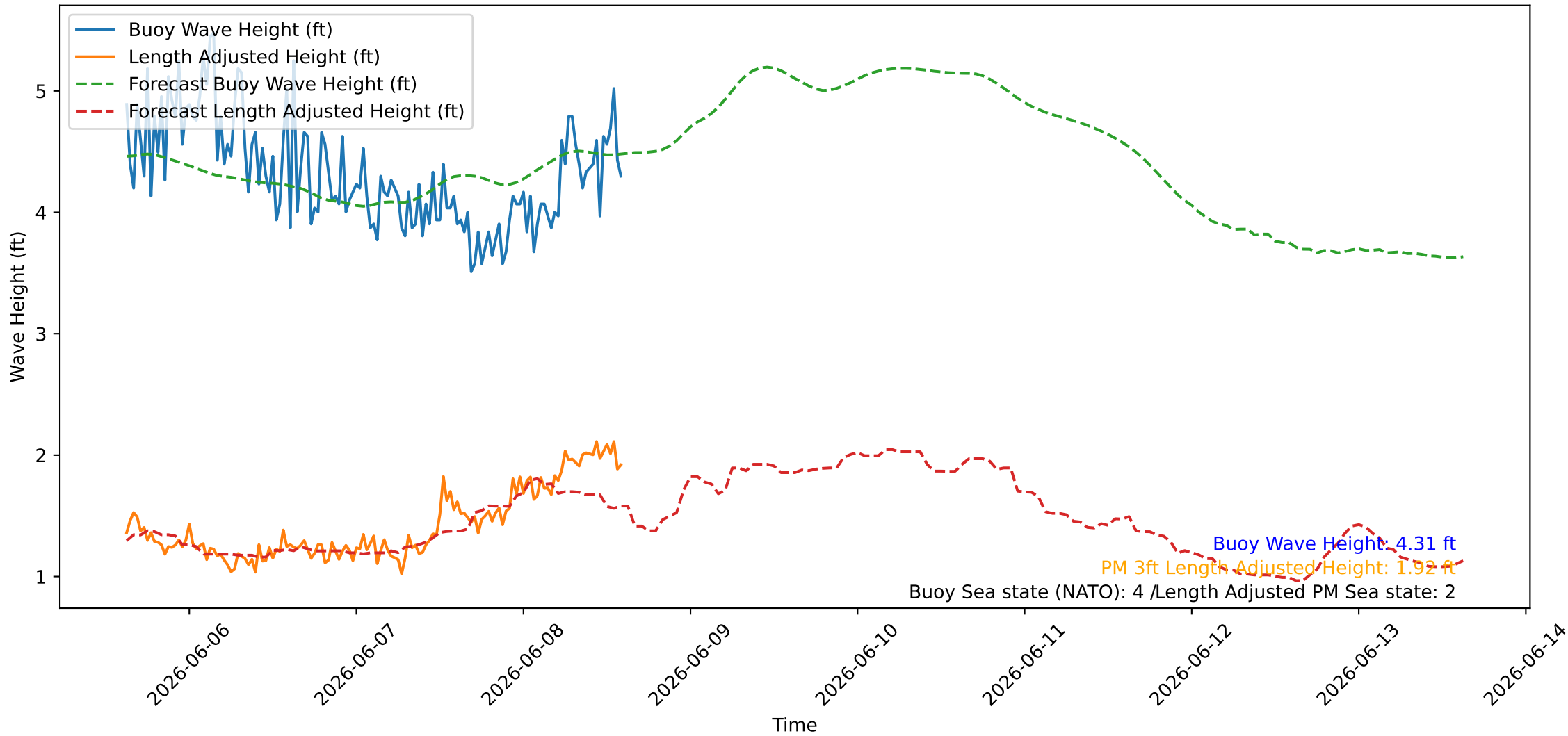
Wave Heights over Time for Oceanside Harbor at 2026-06-08 15:00:26
