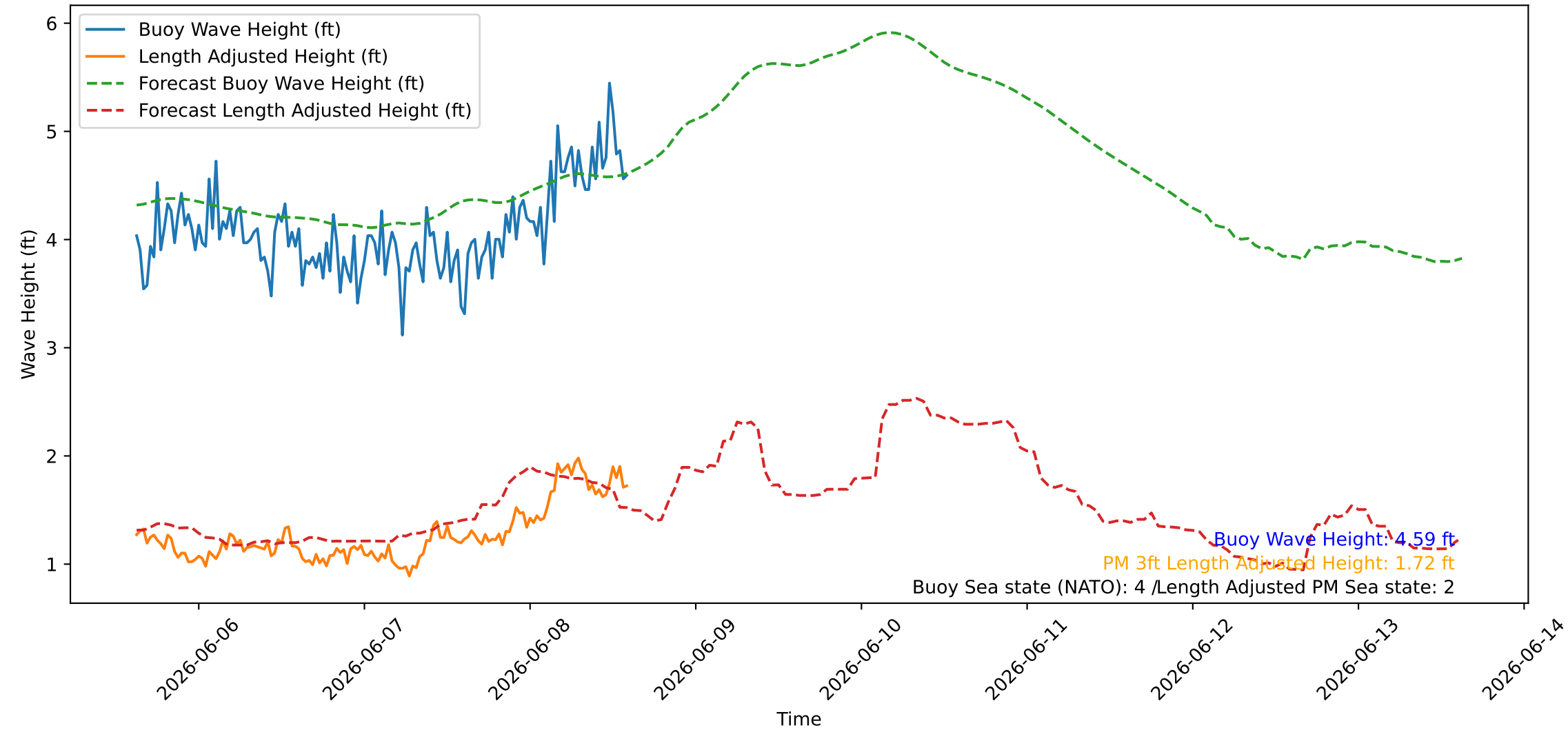
Wave Heights over Time for Green Beach at 2026-06-08 15:01:08
