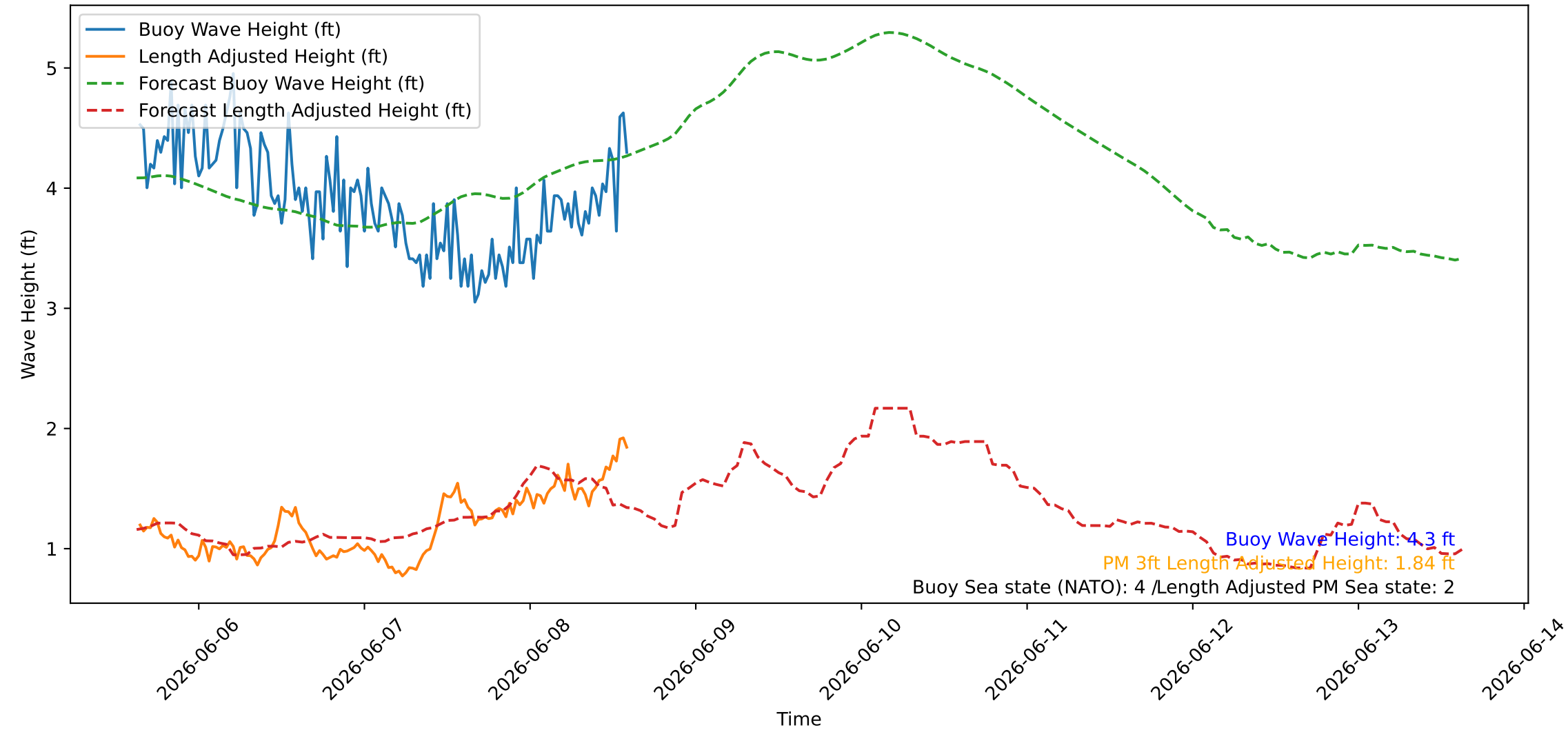
Wave Heights over Time for Red Beach at 2026-06-08 15:00:46
