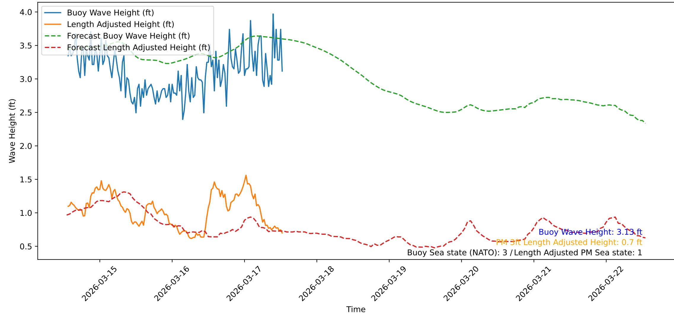
Wave Heights over Time for Oceanside Harbor at 2026-03-17 13:20:43
